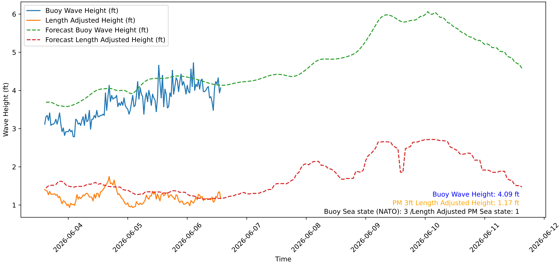
Wave Heights over Time for Green Beach at 2026-06-06 14:31:09
