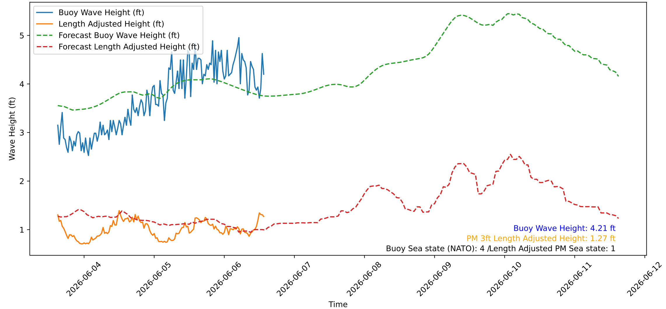
Wave Heights over Time for Red Beach at 2026-06-06 14:30:46
