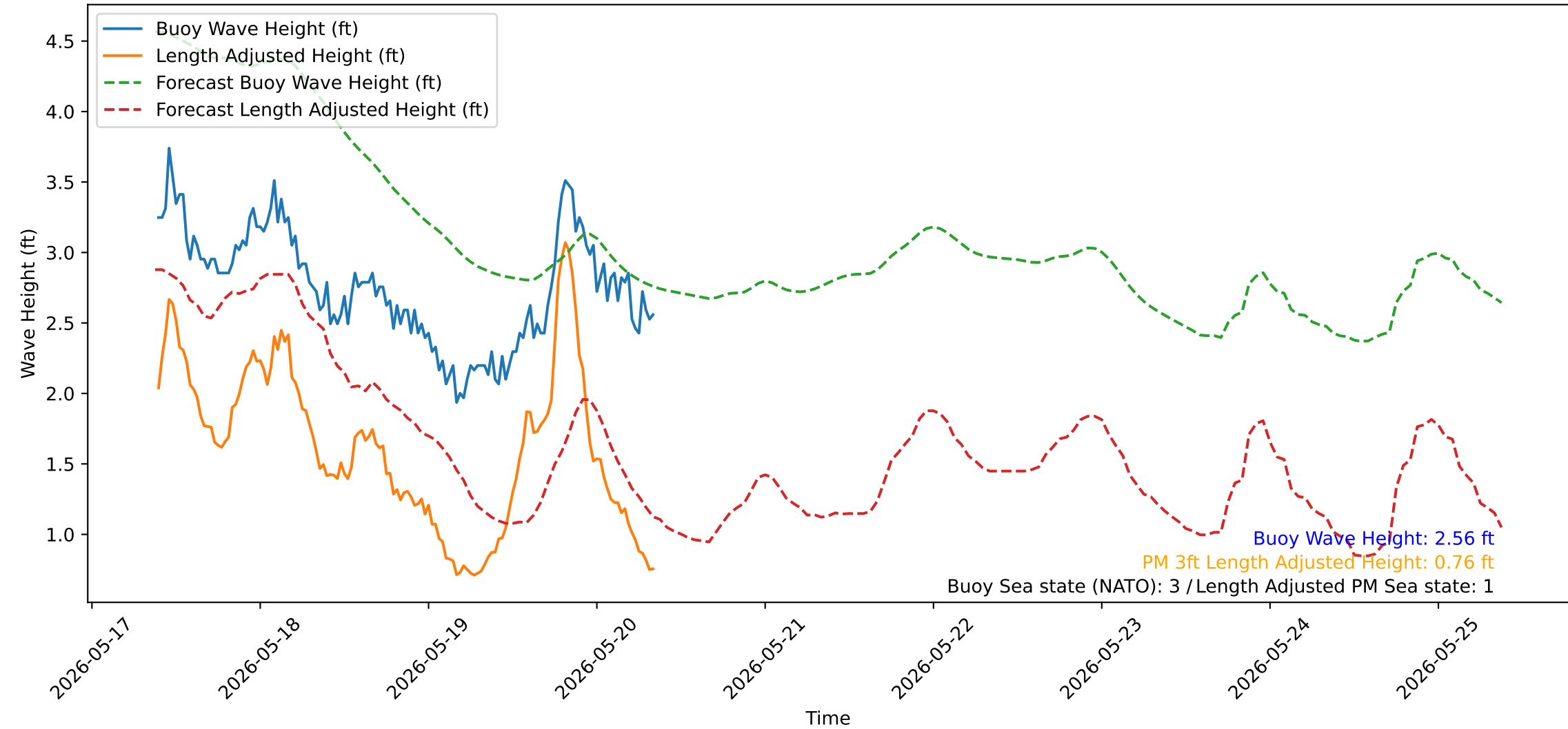
Wave Heights over Time for Red Beach at 2026-05-20 09:00:51
