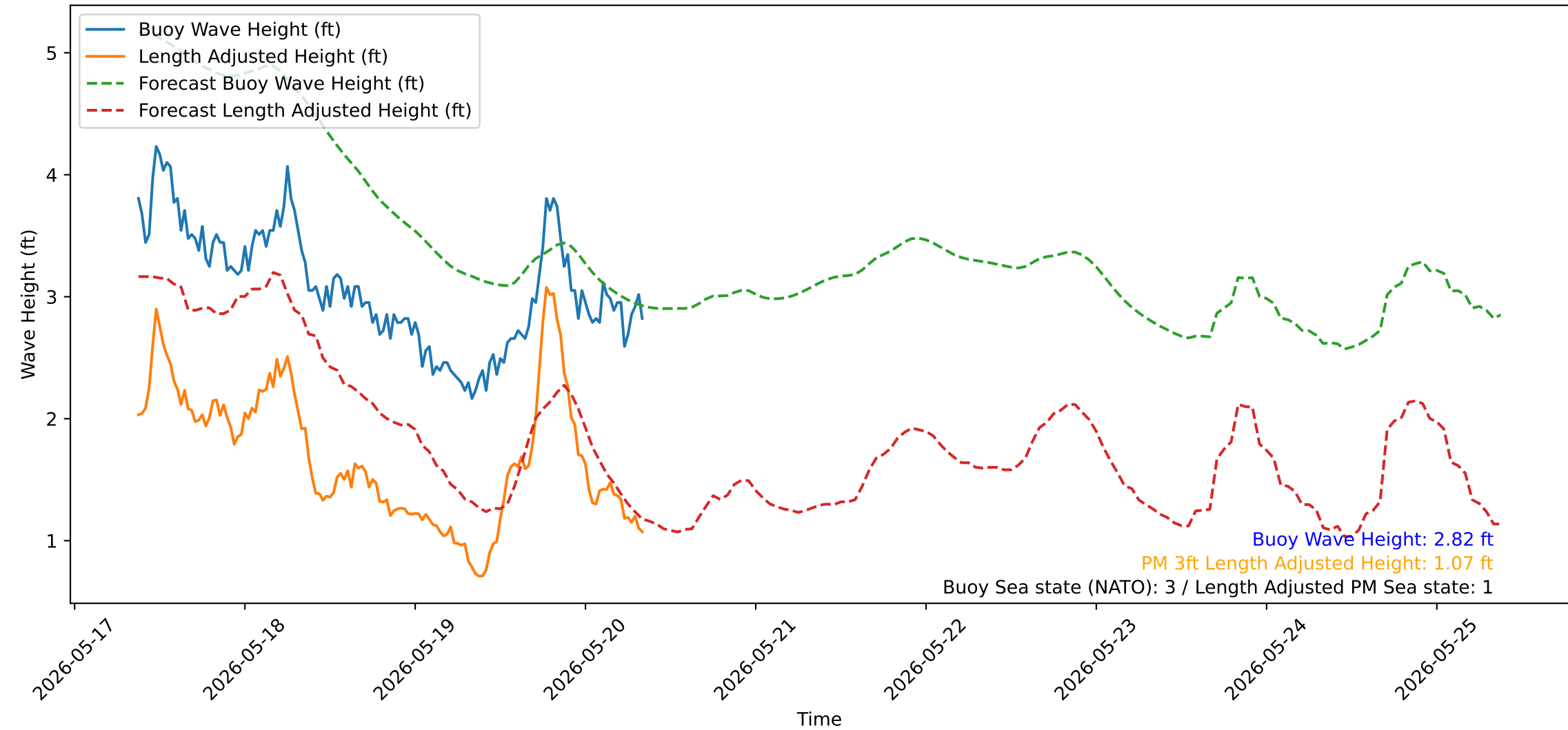
Wave Heights over Time for Green Beach at 2026-05-20 09:01:14
