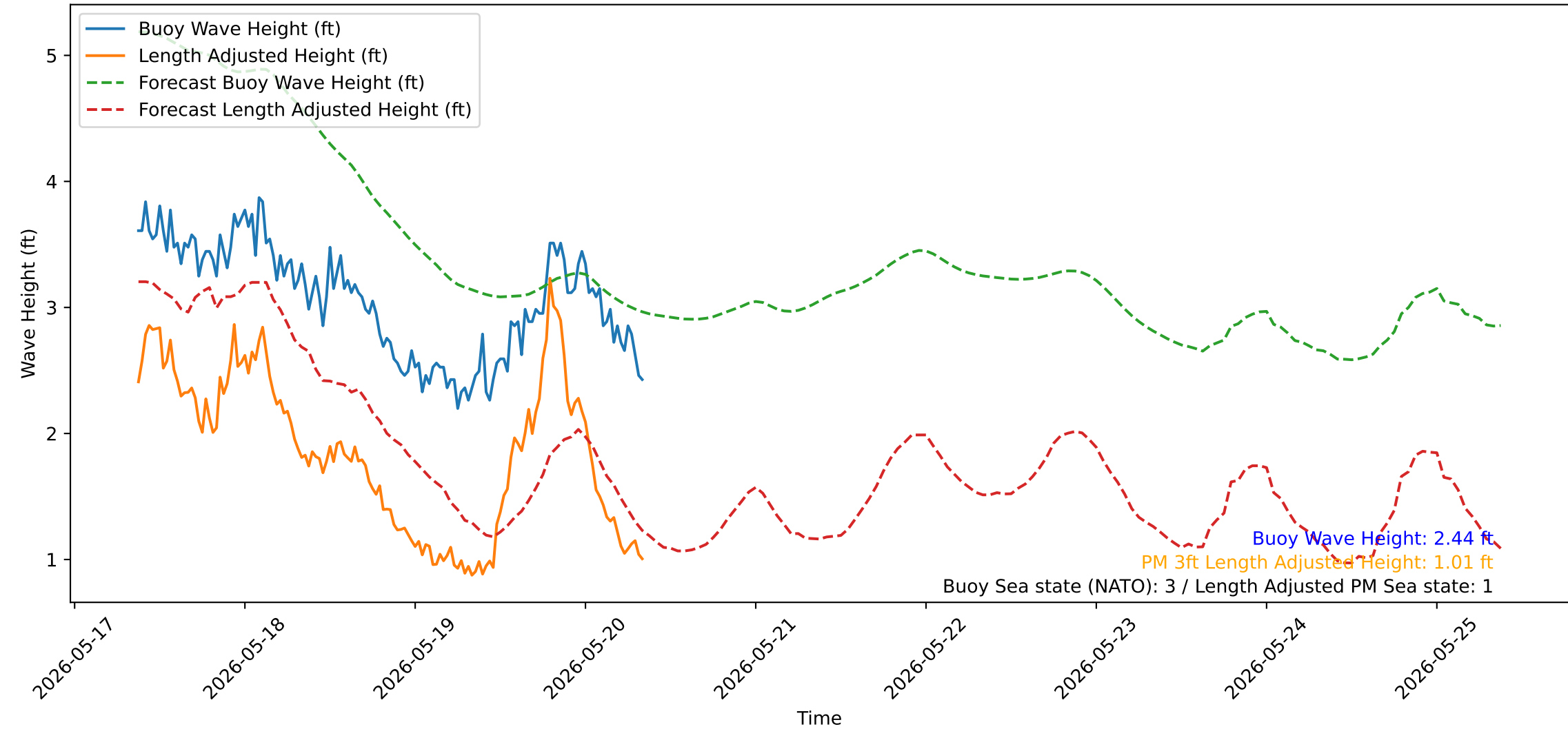
Wave Heights over Time for Oceanside Harbor at 2026-05-20 09:00:32
