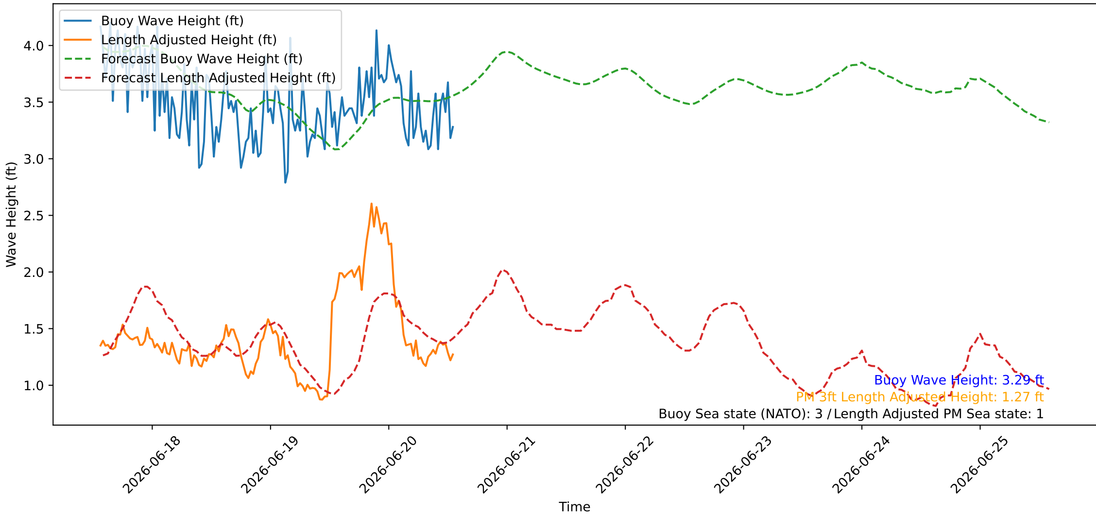
Wave Heights over Time for Oceanside Harbor at 2026-06-20 13:40:26
