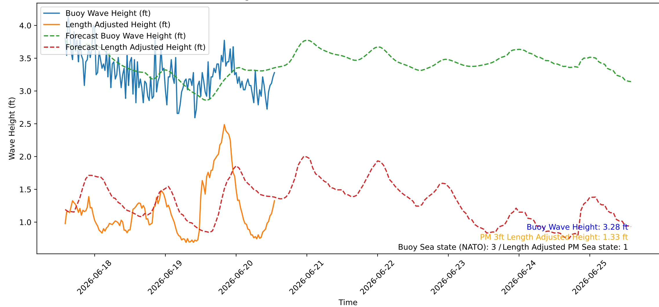
Wave Heights over Time for Red Beach at 2026-06-20 13:40:45
