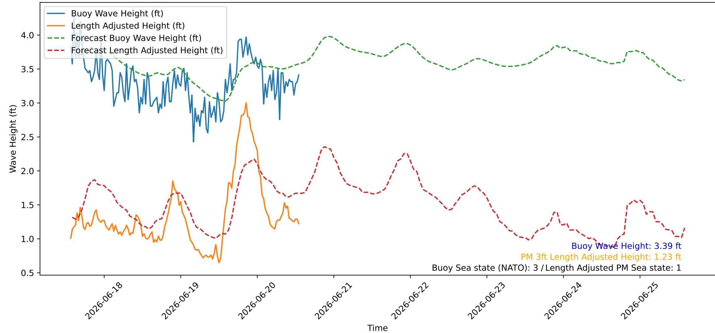
Wave Heights over Time for Green Beach at 2026-06-20 13:41:07
