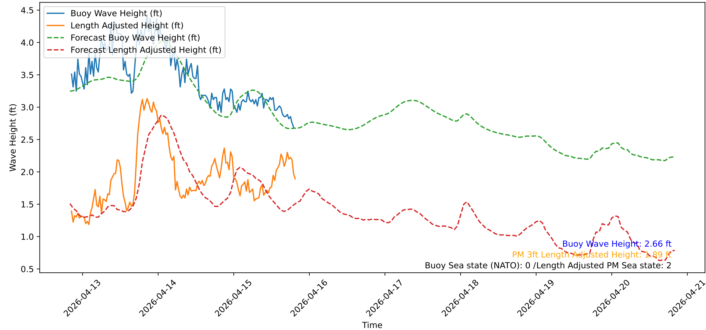
Wave Heights over Time for Red Beach at 2026-04-15 20:20:51
