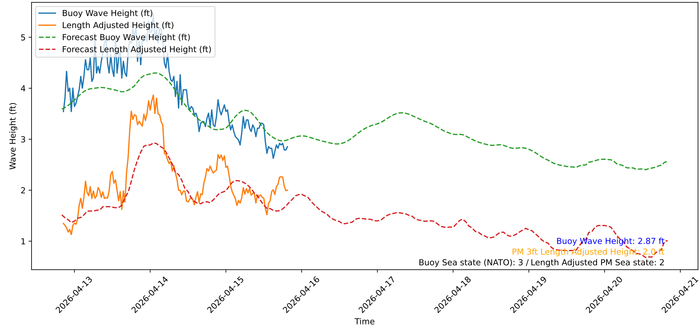
Wave Heights over Time for Oceanside Harbor at 2026-04-15 20:20:31
