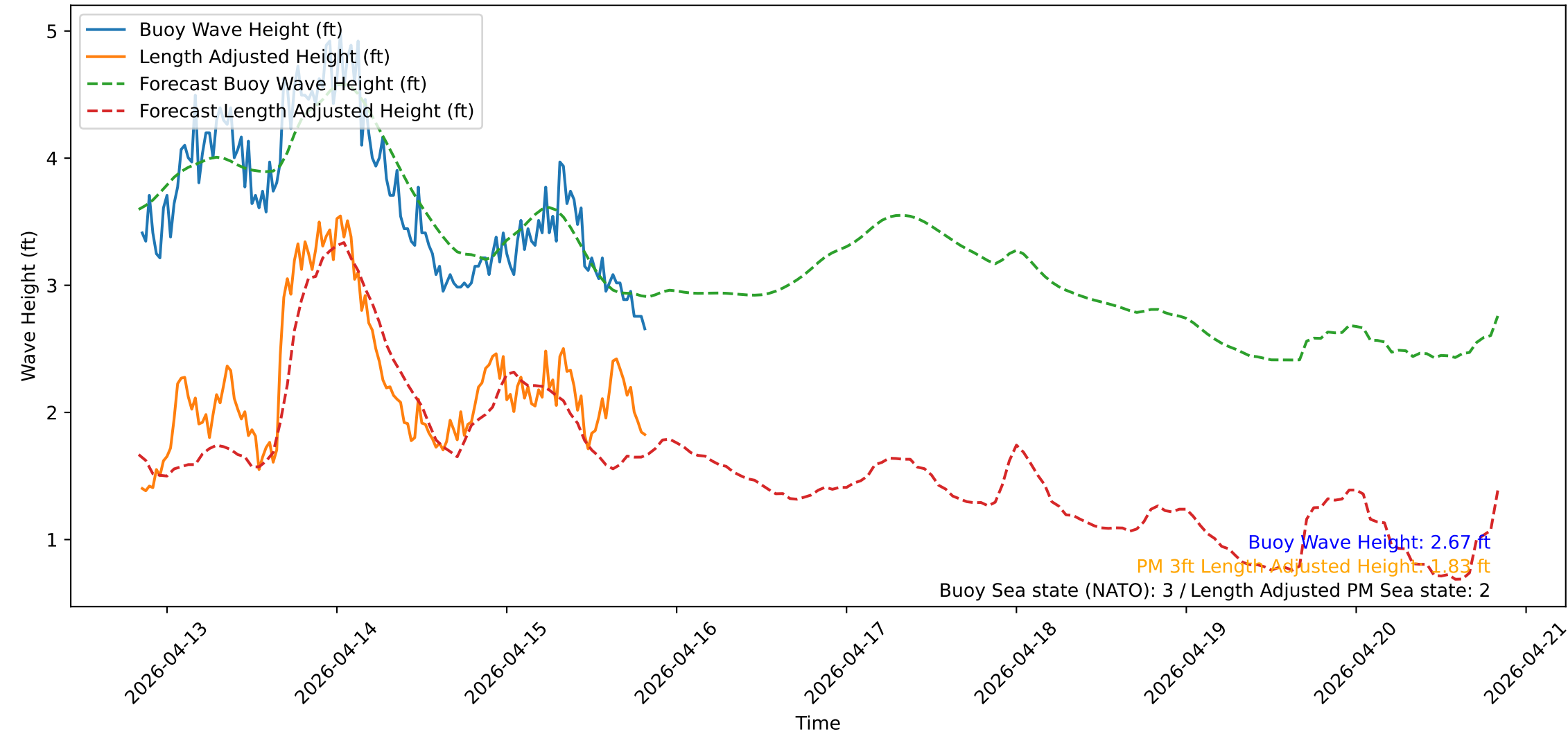
Wave Heights over Time for Green Beach at 2026-04-15 20:21:14
