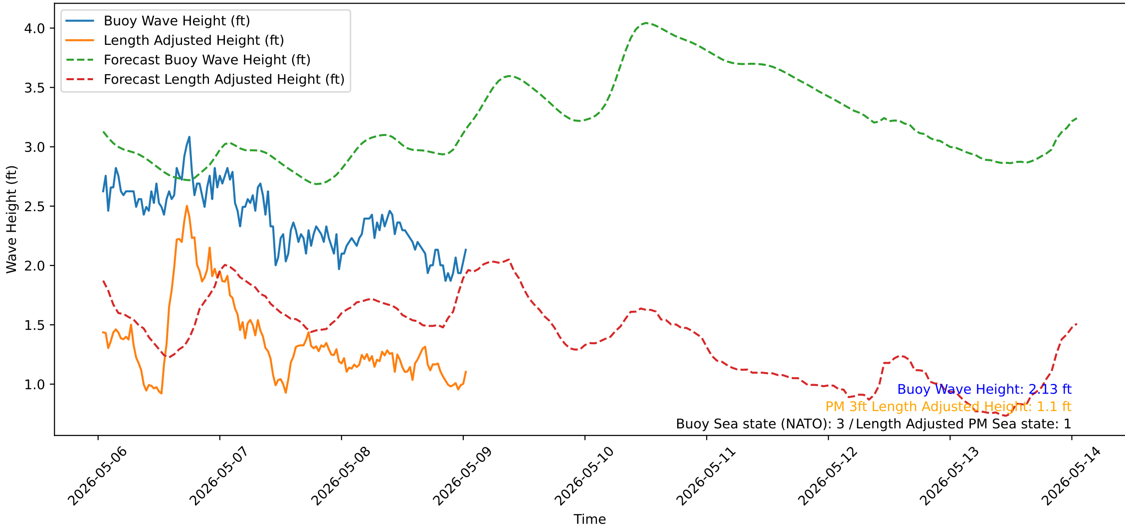
Wave Heights over Time for Oceanside Harbor at 2026-05-09 01:00:32
