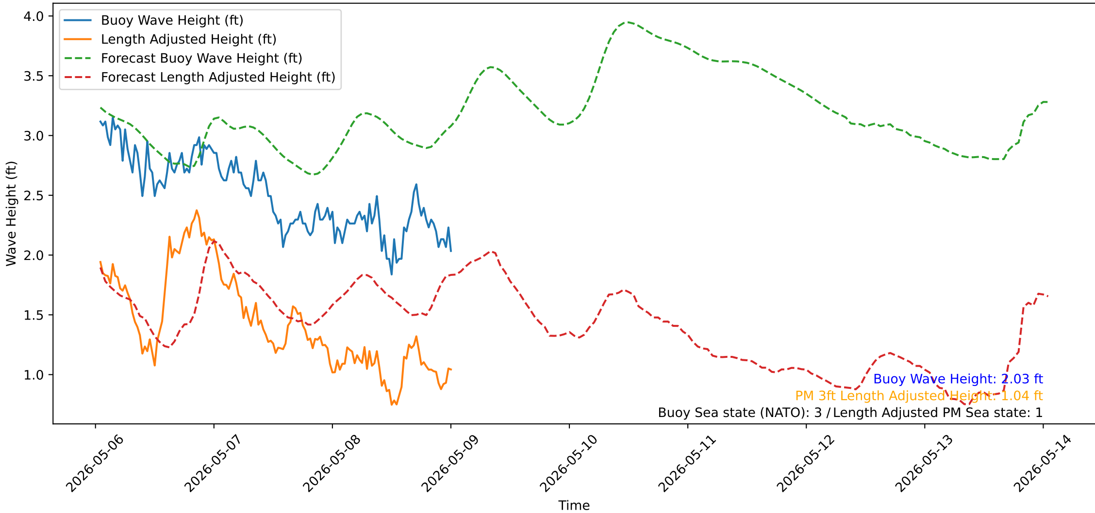
Wave Heights over Time for Green Beach at 2026-05-09 01:01:13
