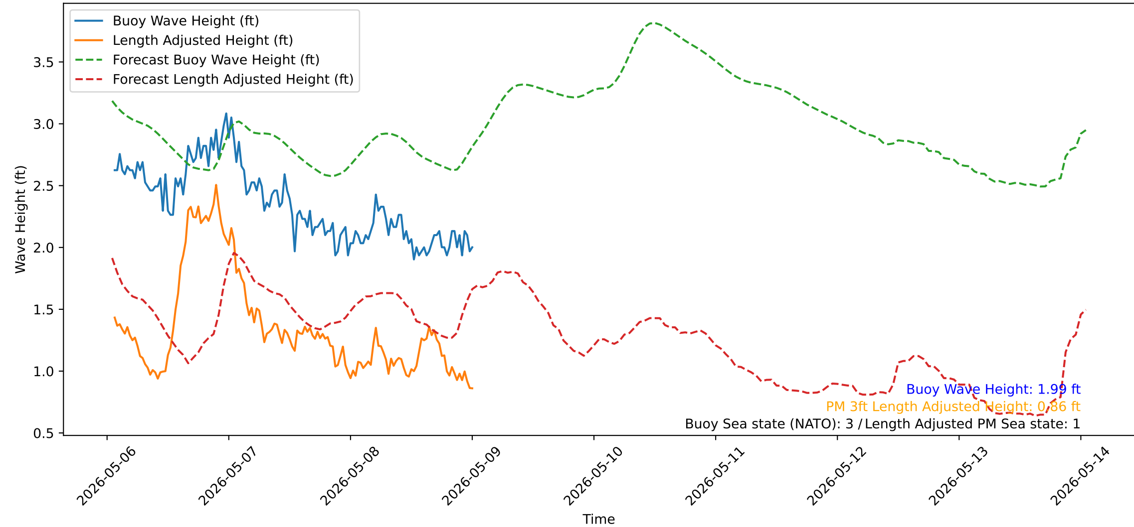
Wave Heights over Time for Red Beach at 2026-05-09 01:00:51
