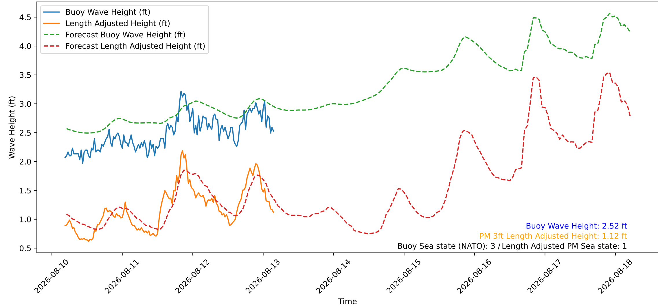
Wave Heights over Time for Green Beach at 2026-08-13 04:31:08
