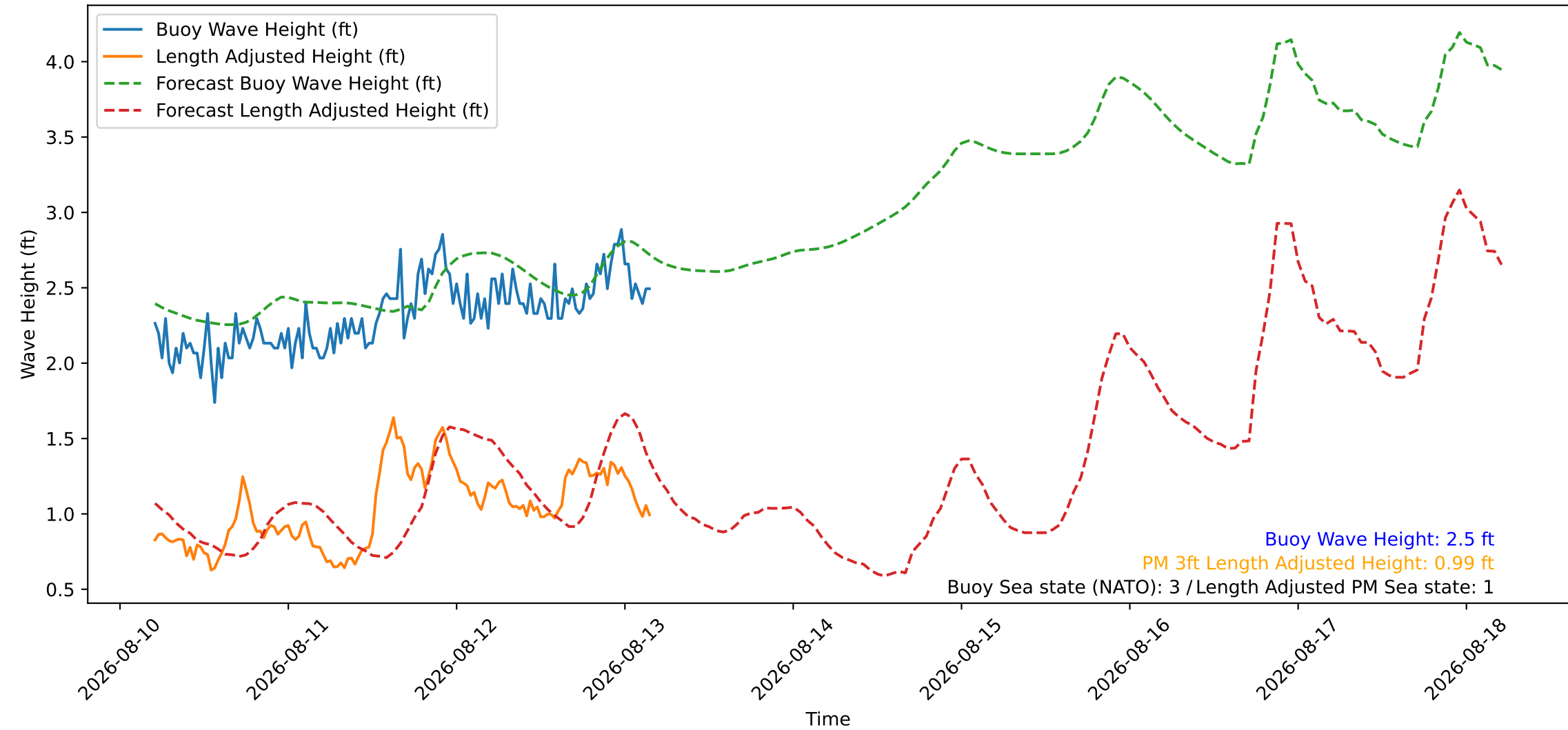
Wave Heights over Time for Red Beach at 2026-08-13 04:30:46
