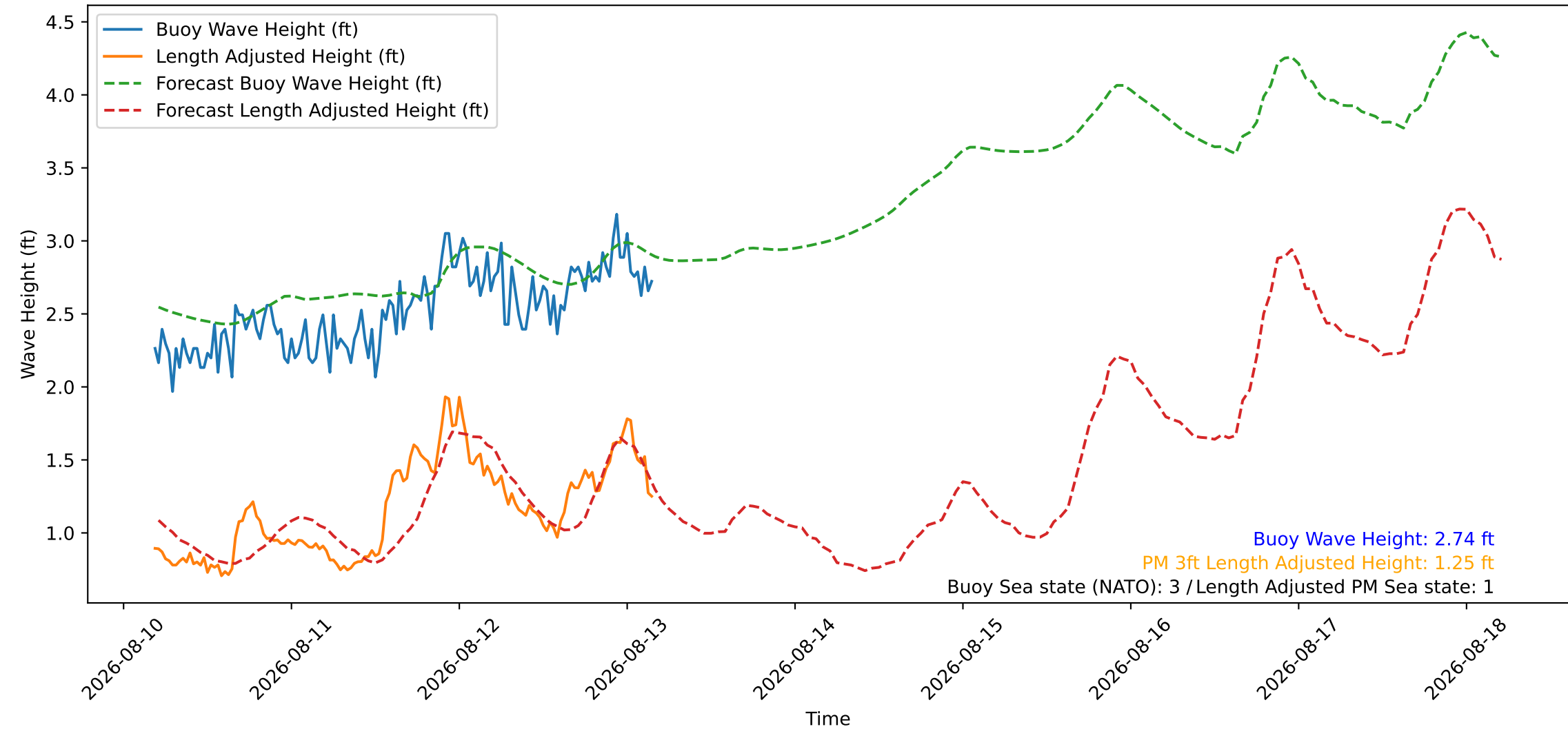
Wave Heights over Time for Oceanside Harbor at 2026-08-13 04:30:26
