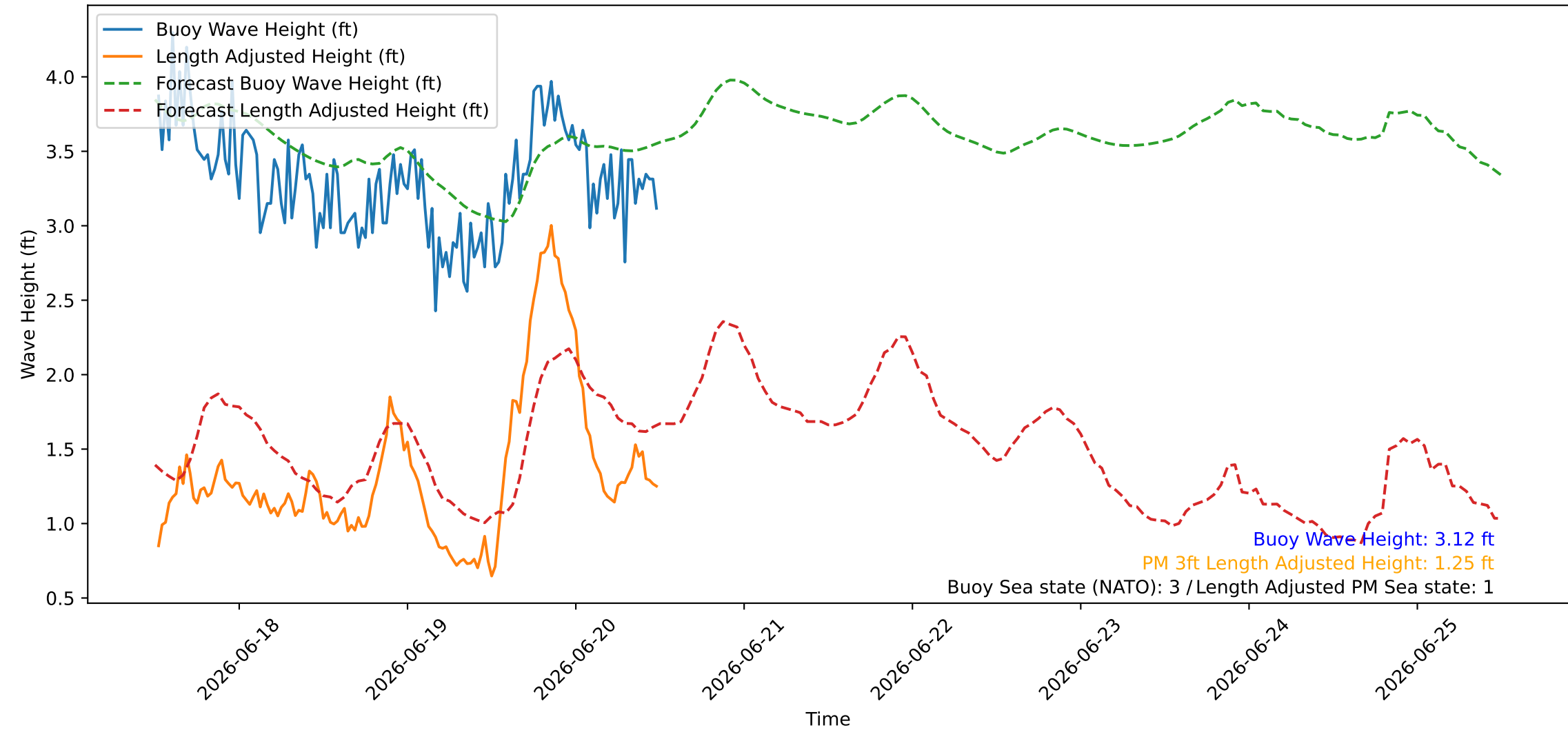
Wave Heights over Time for Green Beach at 2026-06-20 12:21:08
