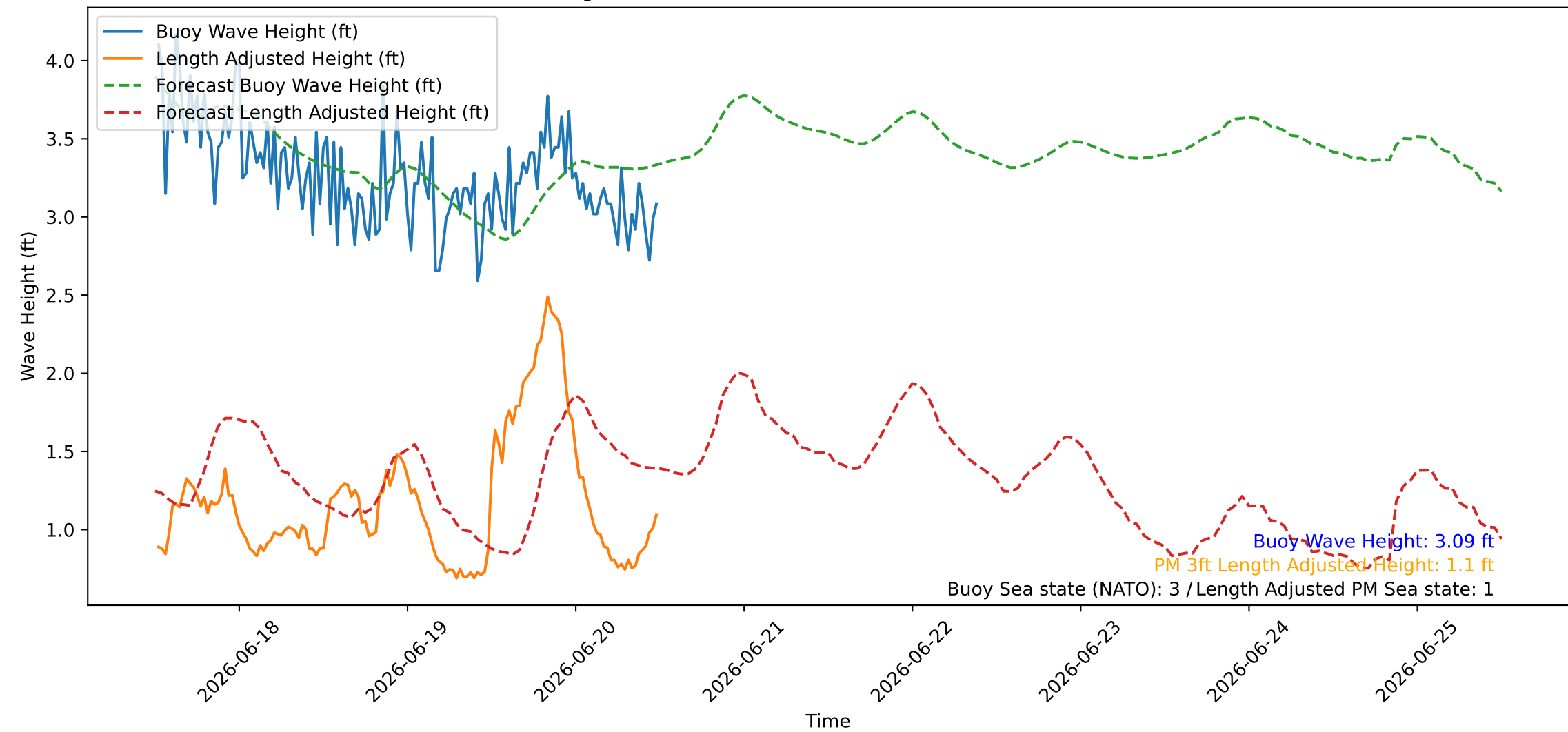
Wave Heights over Time for Red Beach at 2026-06-20 12:20:46
