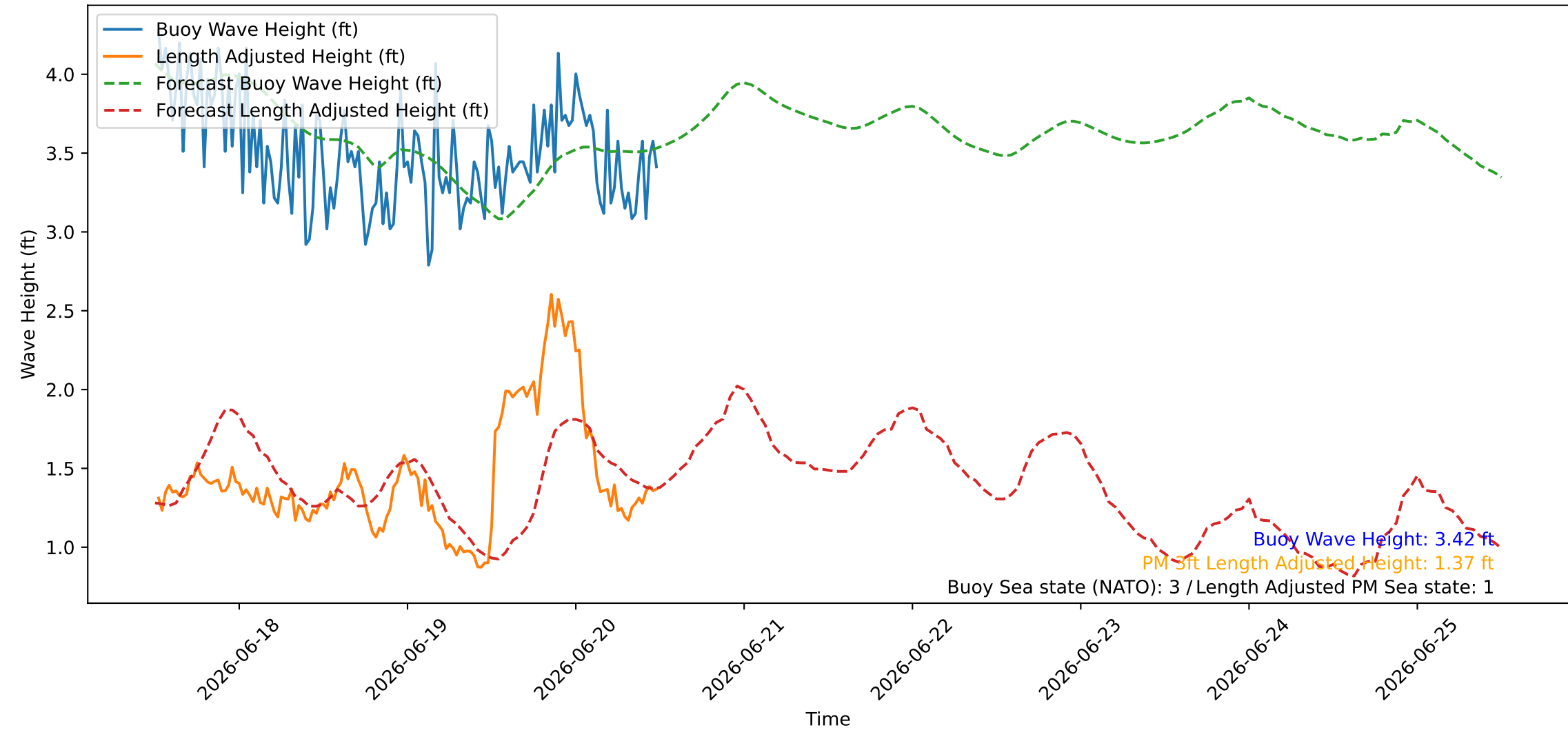
Wave Heights over Time for Oceanside Harbor at 2026-06-20 12:20:26
