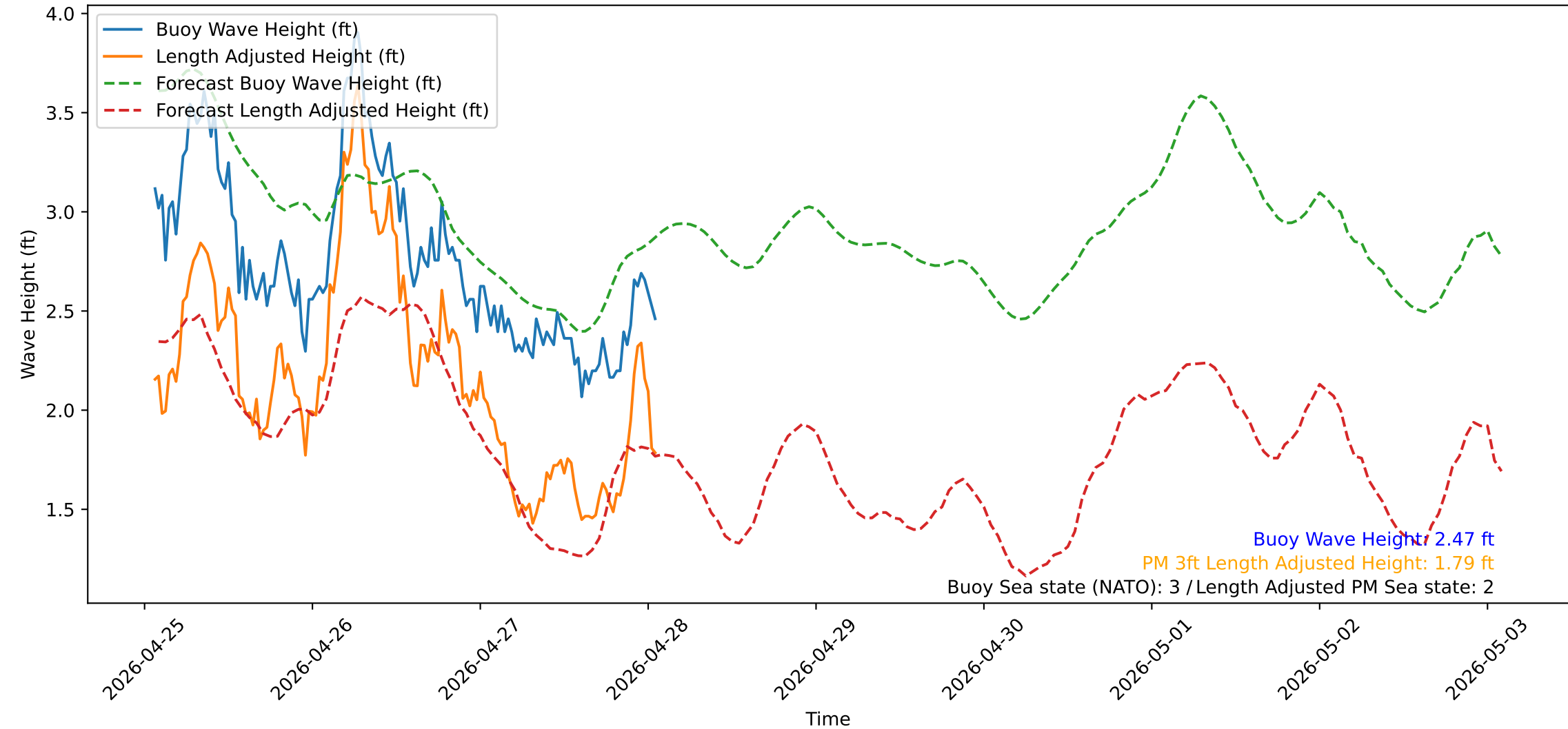
Wave Heights over Time for Oceanside Harbor at 2026-04-28 01:40:31
