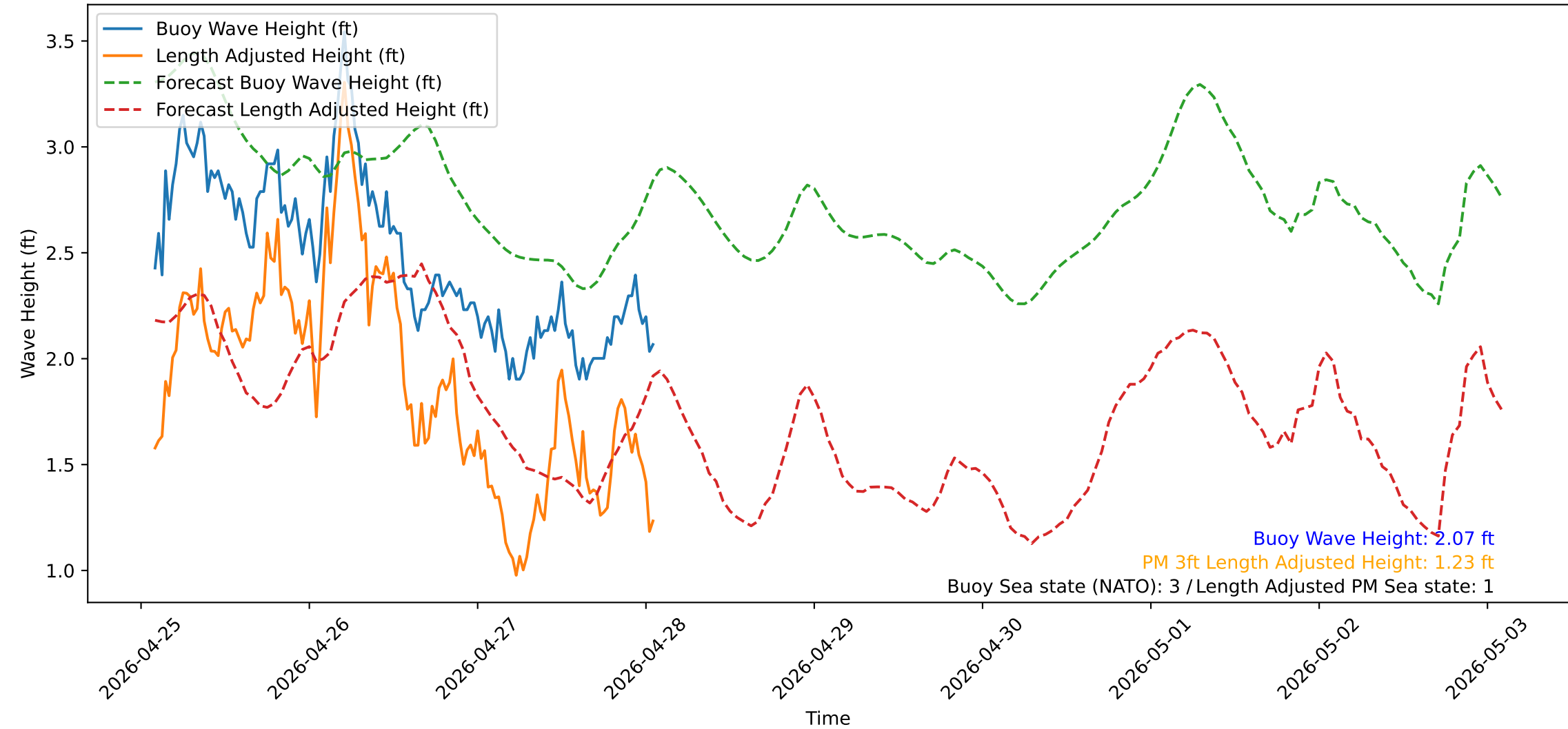
Wave Heights over Time for Red Beach at 2026-04-28 01:40:51
