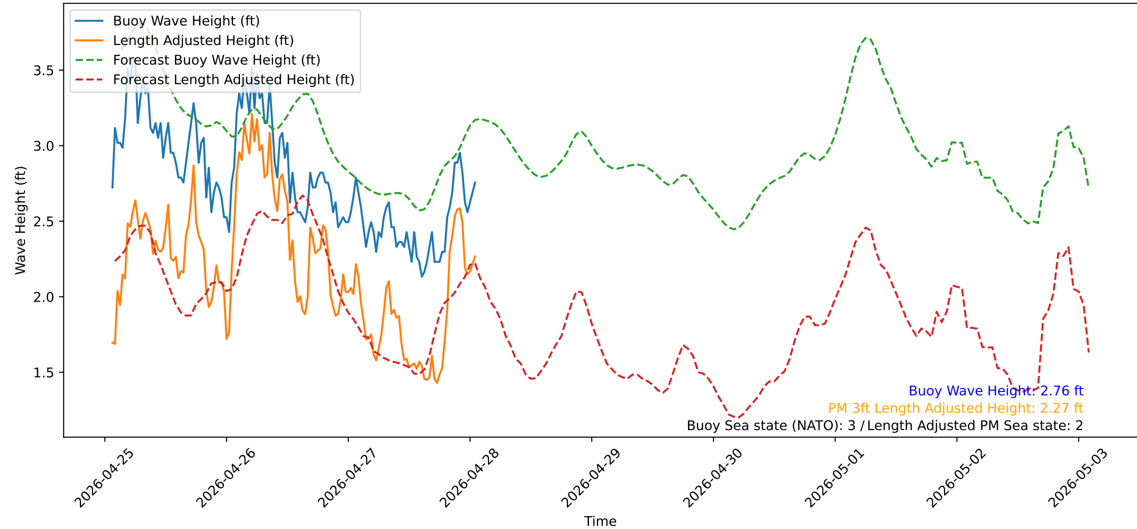
Wave Heights over Time for Green Beach at 2026-04-28 01:41:13
