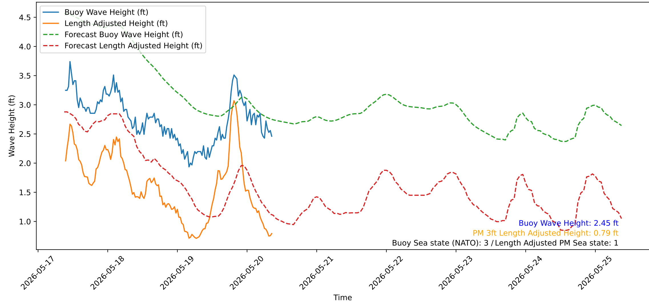
Wave Heights over Time for Red Beach at 2026-05-20 09:10:51
