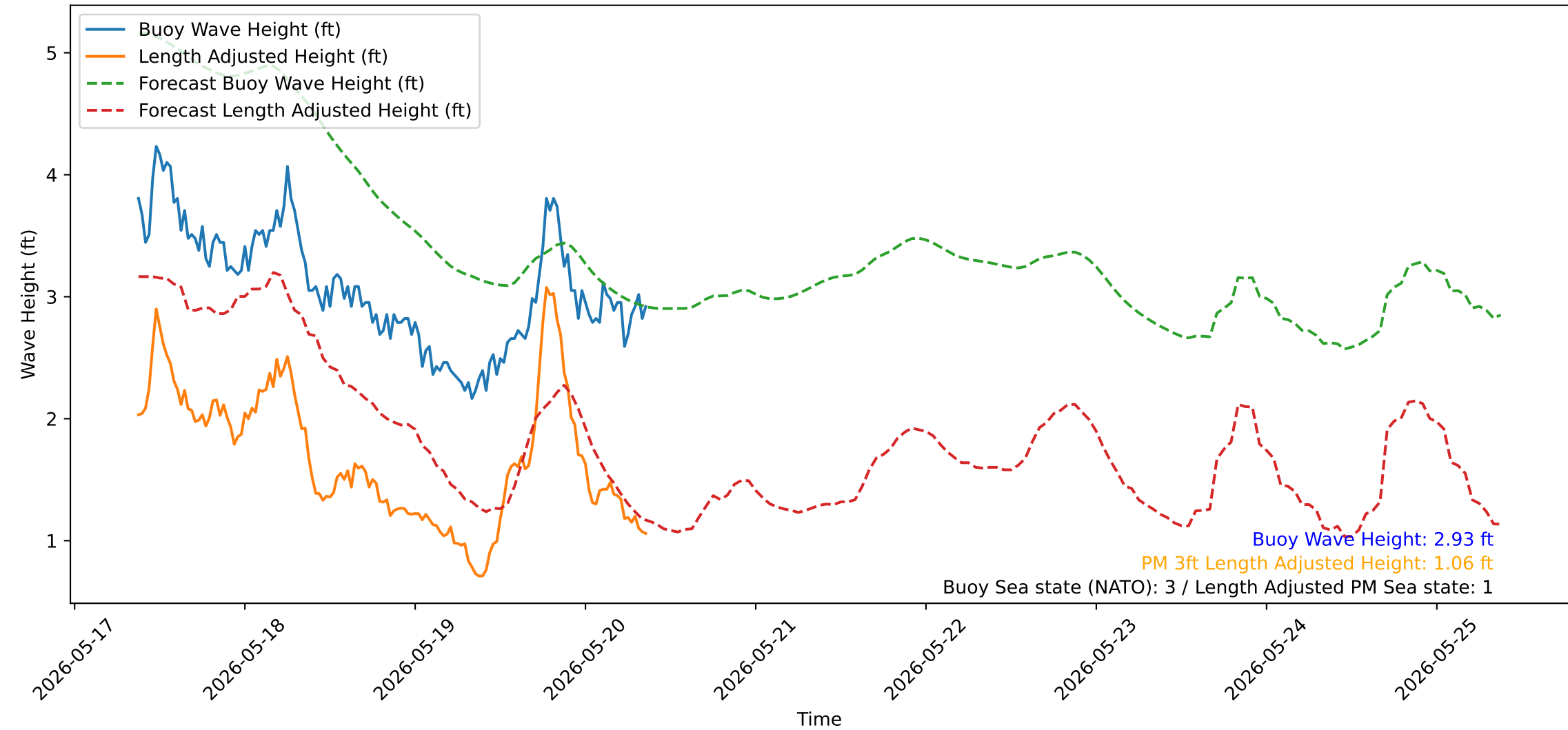
Wave Heights over Time for Green Beach at 2026-05-20 09:11:13
