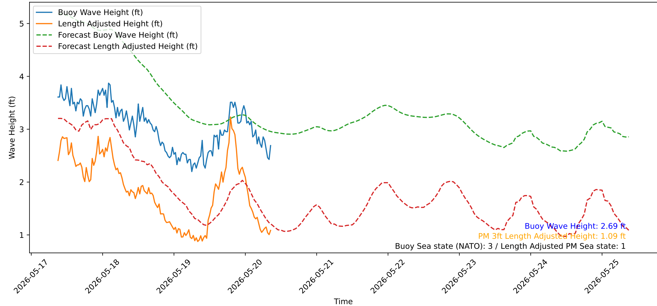
Wave Heights over Time for Oceanside Harbor at 2026-05-20 09:10:31
