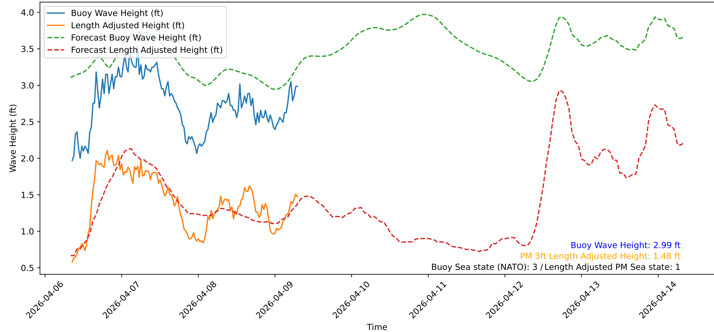
Wave Heights over Time for Red Beach at 2026-04-09 08:00:47
