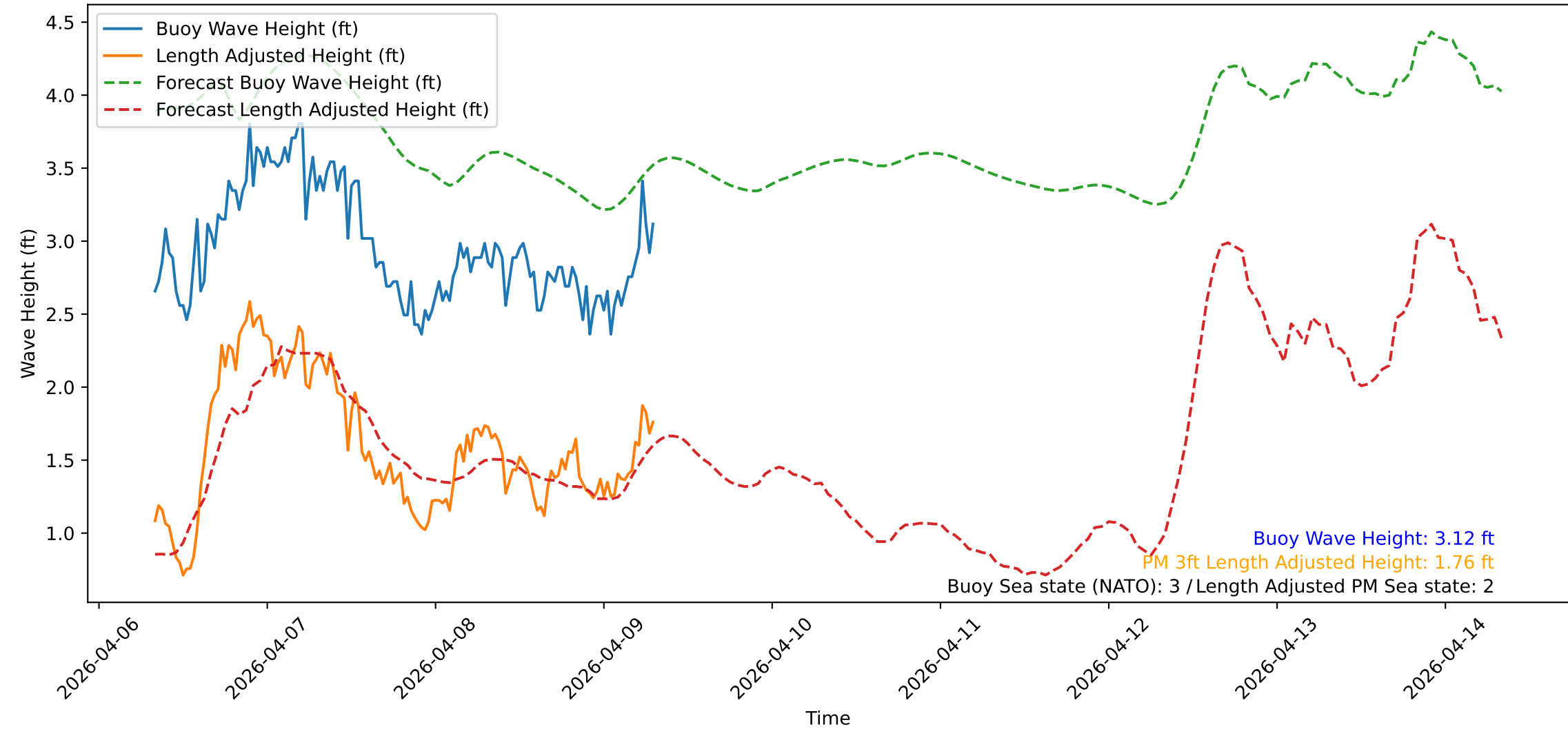
Wave Heights over Time for Green Beach at 2026-04-09 08:01:10
