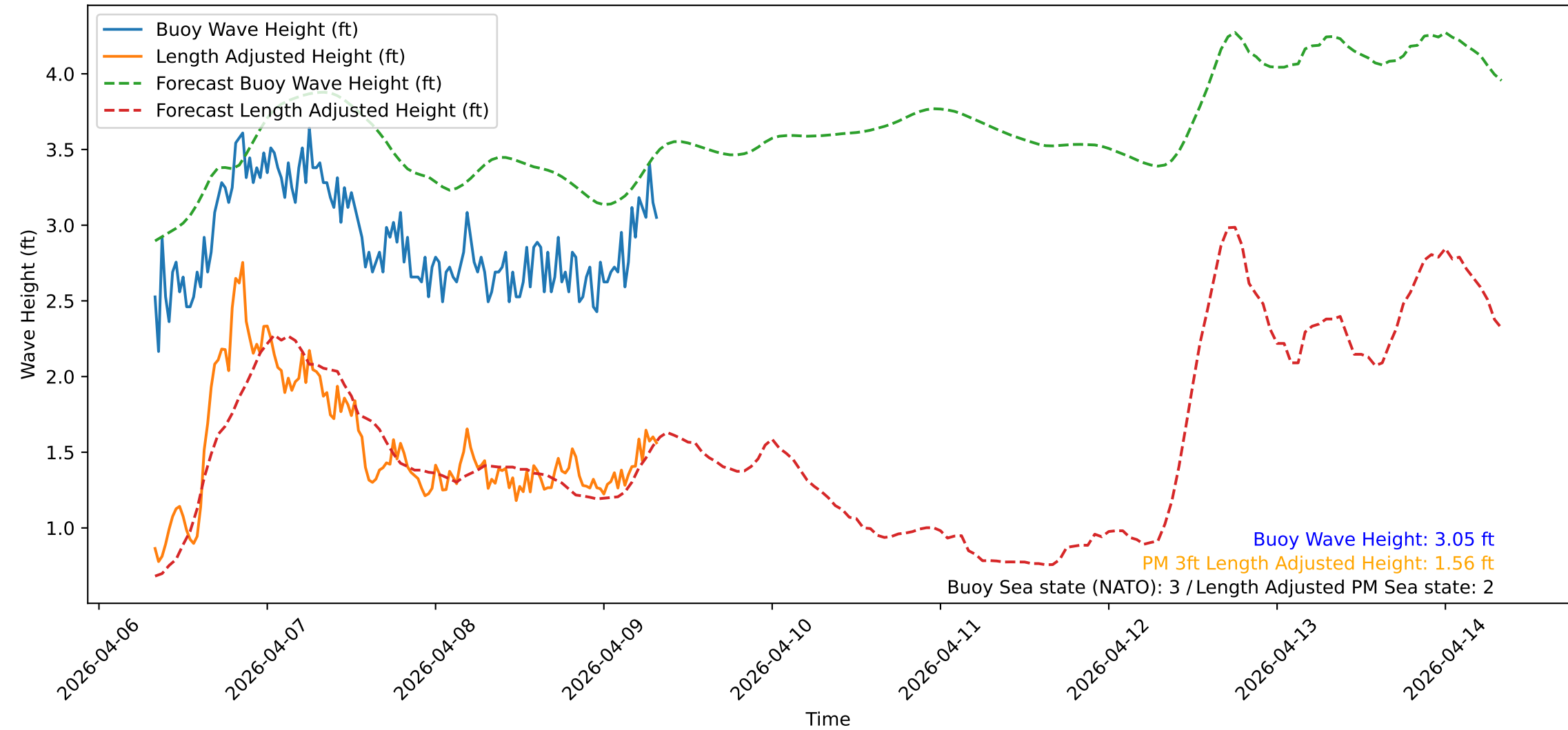
Wave Heights over Time for Oceanside Harbor at 2026-04-09 08:00:31
