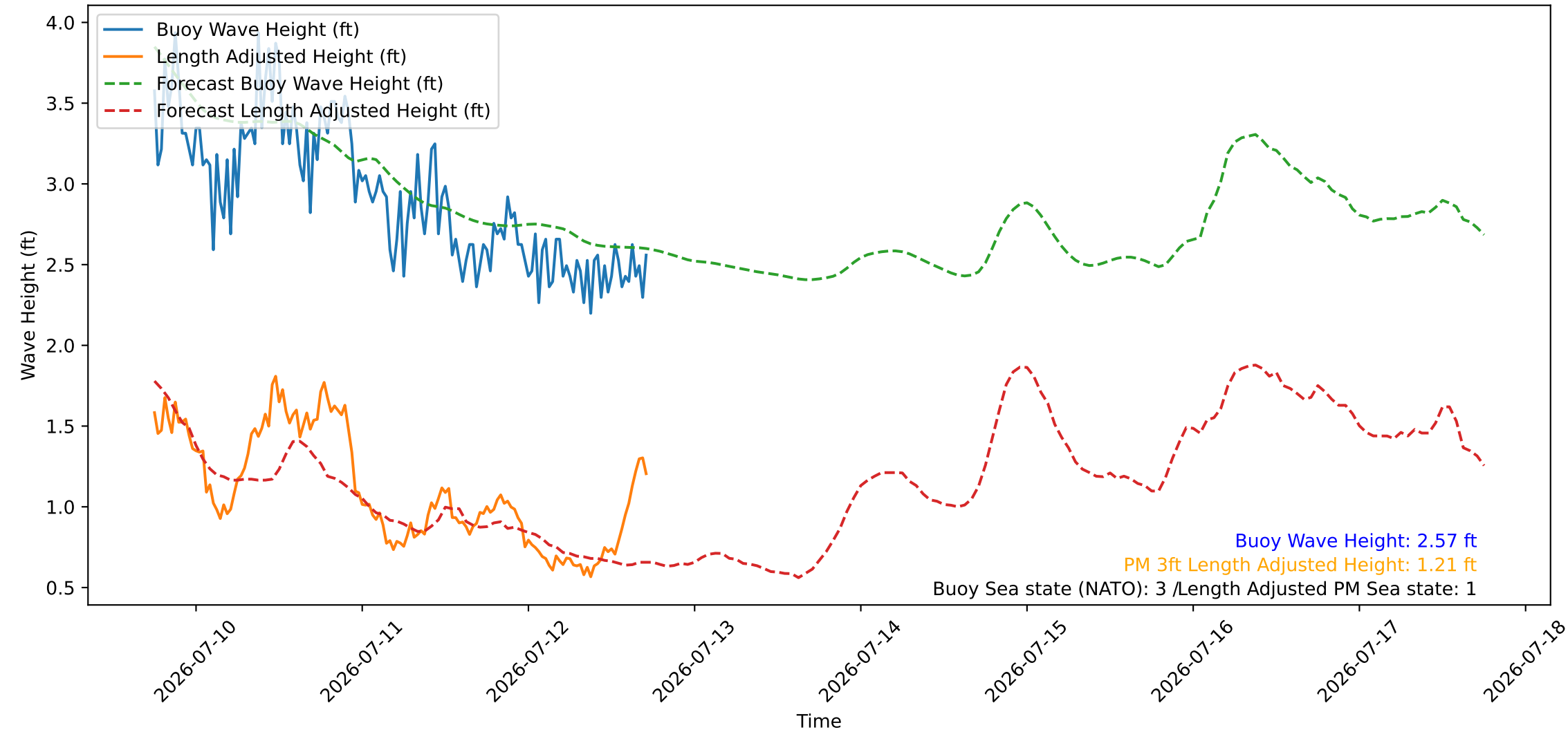
Wave Heights over Time for Red Beach at 2026-07-12 17:40:46
