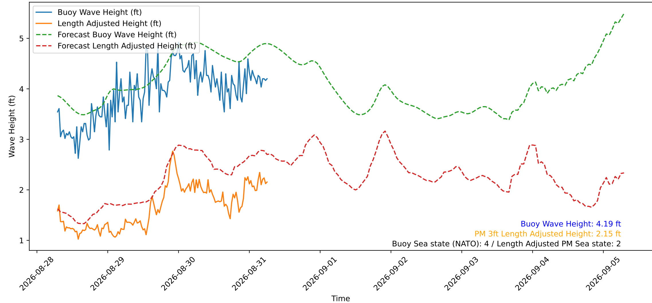
Wave Heights over Time for Green Beach at 2026-08-31 06:51:15
