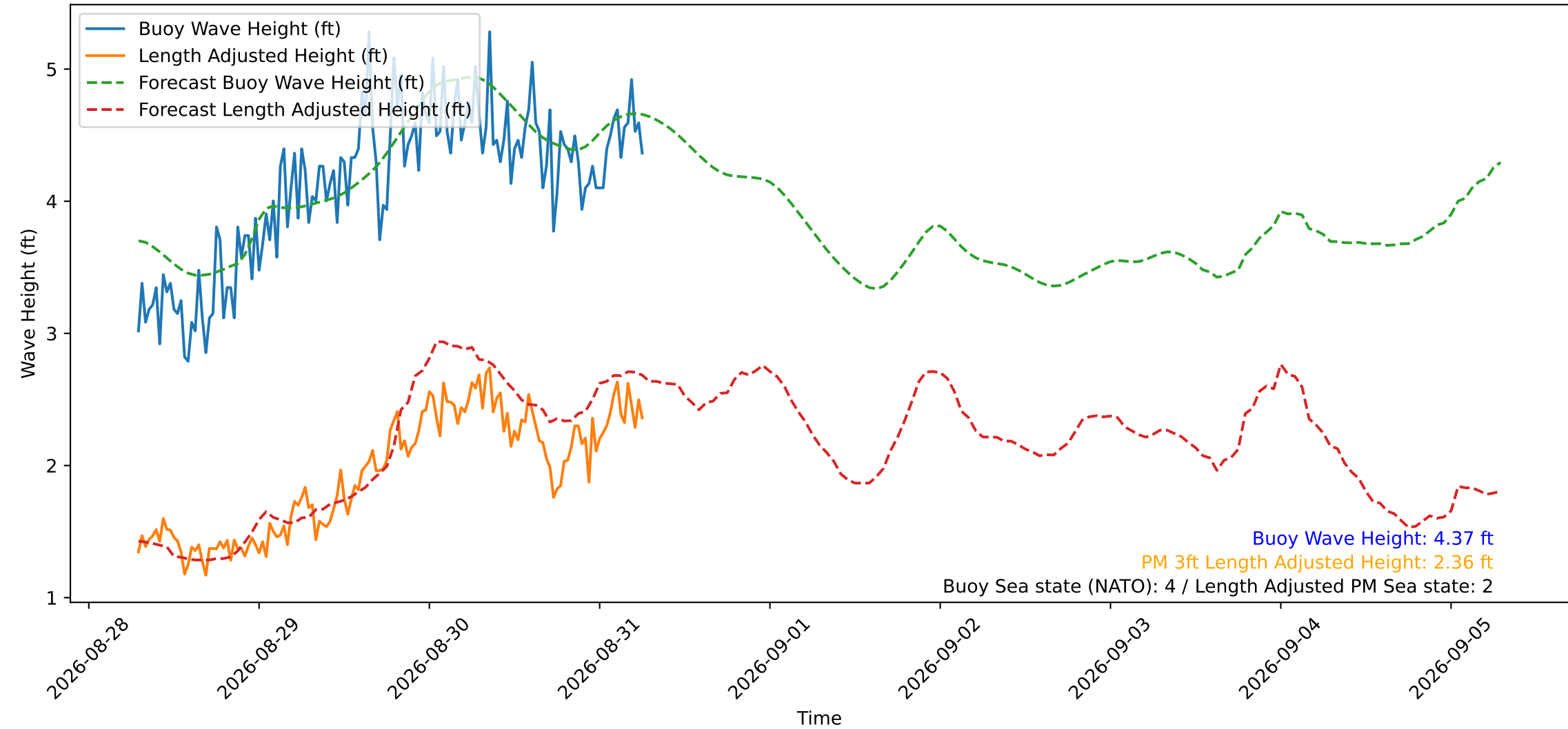
Wave Heights over Time for Oceanside Harbor at 2026-08-31 06:50:29
