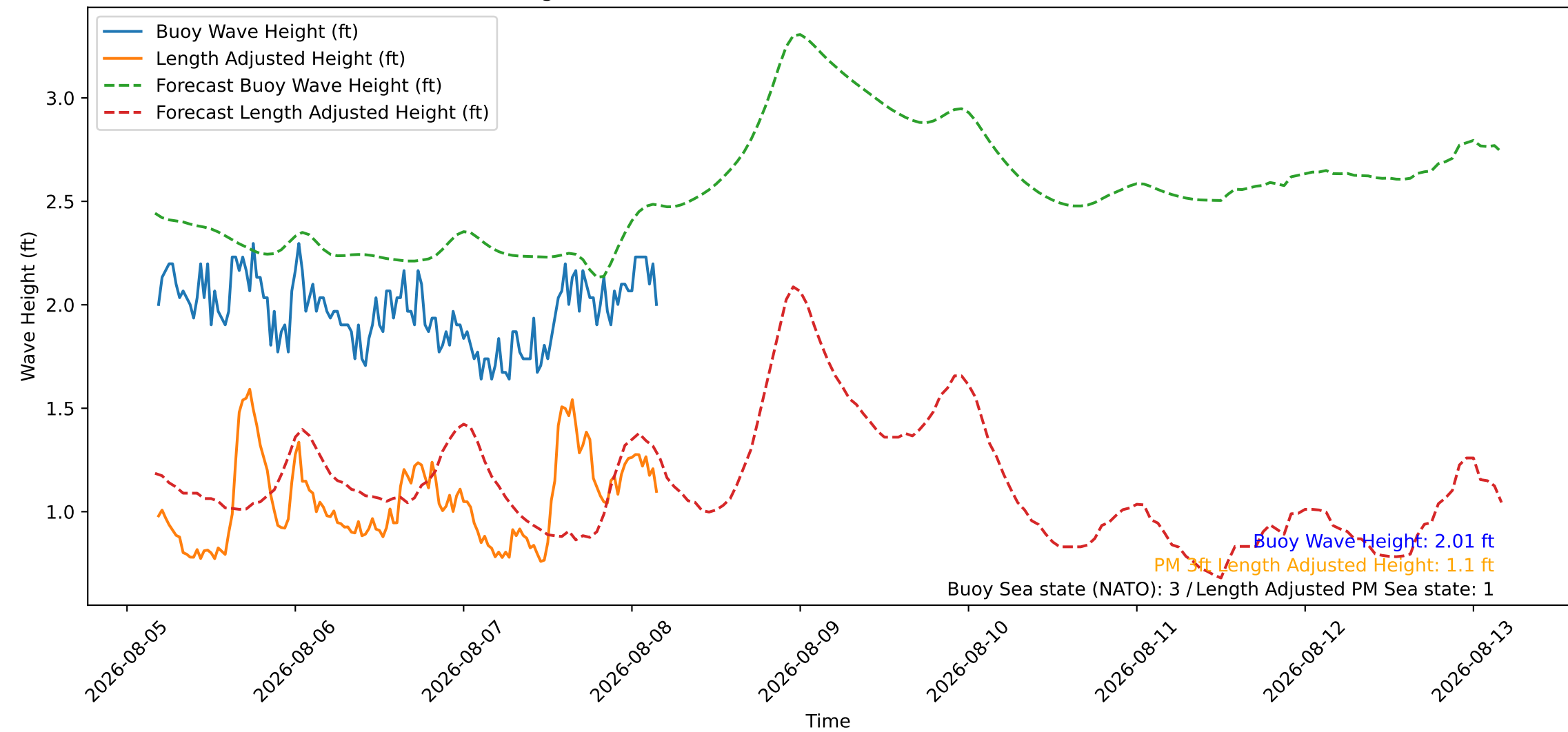
Wave Heights over Time for Oceanside Harbor at 2026-08-08 04:20:26
