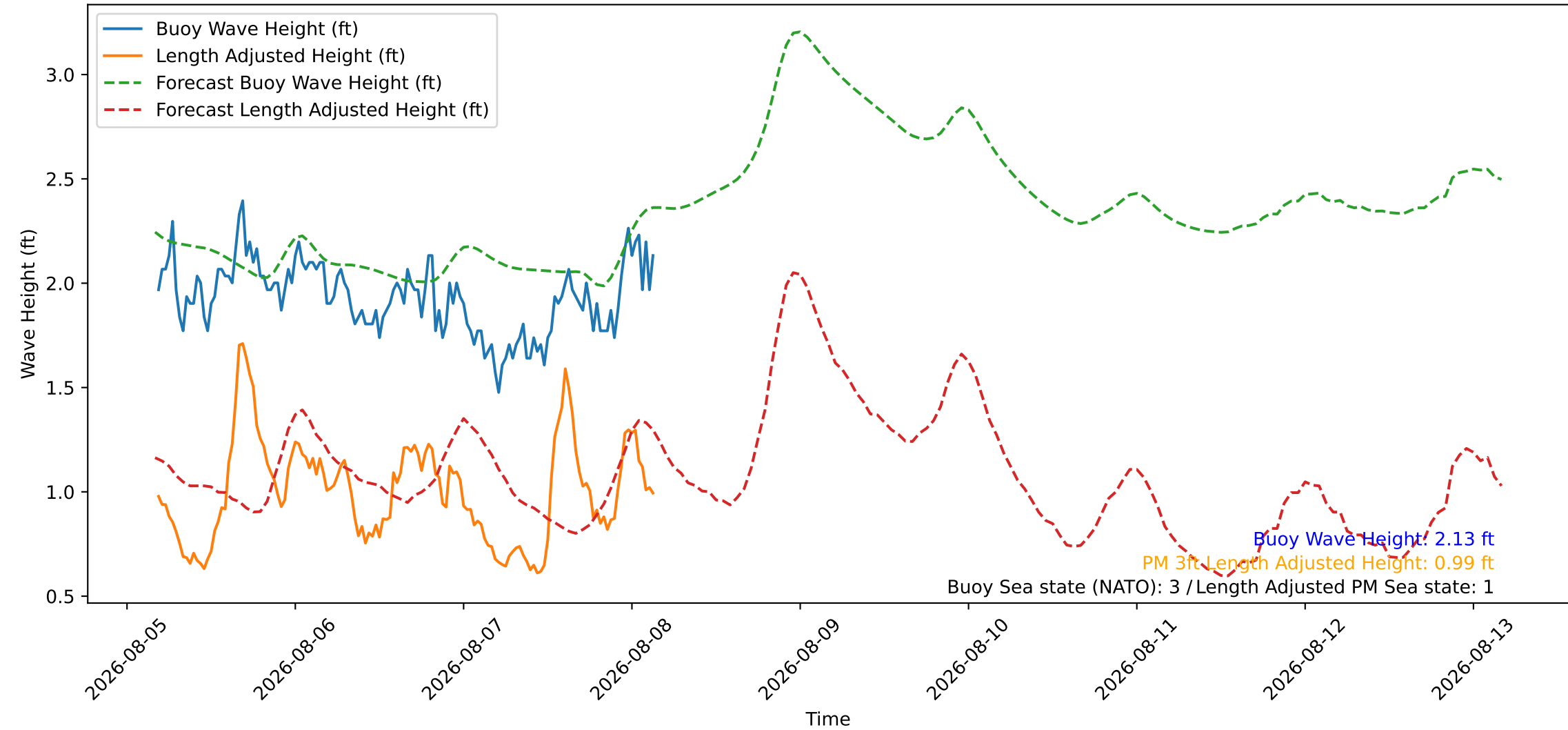
Wave Heights over Time for Red Beach at 2026-08-08 04:20:47
