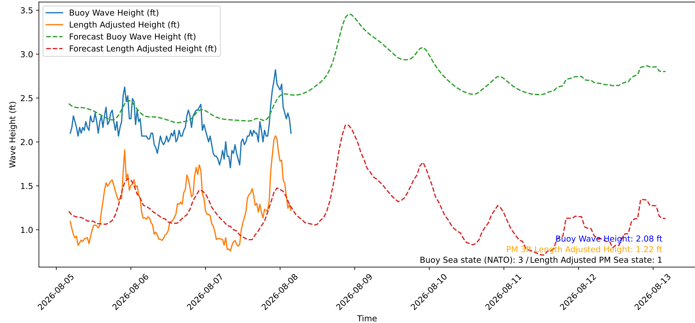
Wave Heights over Time for Green Beach at 2026-08-08 04:21:09
