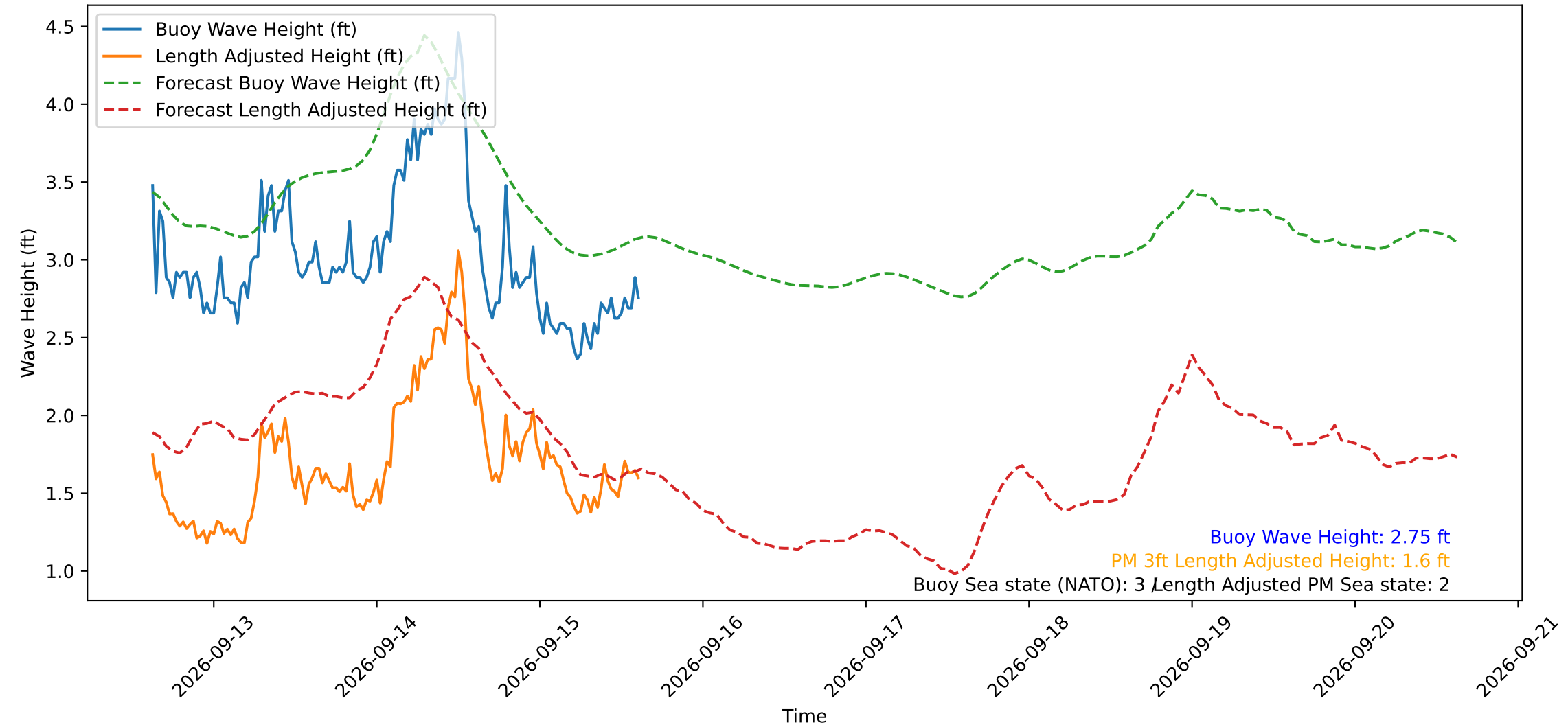
Wave Heights over Time for Oceanside Harbor at 2026-09-15 15:00:29
