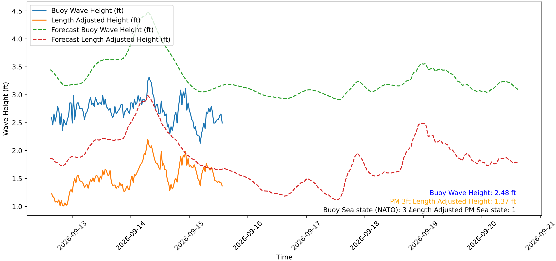
Wave Heights over Time for Green Beach at 2026-09-15 15:01:12
