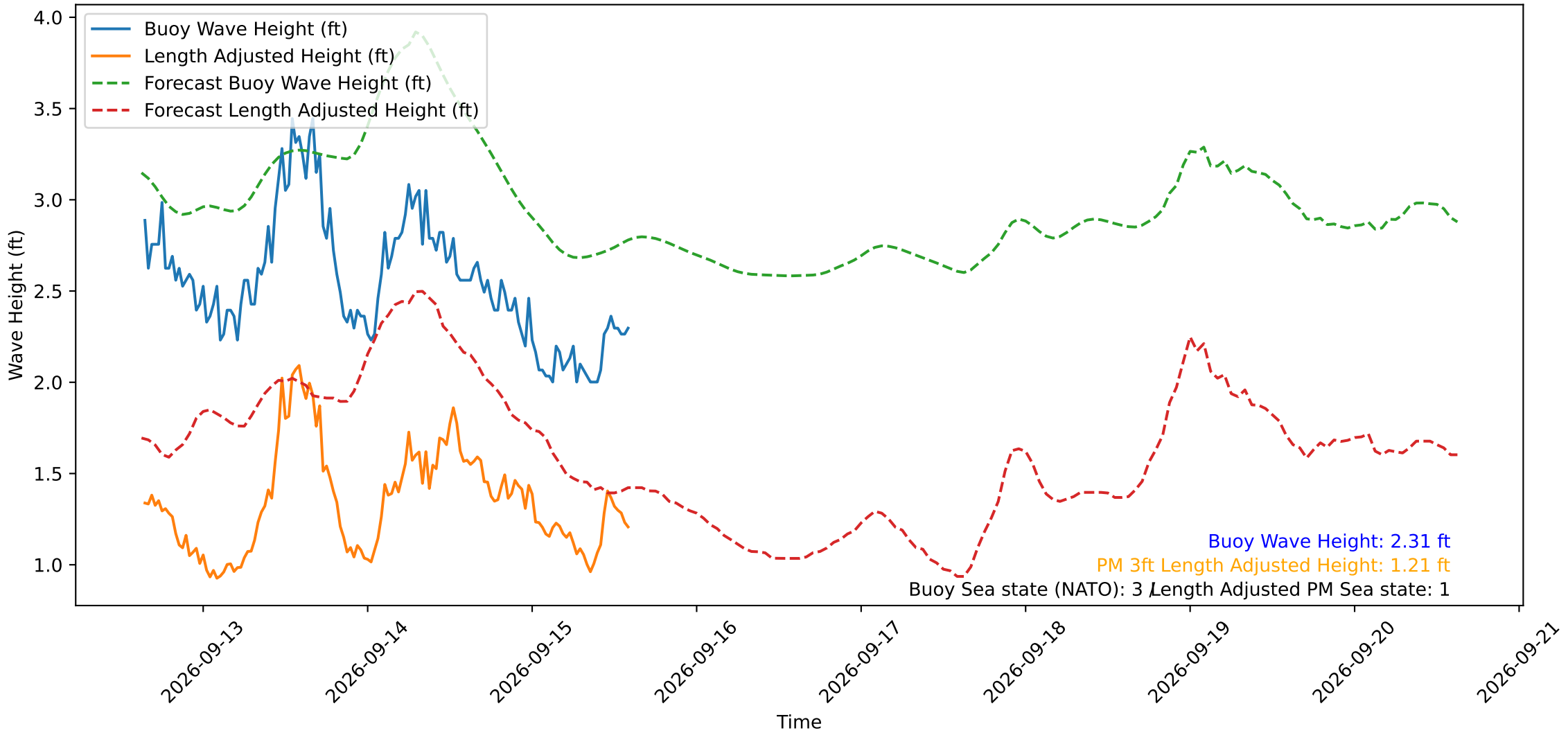
Wave Heights over Time for Red Beach at 2026-09-15 15:00:49
