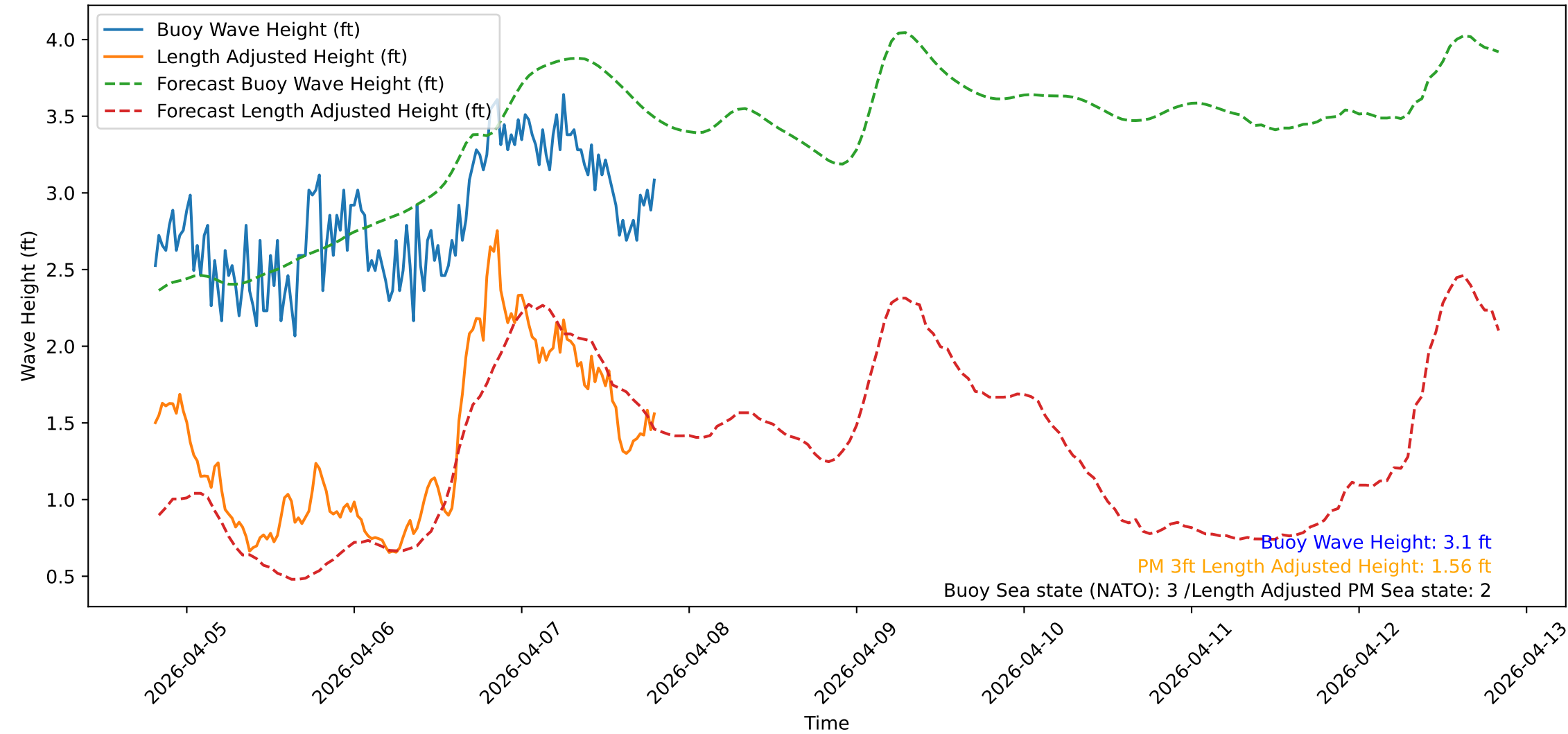
Wave Heights over Time for Oceanside Harbor at 2026-04-07 19:40:32
