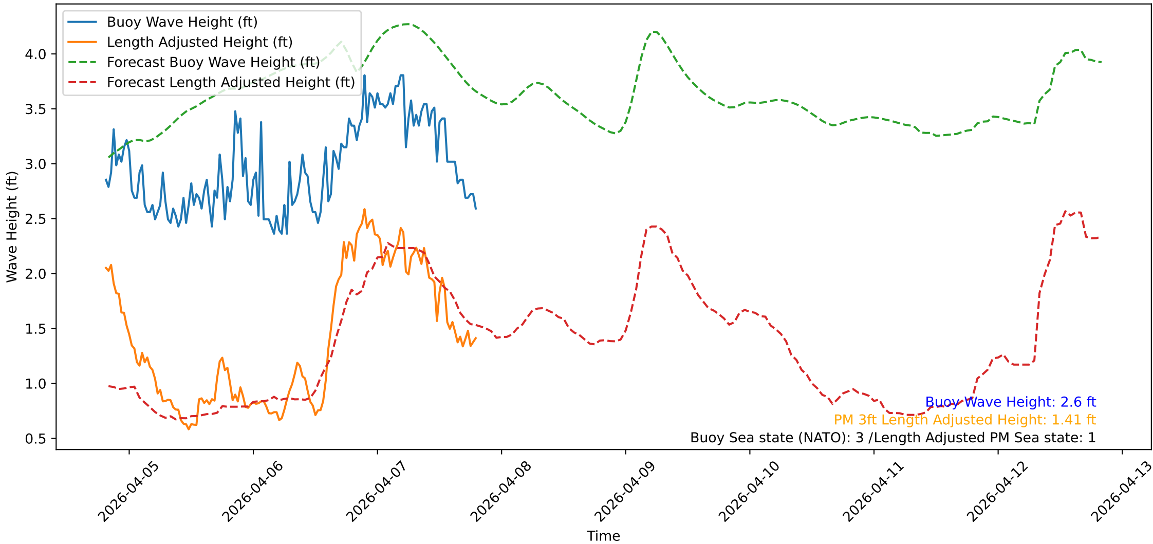
Wave Heights over Time for Green Beach at 2026-04-07 19:41:12
