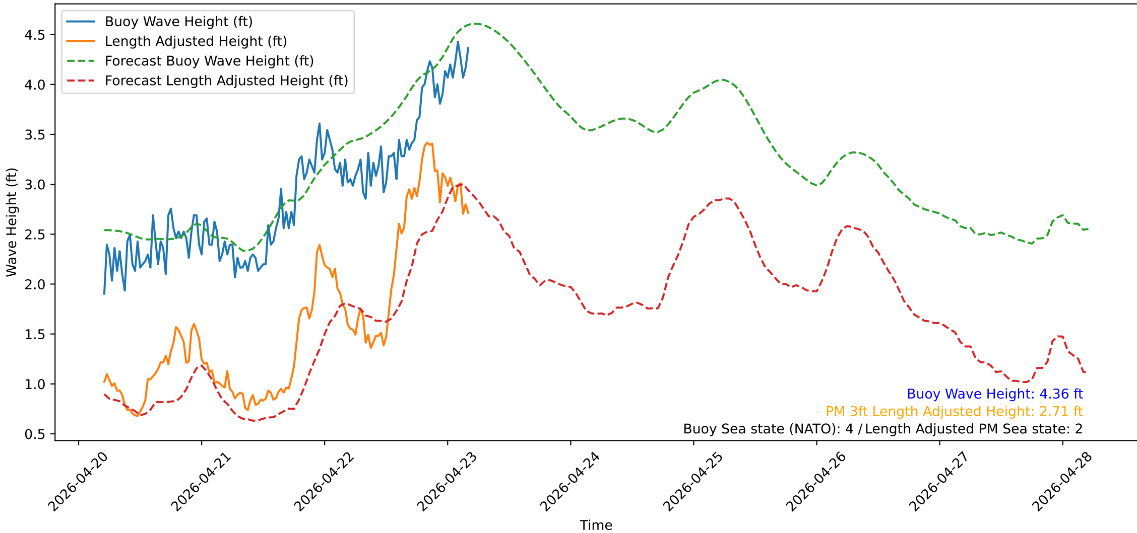
Wave Heights over Time for Oceanside Harbor at 2026-04-23 04:50:31
