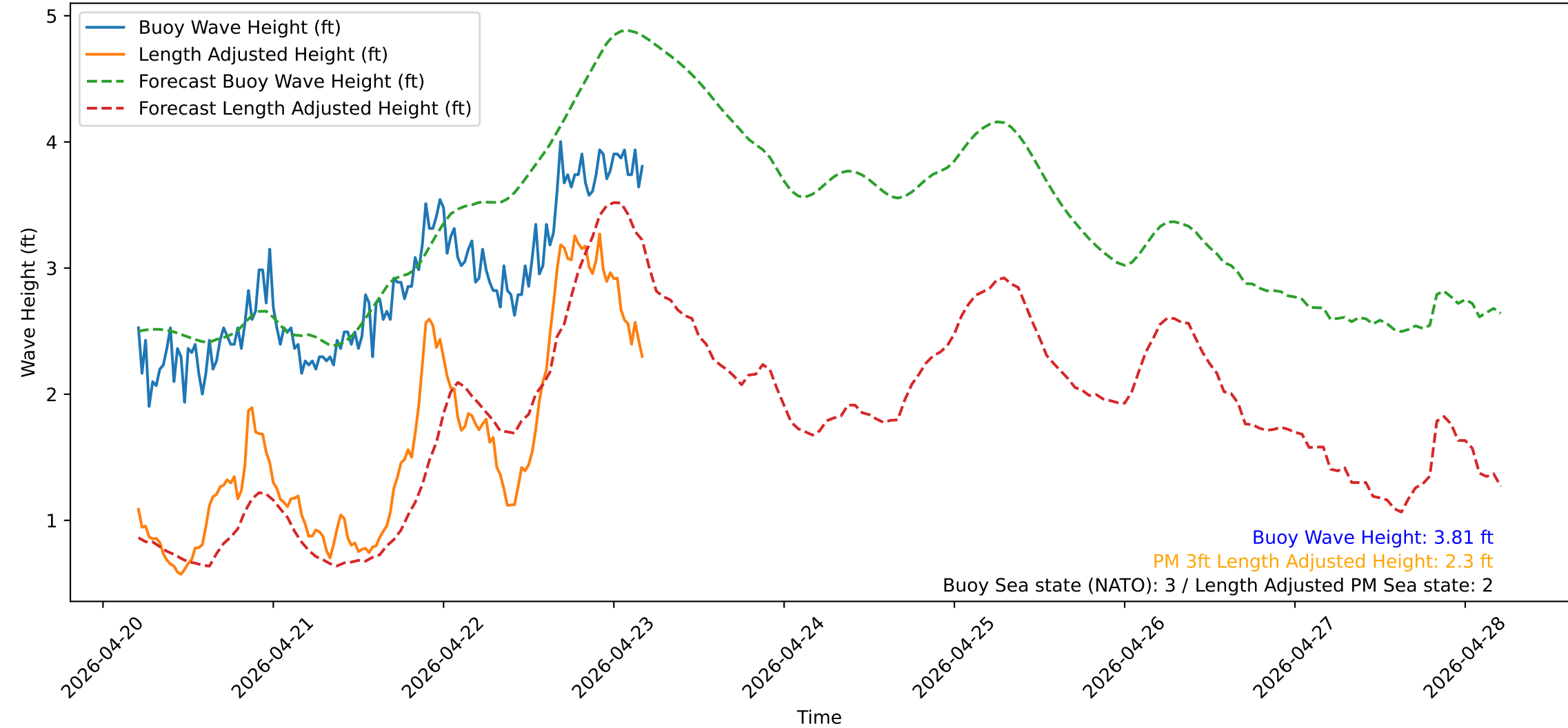
Wave Heights over Time for Green Beach at 2026-04-23 04:51:14
