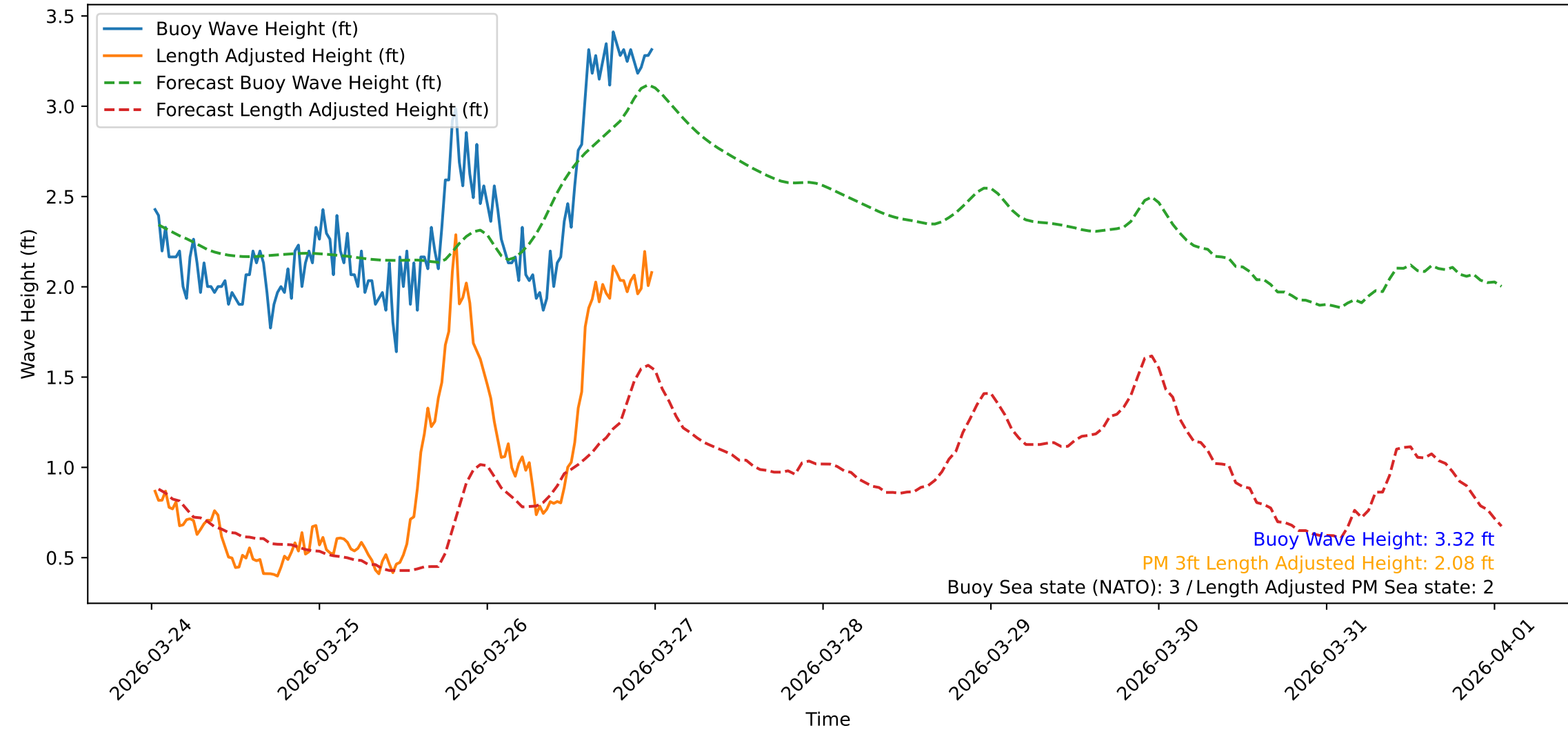
Wave Heights over Time for Green Beach at 2026-03-27 00:31:09
