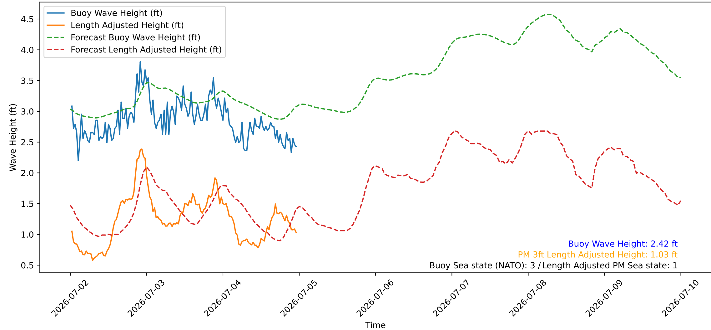
Wave Heights over Time for Red Beach at 2026-07-05 00:00:45
