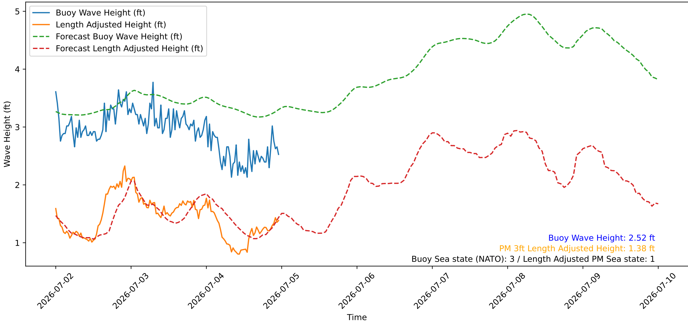
Wave Heights over Time for Oceanside Harbor at 2026-07-05 00:00:26
