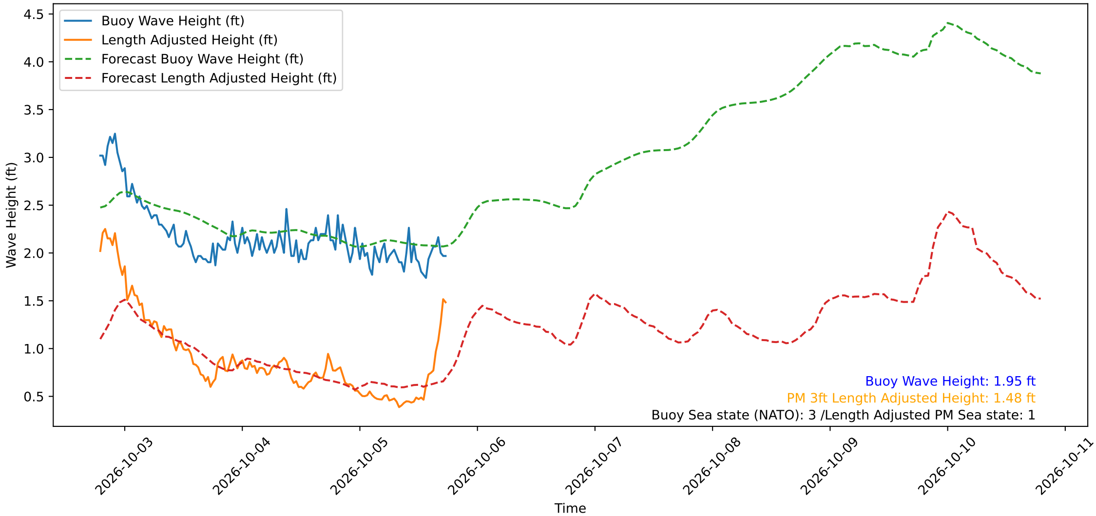
Wave Heights over Time for Red Beach at 2026-10-05 18:30:49
