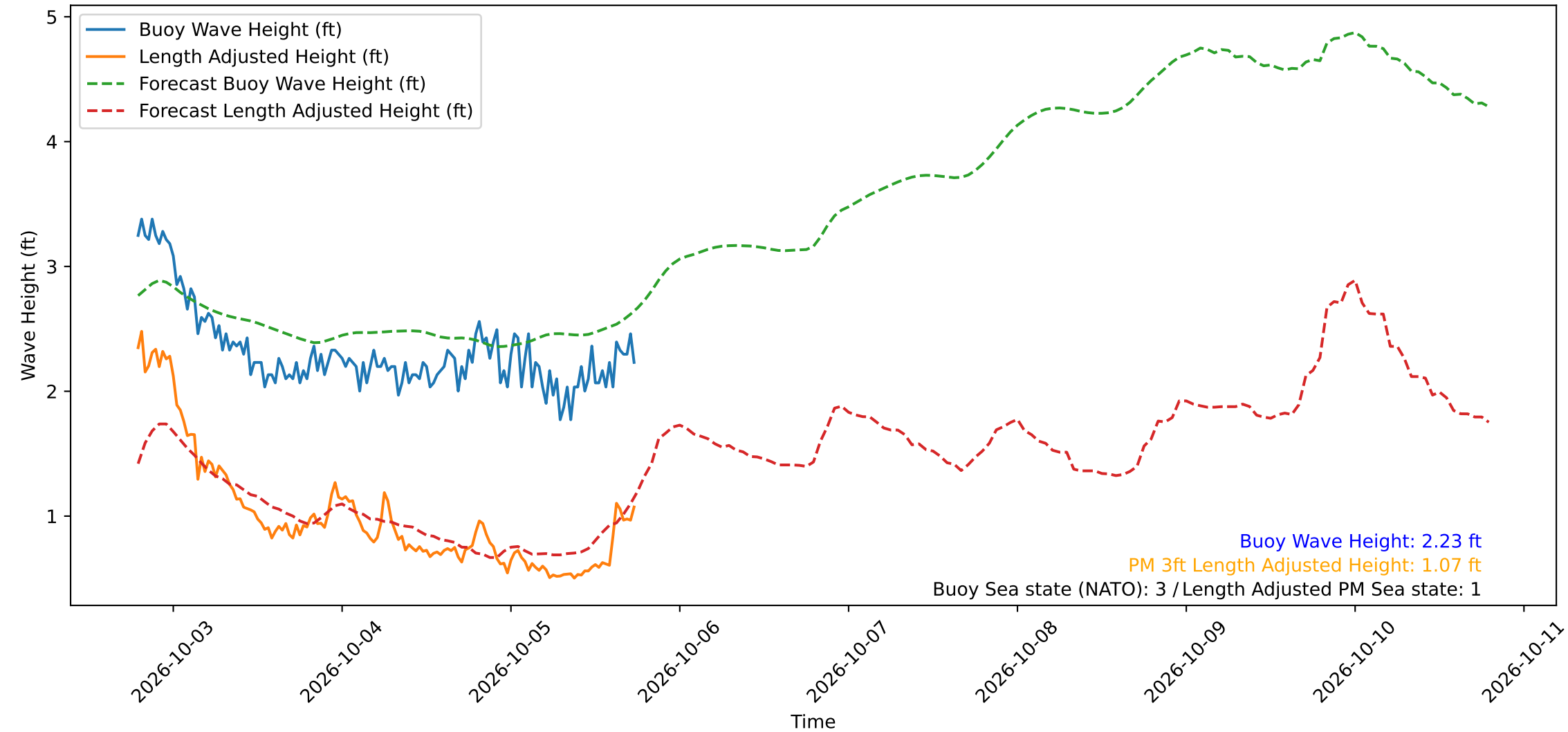
Wave Heights over Time for Green Beach at 2026-10-05 18:31:11
