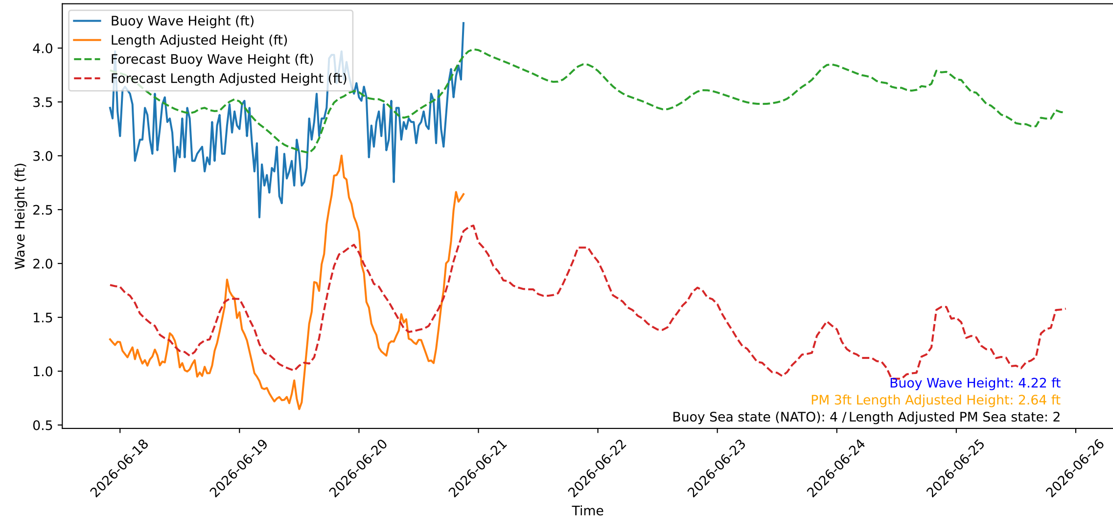
Wave Heights over Time for Green Beach at 2026-06-20 21:51:09
