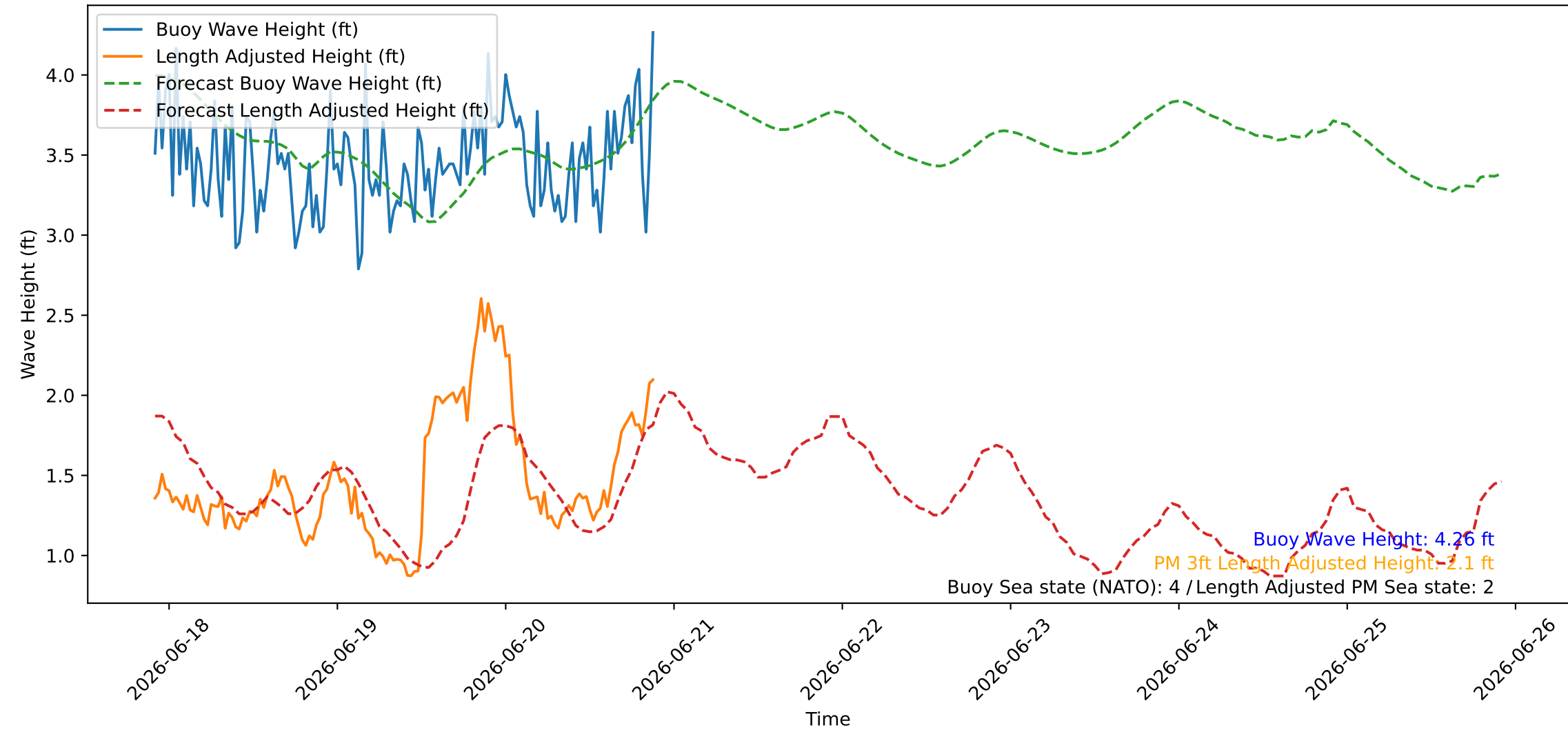
Wave Heights over Time for Oceanside Harbor at 2026-06-20 21:50:26
