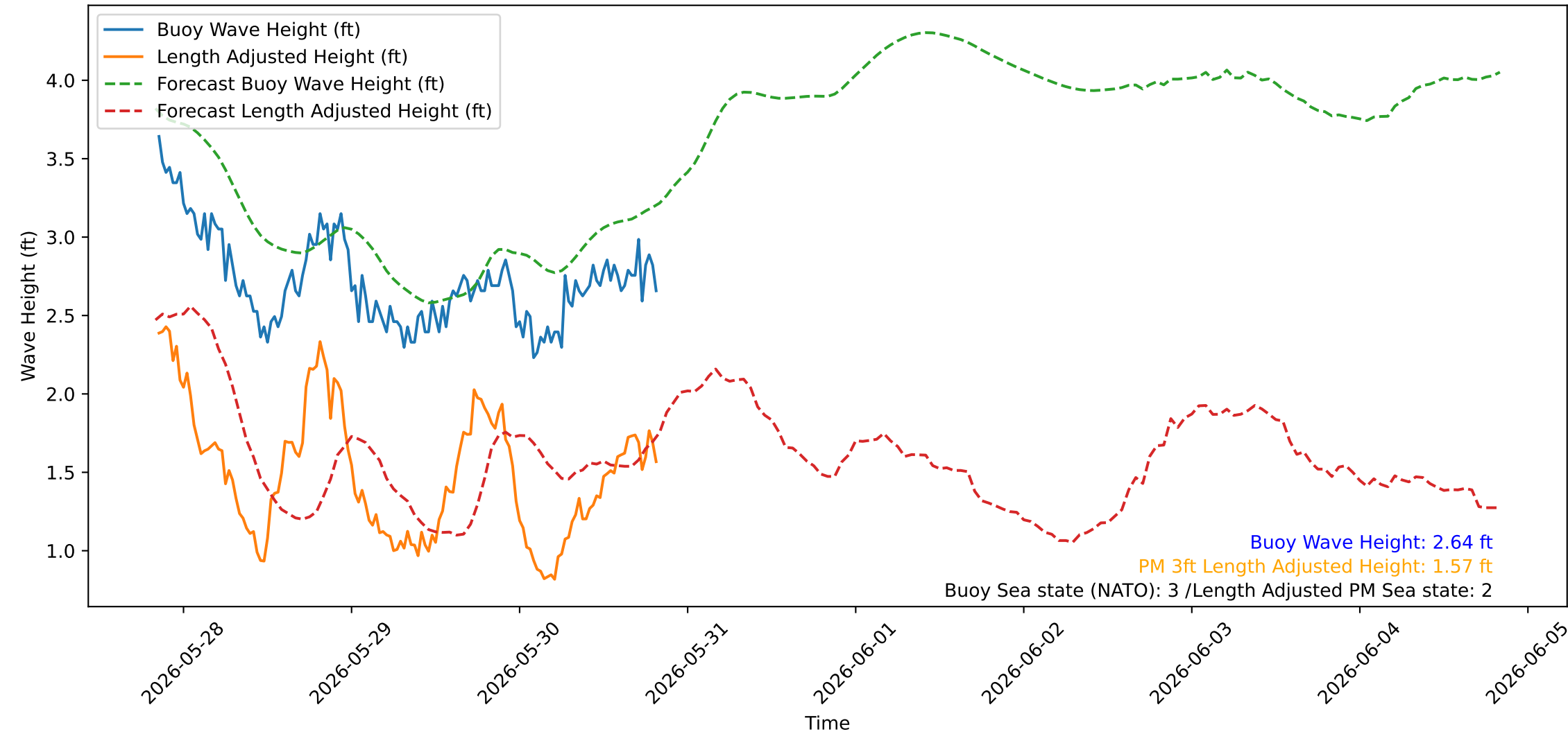
Wave Heights over Time for Red Beach at 2026-05-30 20:10:43
