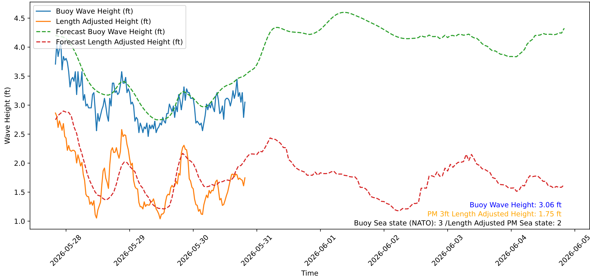
Wave Heights over Time for Green Beach at 2026-05-30 20:11:06
