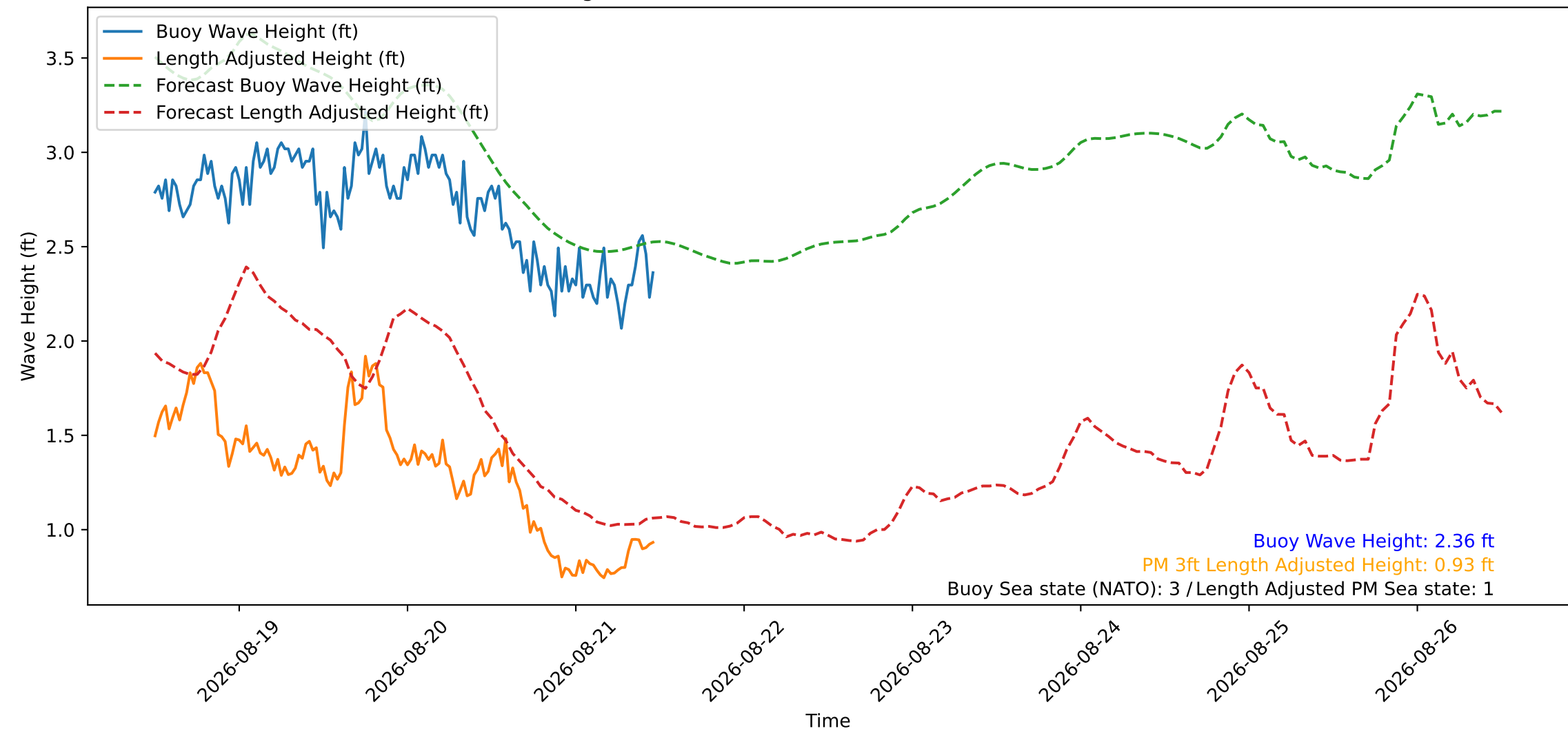
Wave Heights over Time for Red Beach at 2026-08-21 11:40:45
