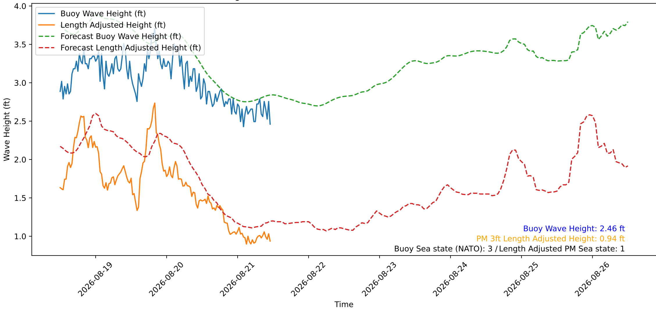
Wave Heights over Time for Green Beach at 2026-08-21 11:41:08
