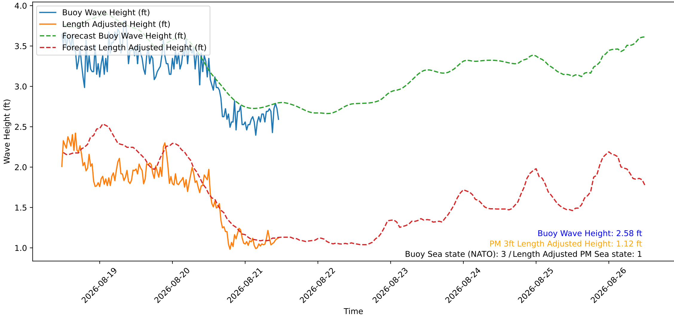
Wave Heights over Time for Oceanside Harbor at 2026-08-21 11:40:26
