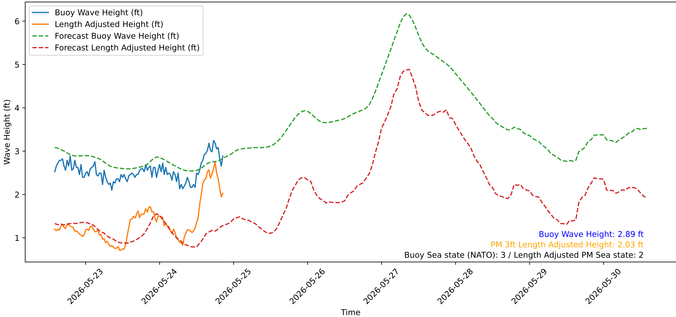
Wave Heights over Time for Oceanside Harbor at 2026-05-25 13:50:30
