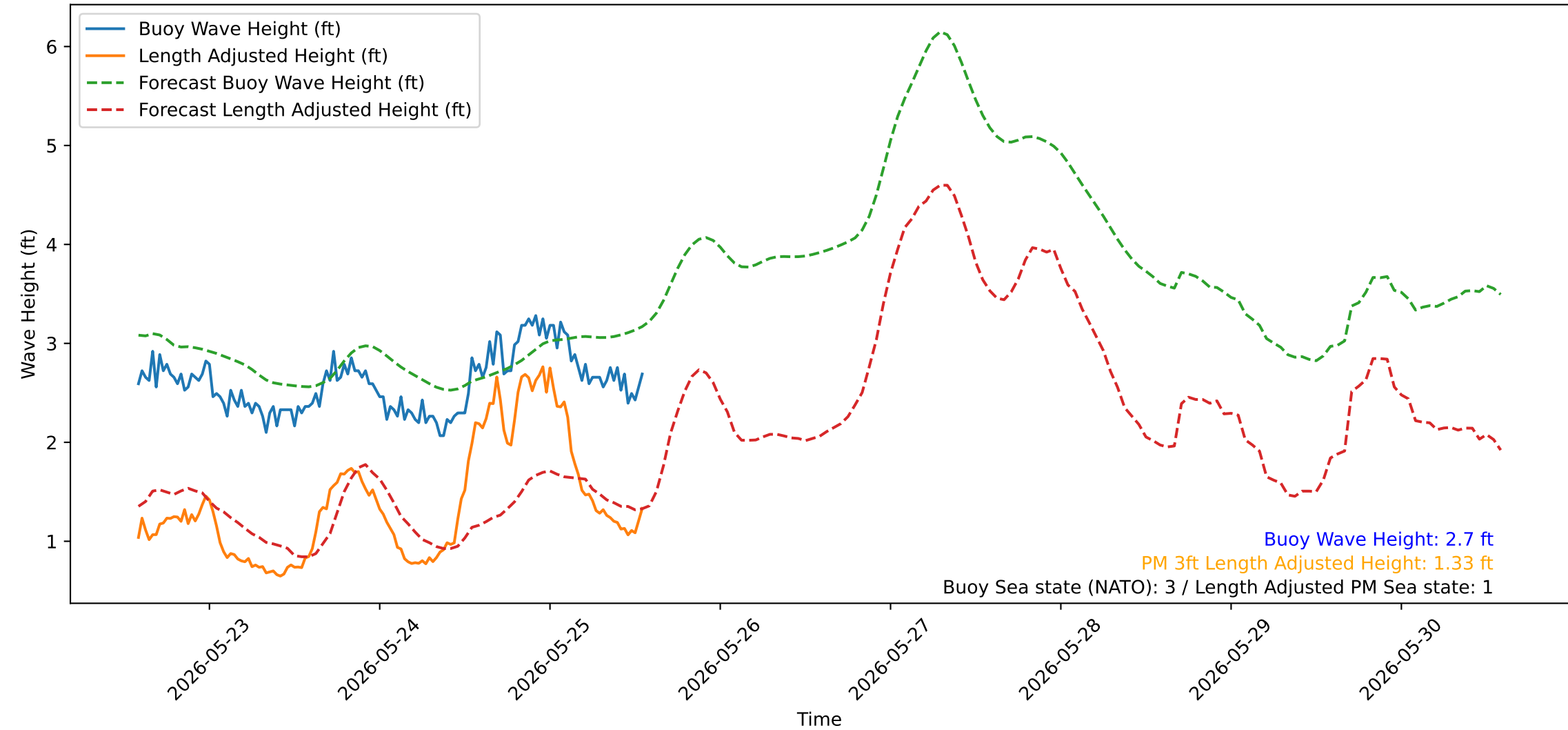
Wave Heights over Time for Green Beach at 2026-05-25 13:51:12
