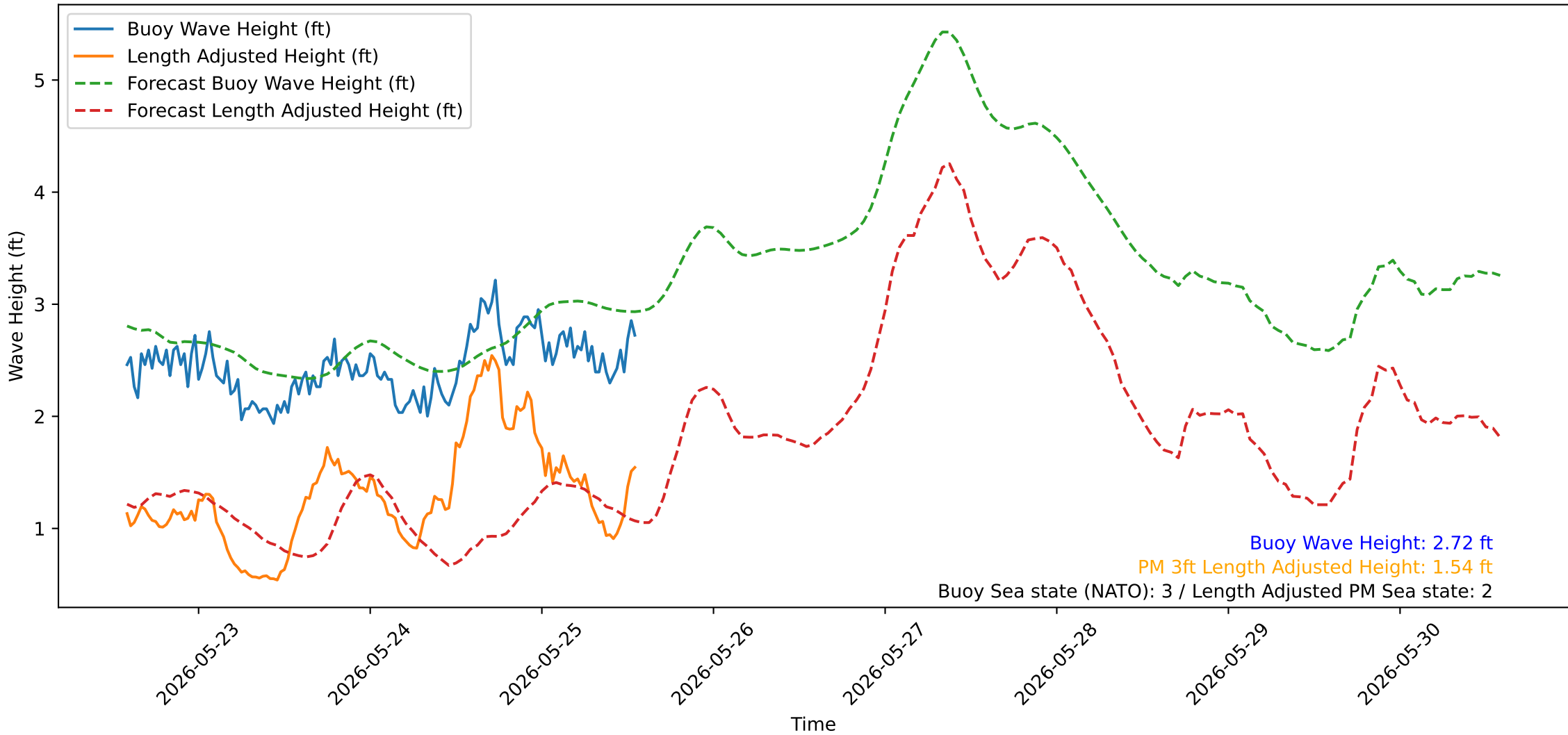
Wave Heights over Time for Red Beach at 2026-05-25 13:50:50
