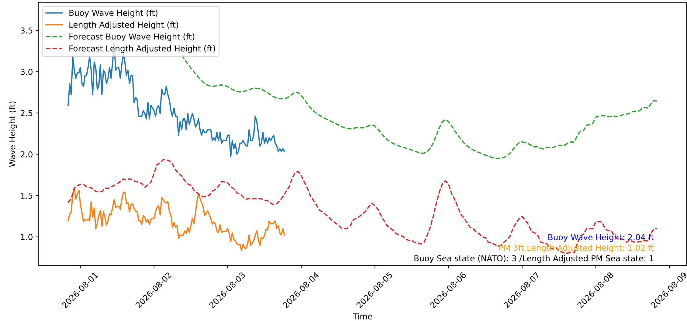
Wave Heights over Time for Red Beach at 2026-08-03 19:40:46
