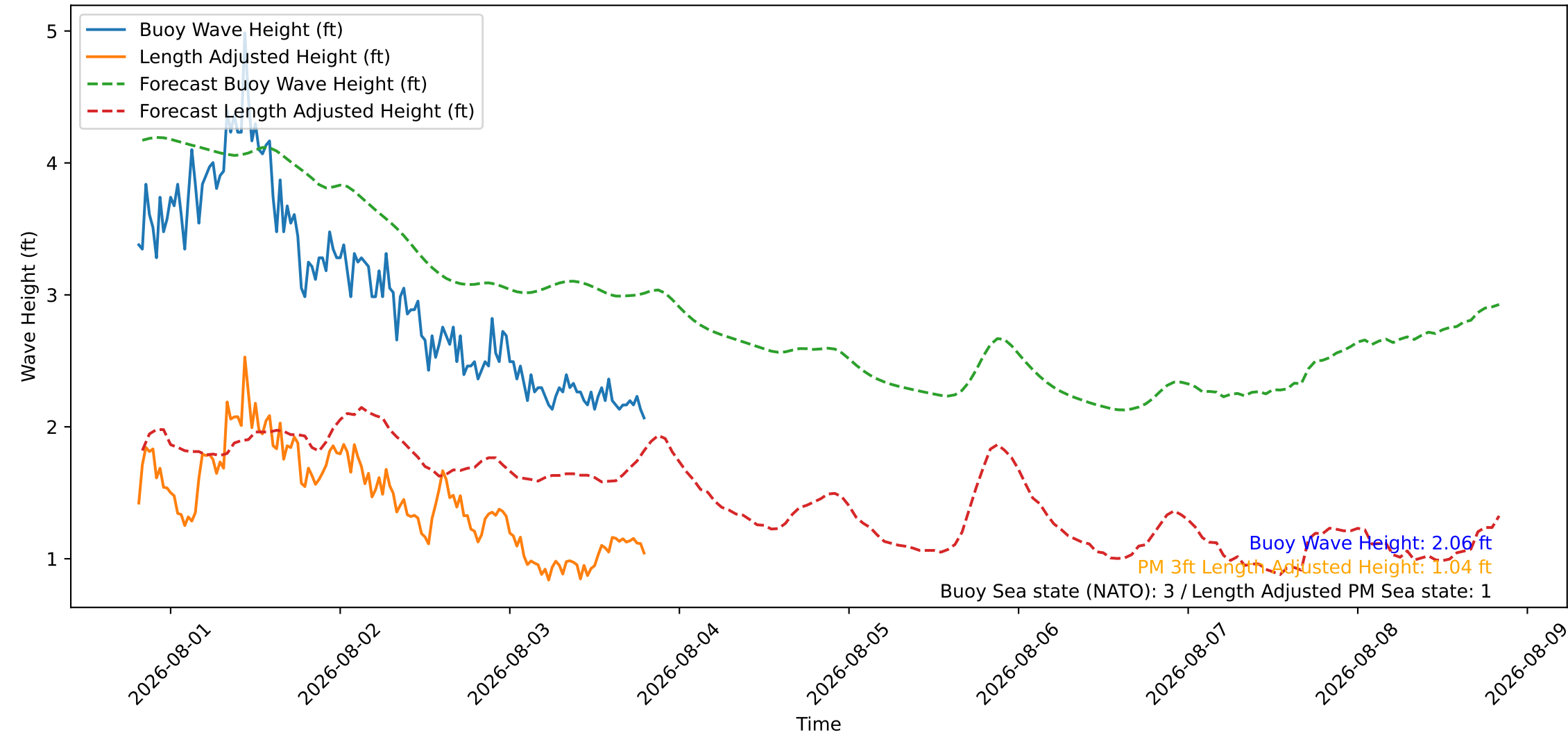
Wave Heights over Time for Green Beach at 2026-08-03 19:41:09
