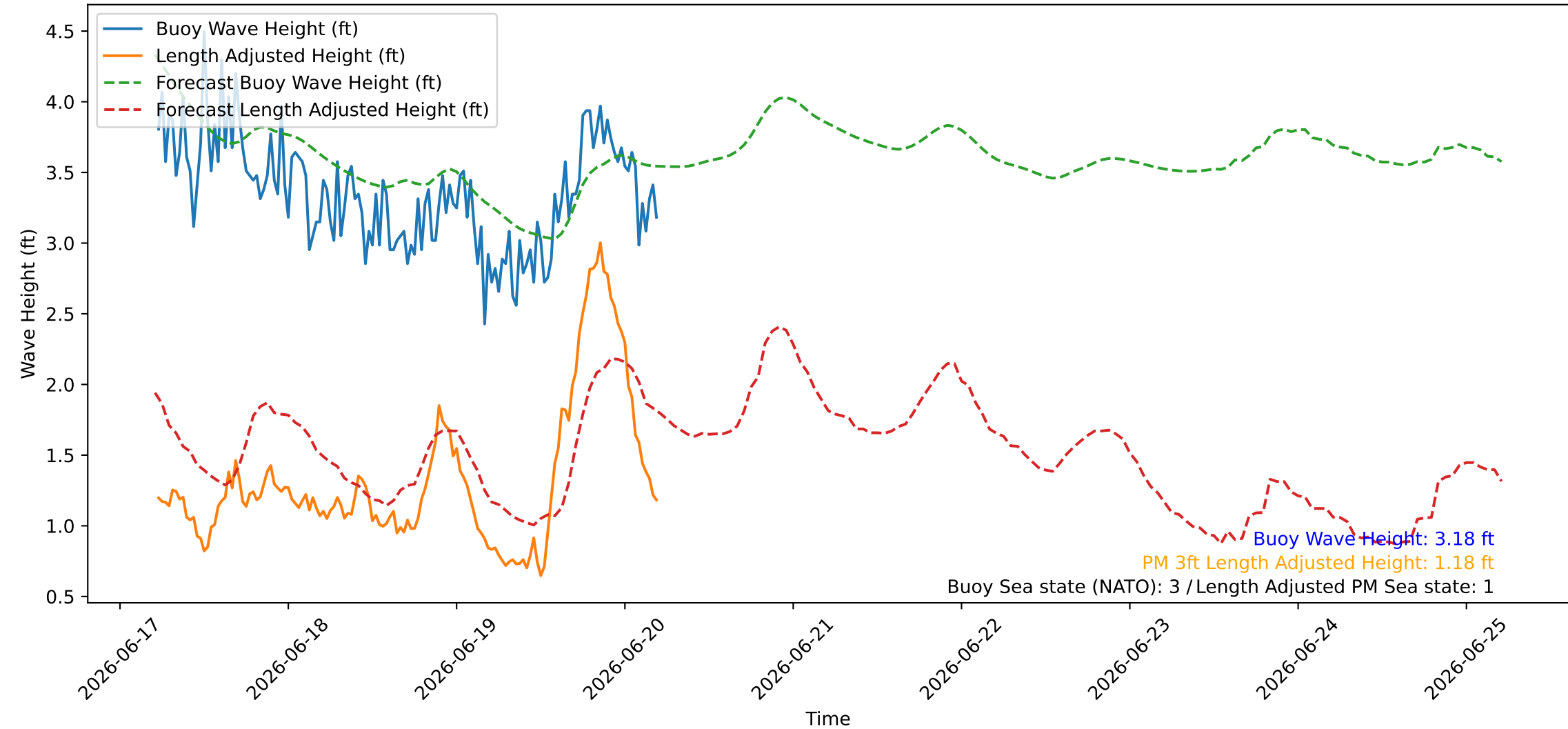
Wave Heights over Time for Green Beach at 2026-06-20 05:21:09
