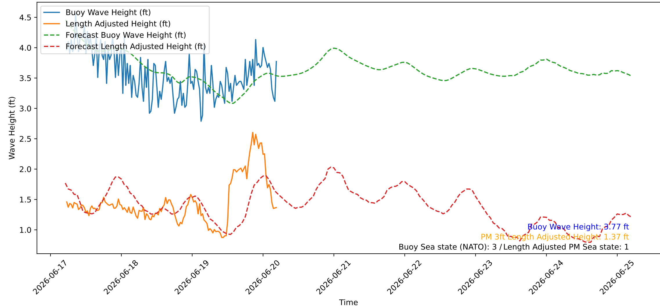
Wave Heights over Time for Oceanside Harbor at 2026-06-20 05:20:26
