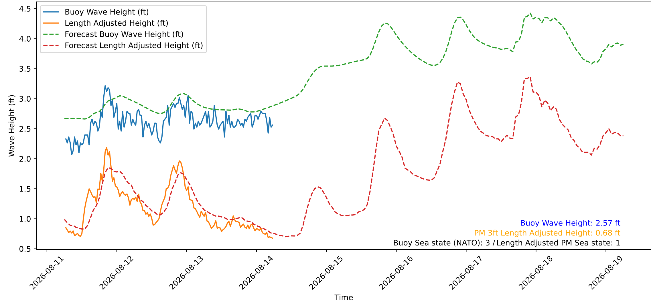
Wave Heights over Time for Green Beach at 2026-08-14 06:21:09
