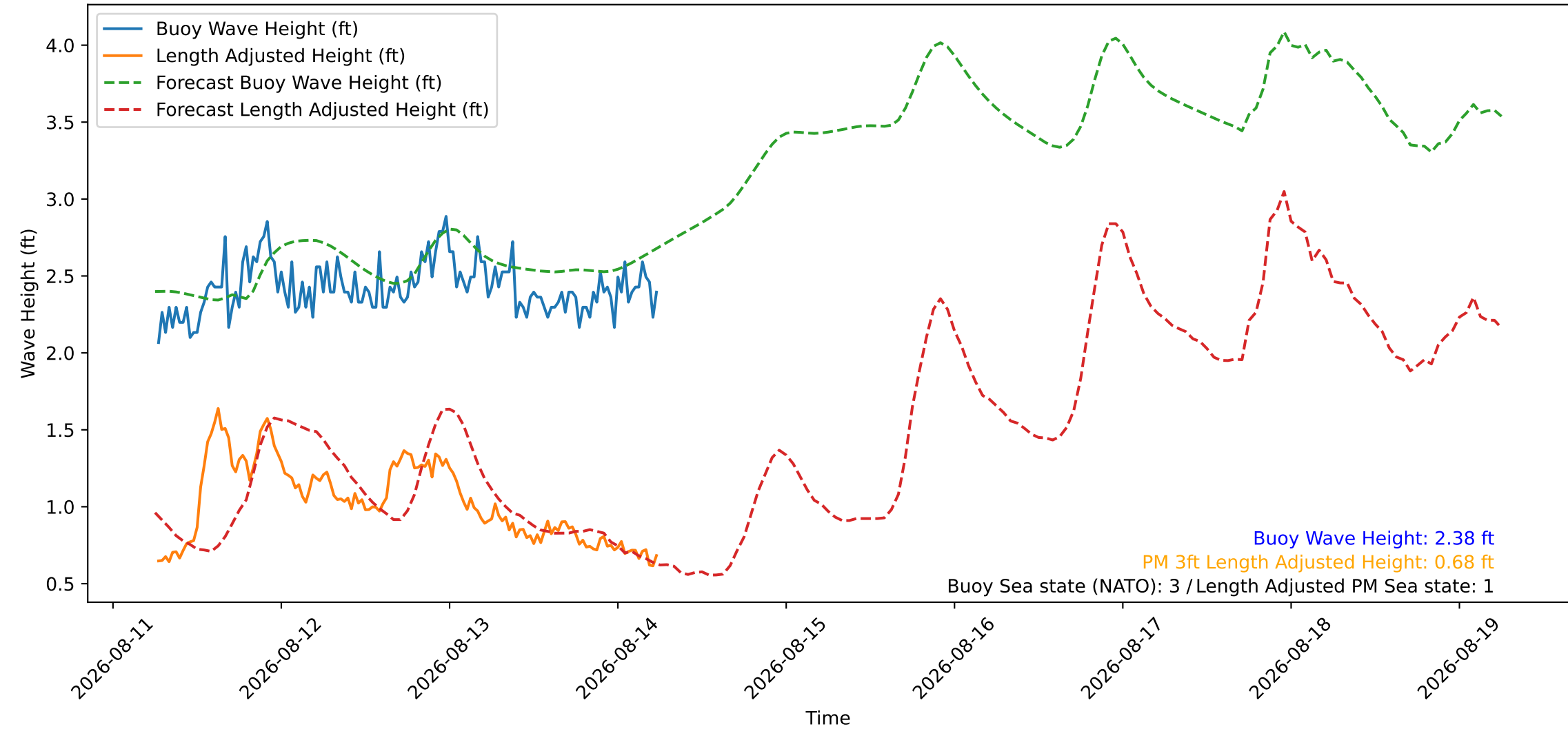
Wave Heights over Time for Red Beach at 2026-08-14 06:20:46
