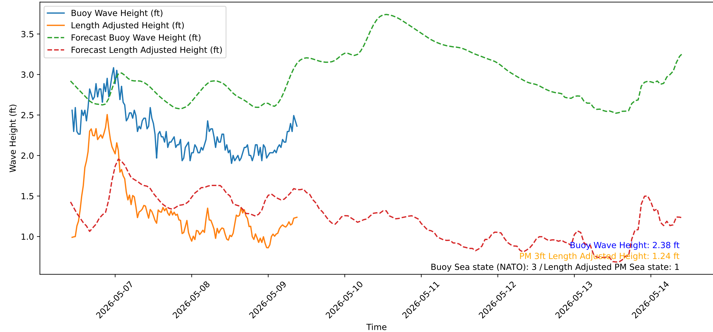
Wave Heights over Time for Red Beach at 2026-05-09 10:00:50
