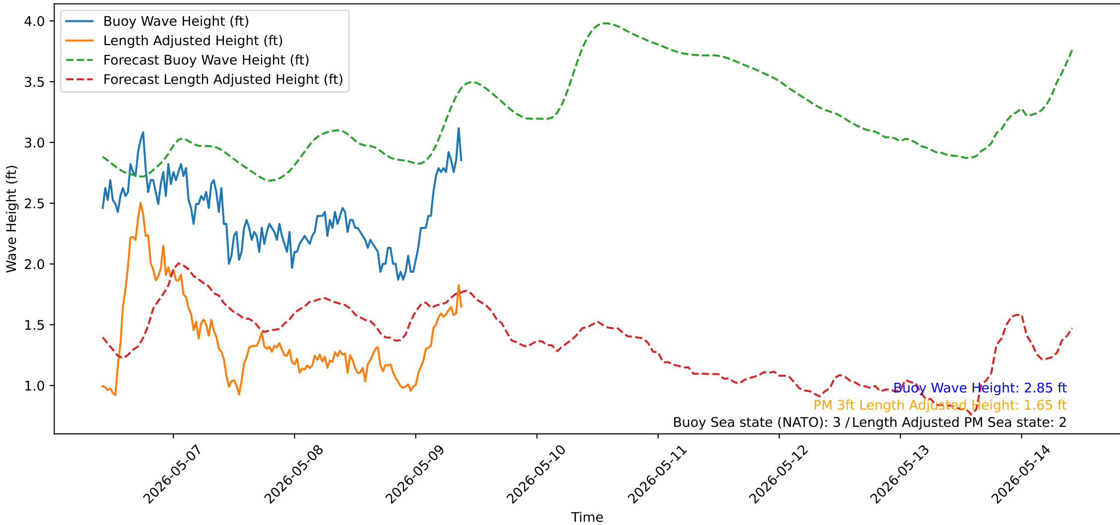
Wave Heights over Time for Oceanside Harbor at 2026-05-09 10:00:31
