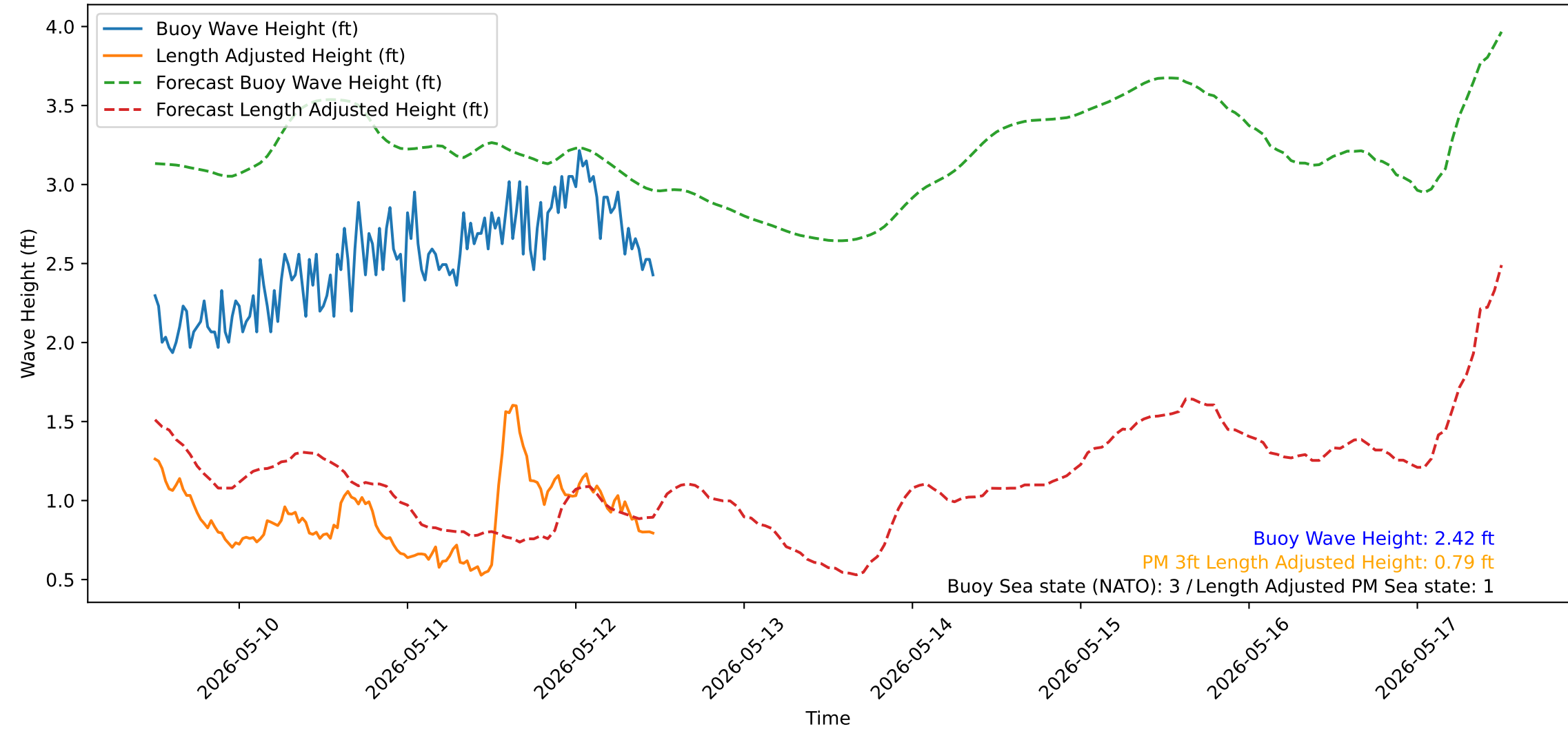
Wave Heights over Time for Red Beach at 2026-05-12 11:50:51
