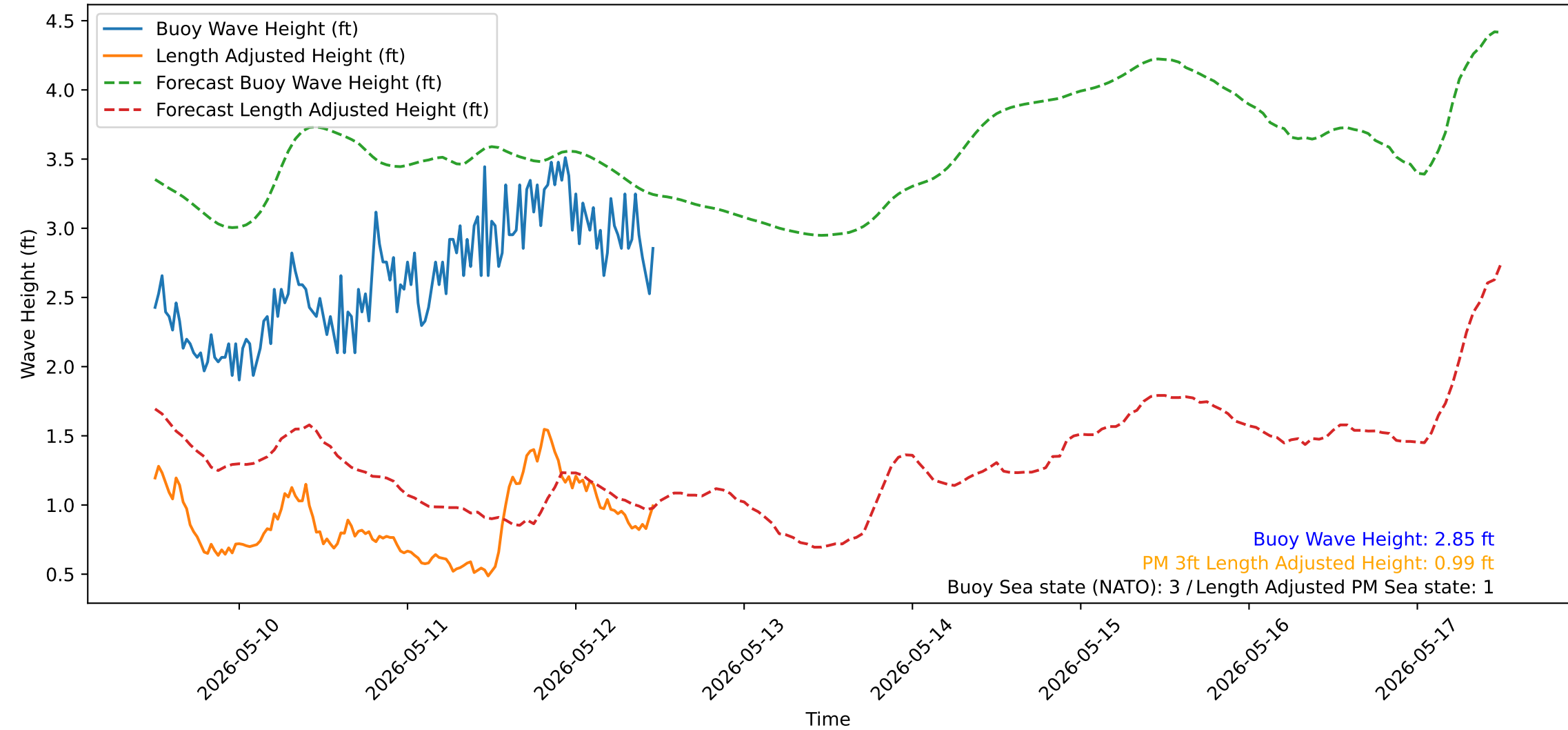
Wave Heights over Time for Green Beach at 2026-05-12 11:51:14
