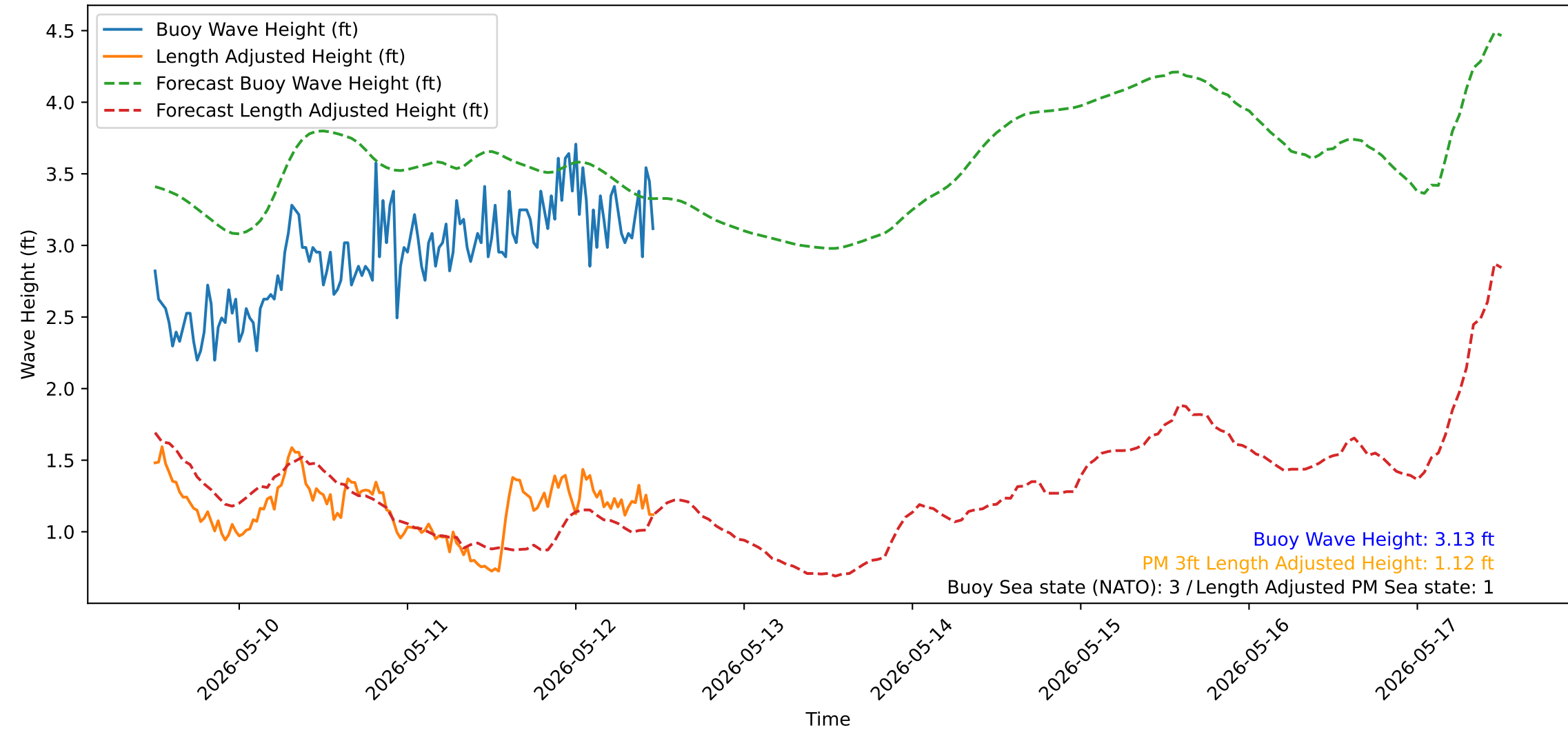
Wave Heights over Time for Oceanside Harbor at 2026-05-12 11:50:31
