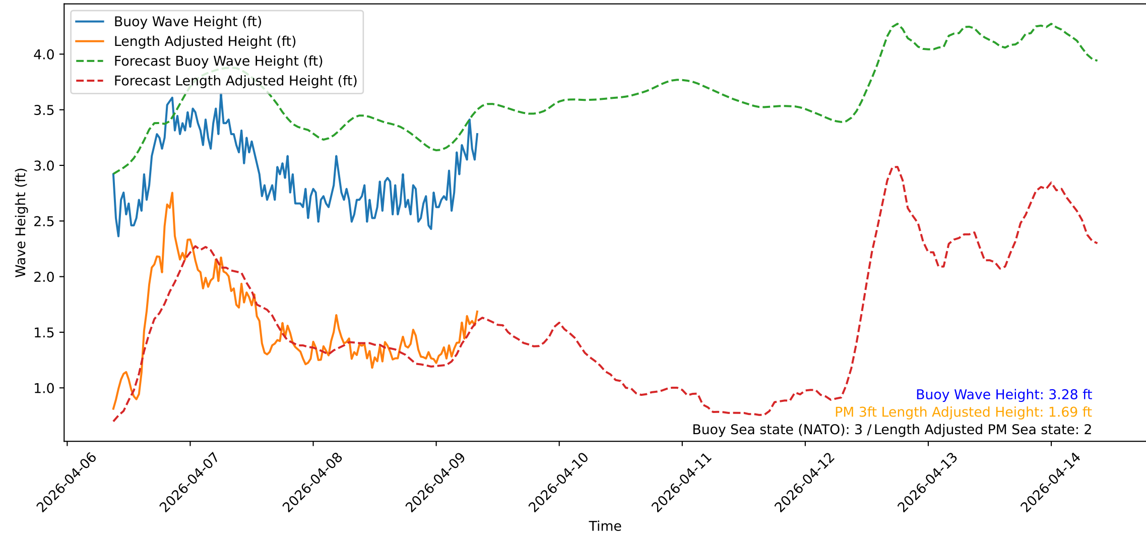
Wave Heights over Time for Oceanside Harbor at 2026-04-09 08:50:31
