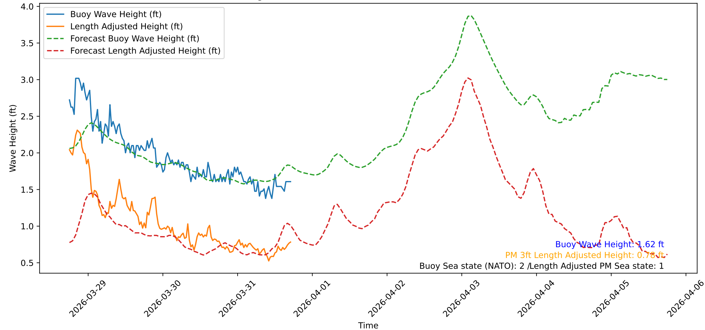
Wave Heights over Time for Red Beach at 2026-03-31 17:50:47
