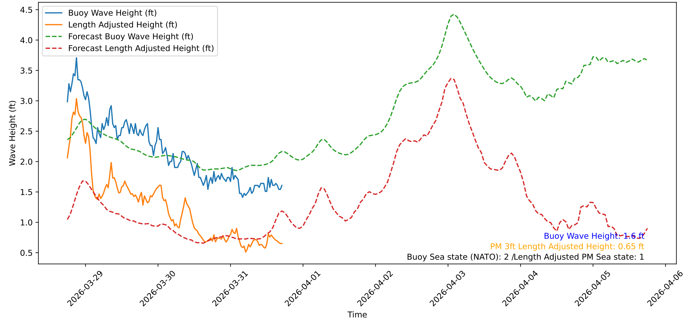
Wave Heights over Time for Green Beach at 2026-03-31 17:51:10
