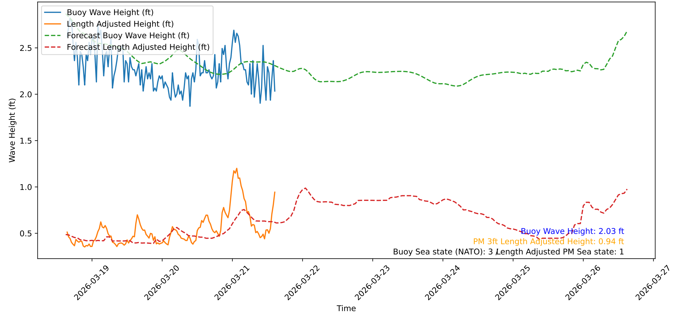
Wave Heights over Time for Red Beach at 2026-03-21 15:20:48
