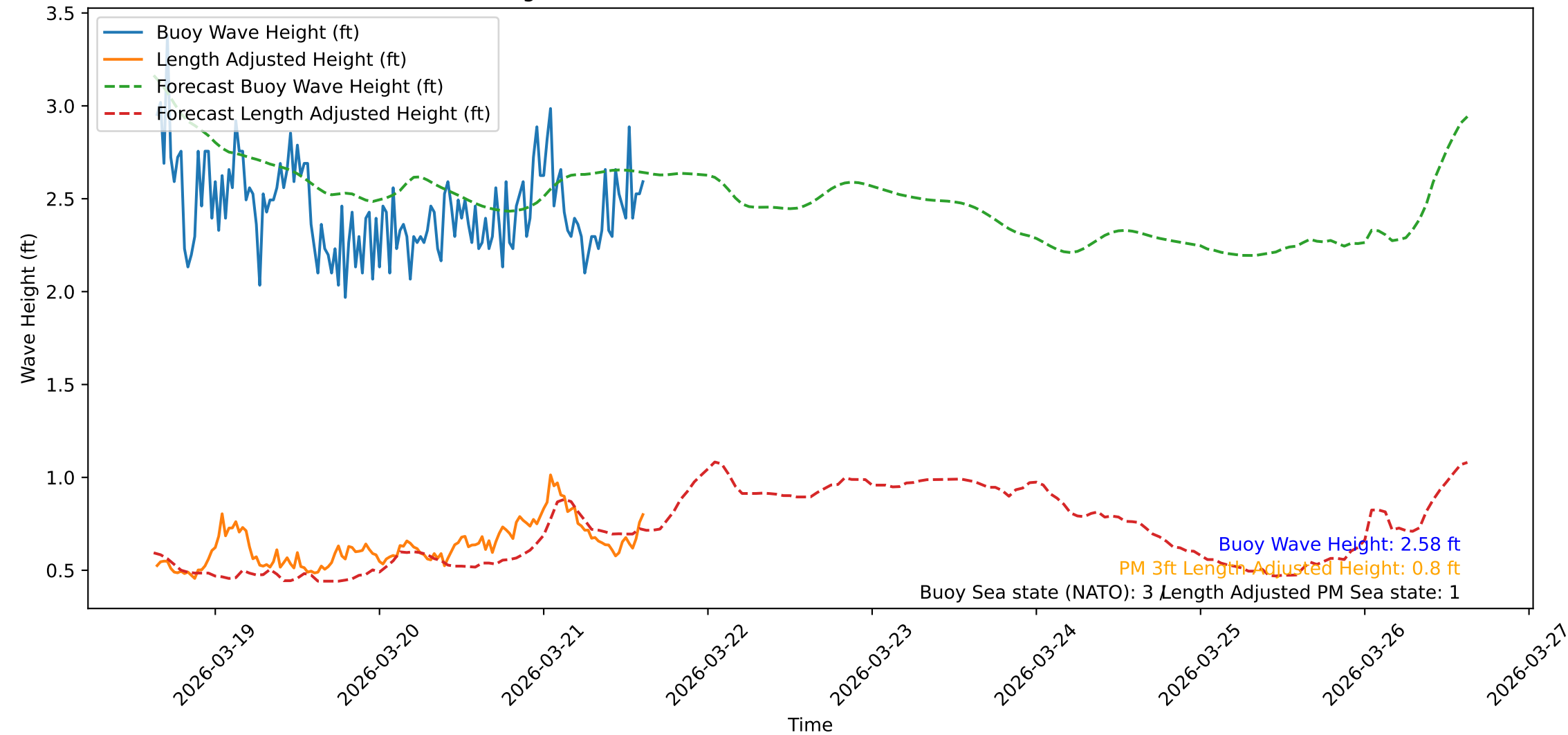
Wave Heights over Time for Oceanside Harbor at 2026-03-21 15:20:32
