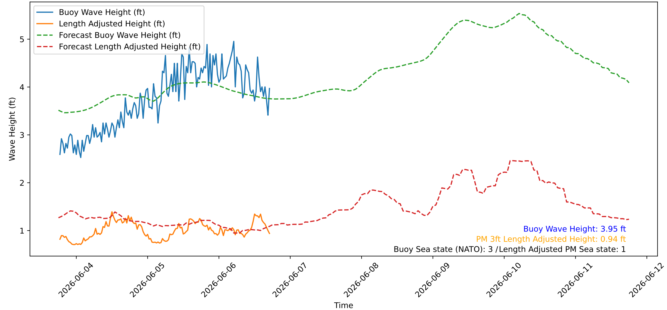
Wave Heights over Time for Red Beach at 2026-06-06 18:00:45
