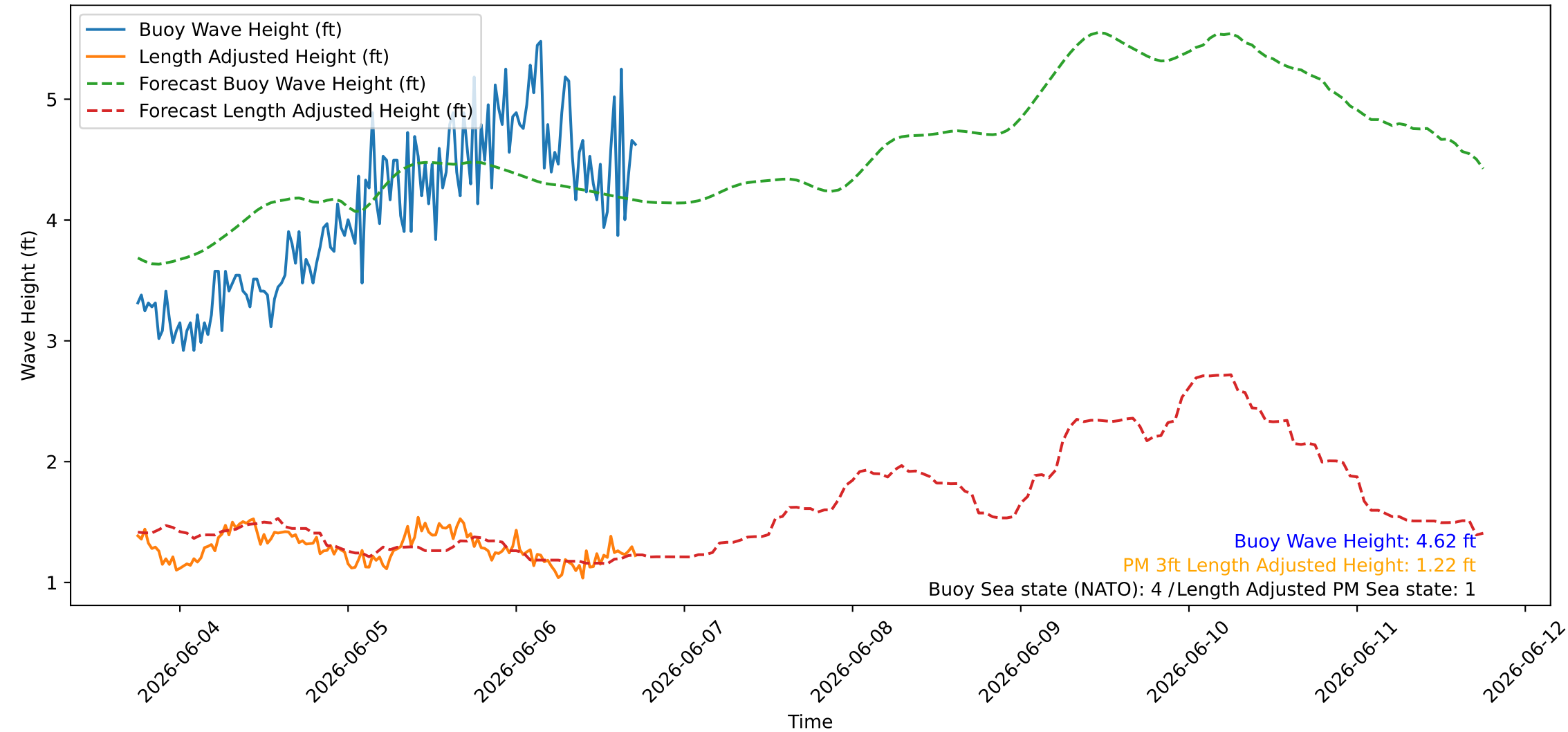
Wave Heights over Time for Oceanside Harbor at 2026-06-06 18:00:26
