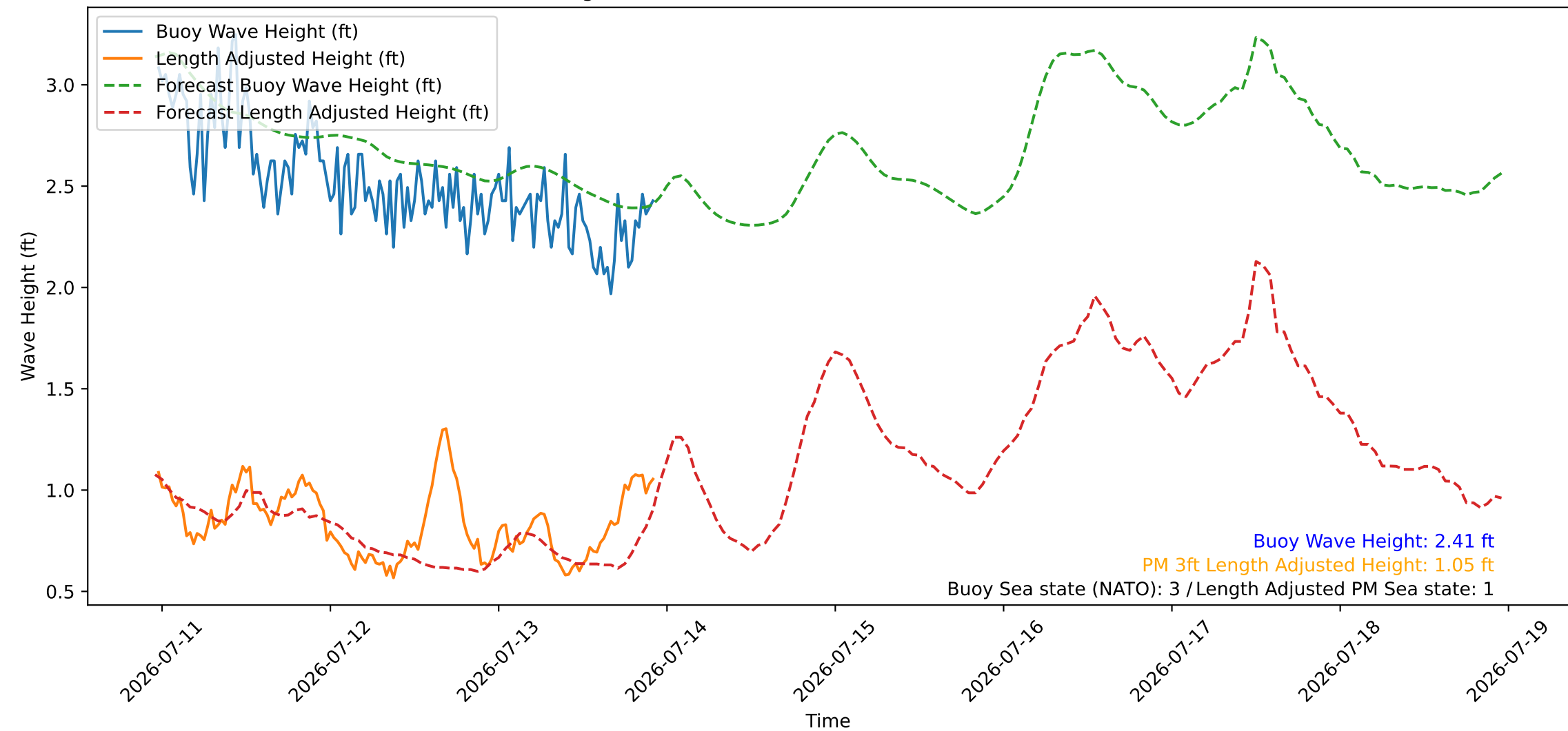
Wave Heights over Time for Red Beach at 2026-07-13 23:00:46
