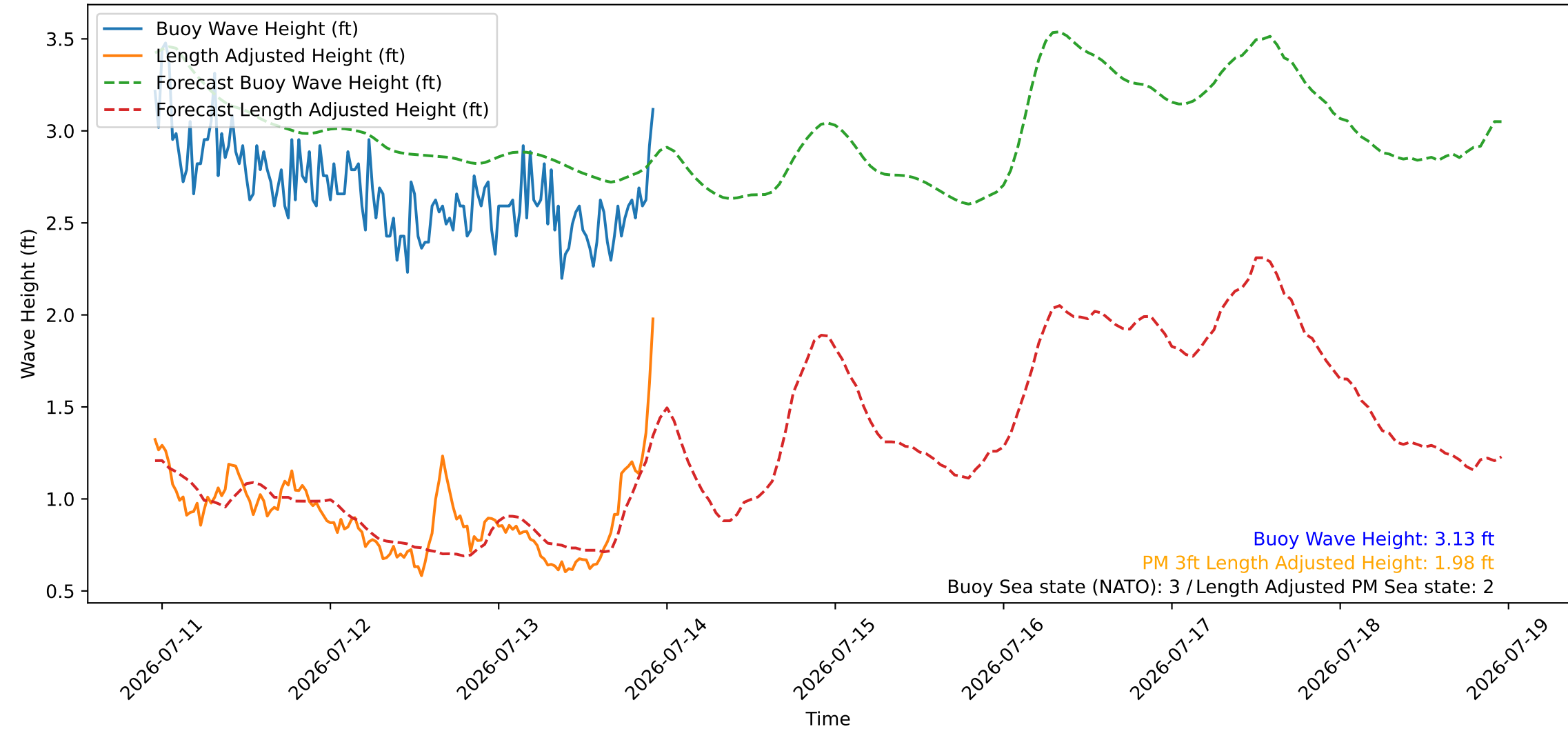
Wave Heights over Time for Green Beach at 2026-07-13 23:01:08
