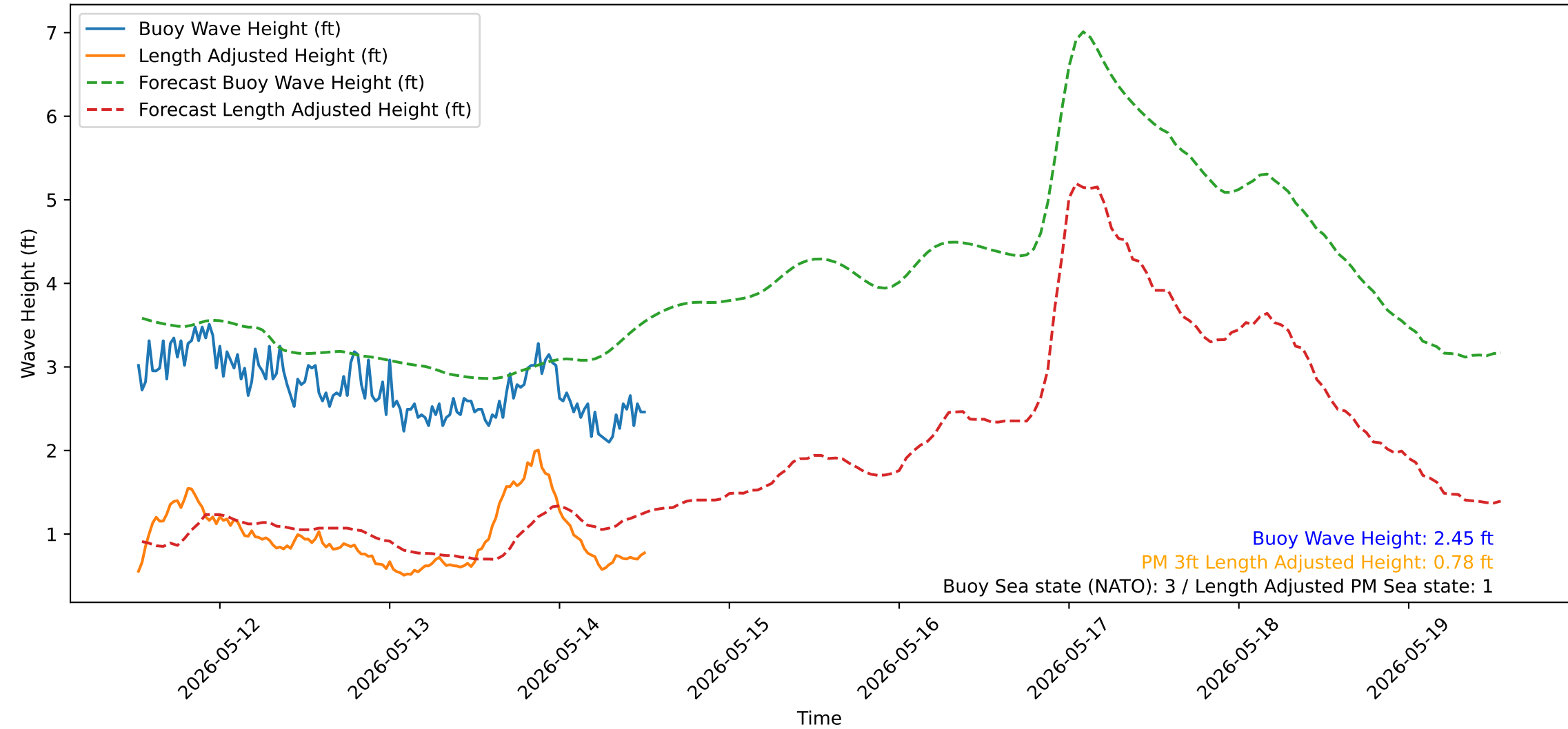
Wave Heights over Time for Green Beach at 2026-05-14 12:41:14
