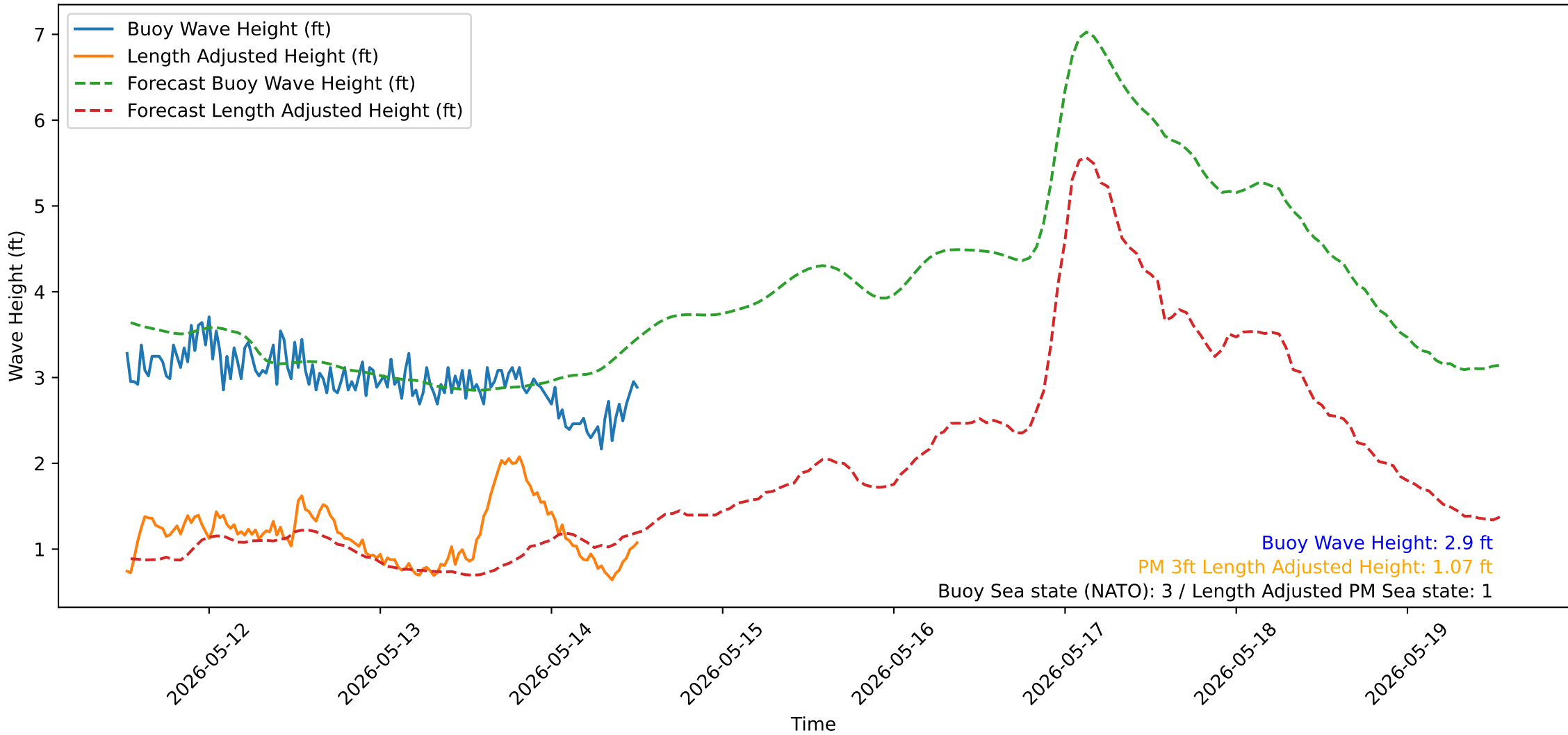
Wave Heights over Time for Oceanside Harbor at 2026-05-14 12:40:32
