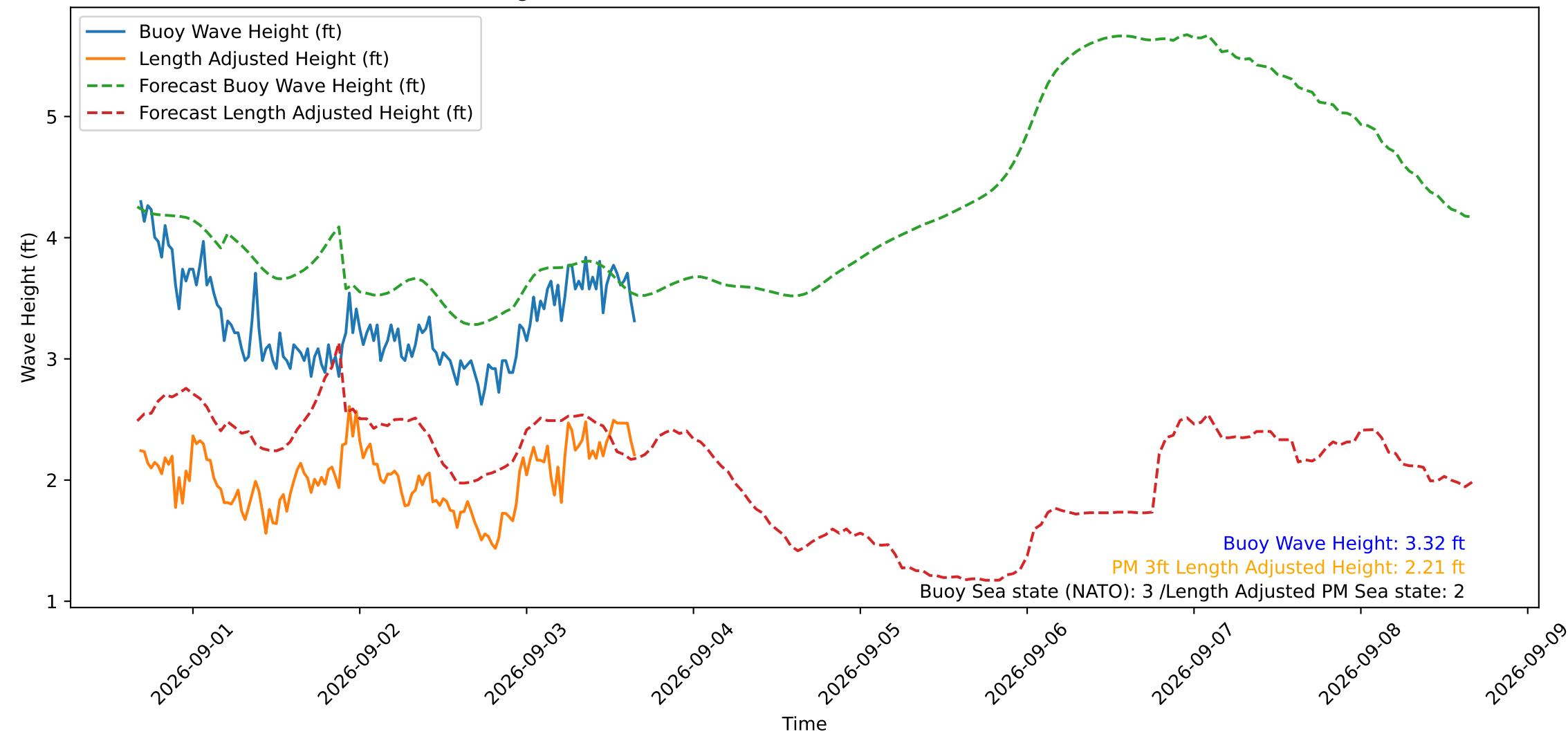
Wave Heights over Time for Oceanside Harbor at 2026-09-03 16:20:30
