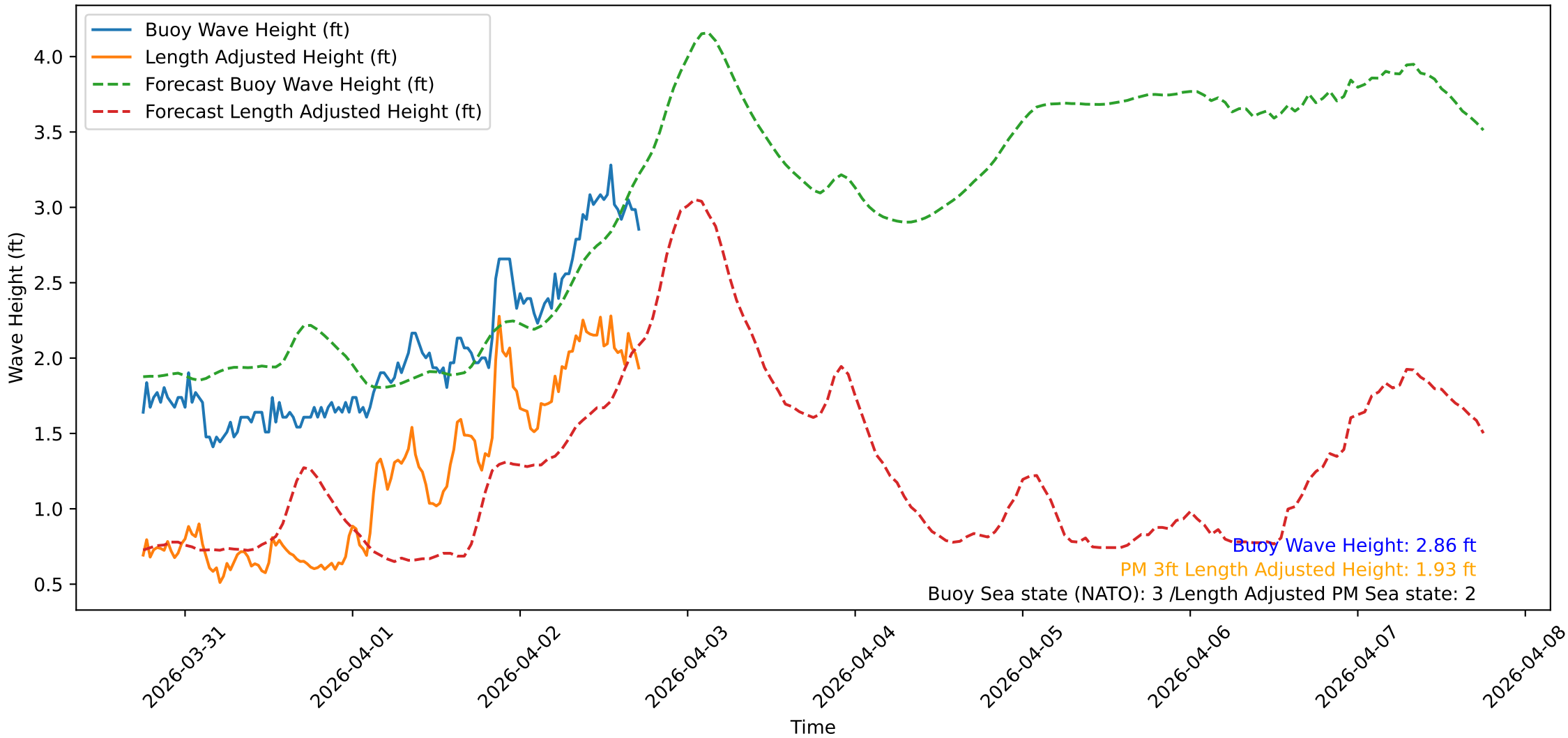
Wave Heights over Time for Green Beach at 2026-04-02 17:51:10
