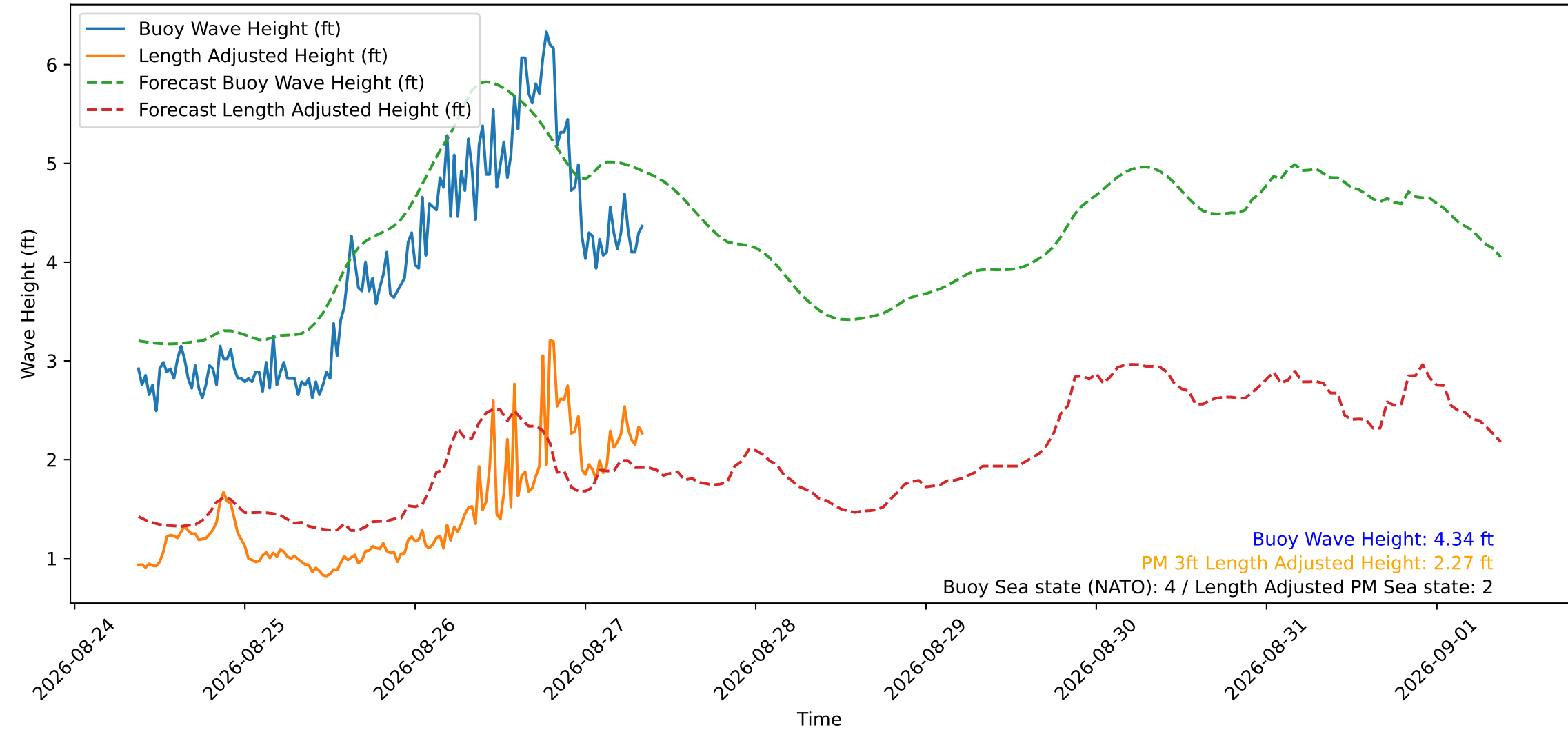
Wave Heights over Time for Green Beach at 2026-08-27 08:41:20
