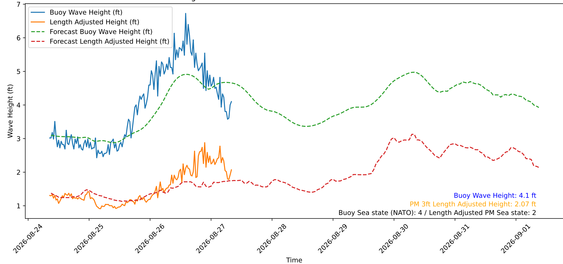
Wave Heights over Time for Oceanside Harbor at 2026-08-27 08:40:30
