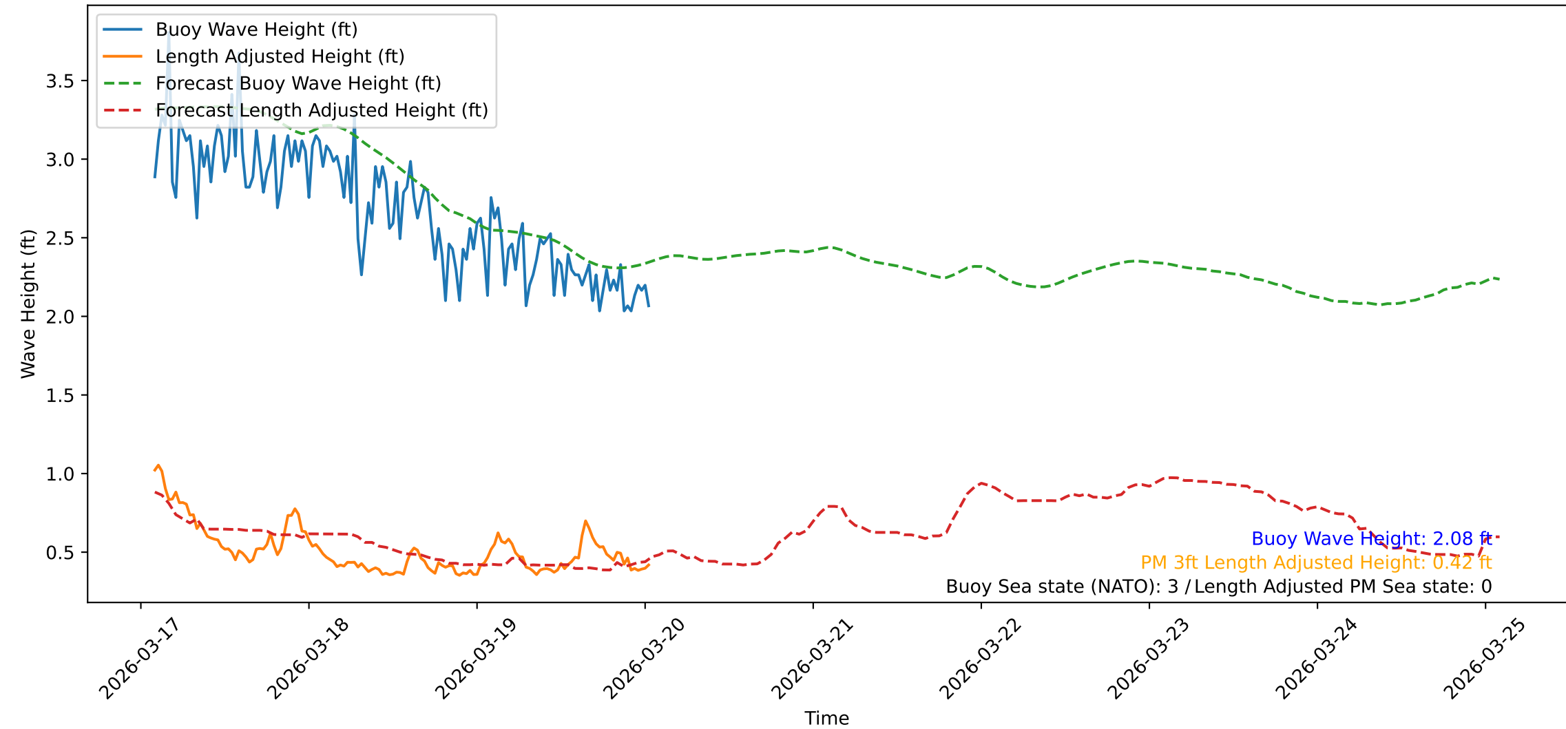
Wave Heights over Time for Red Beach at 2026-03-20 01:30:48
