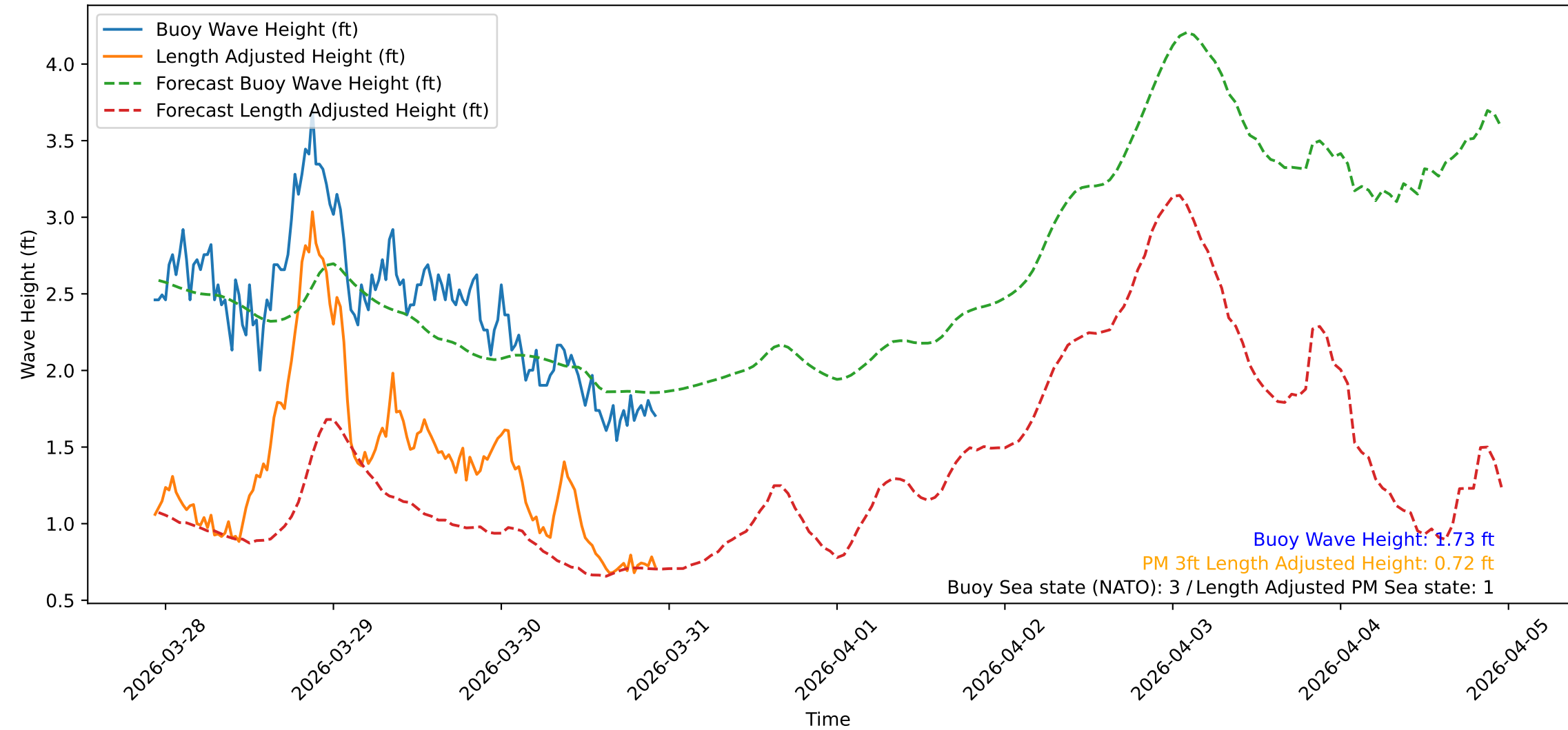
Wave Heights over Time for Green Beach at 2026-03-30 22:41:09
