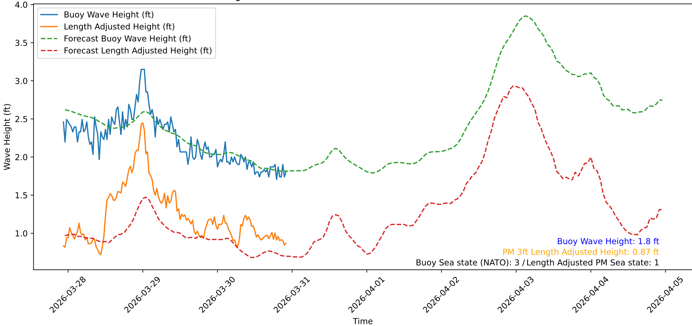
Wave Heights over Time for Oceanside Harbor at 2026-03-30 22:40:31
