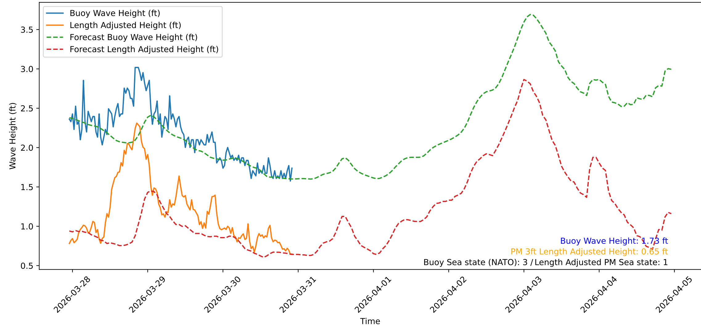
Wave Heights over Time for Red Beach at 2026-03-30 22:40:47
