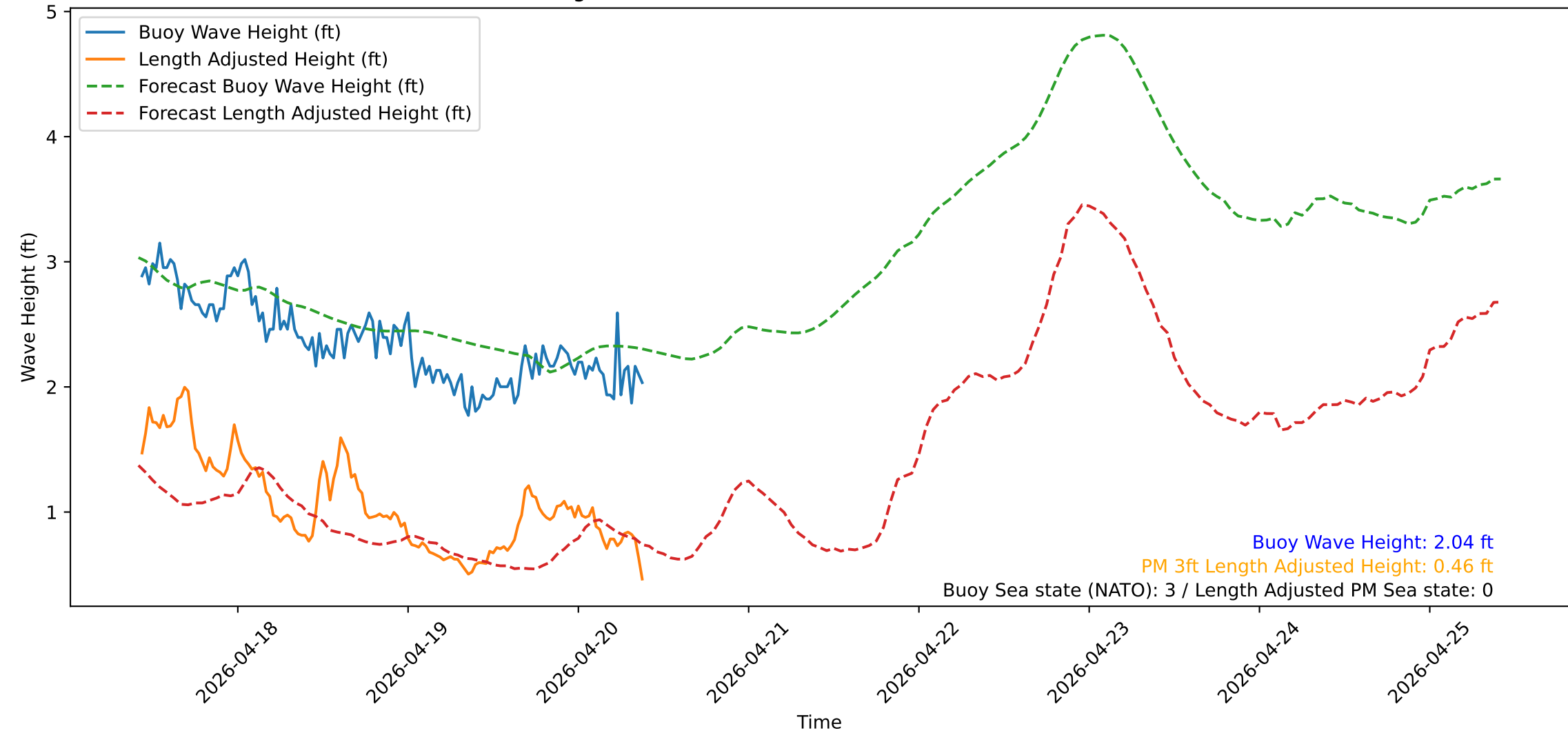
Wave Heights over Time for Red Beach at 2026-04-20 10:00:50
