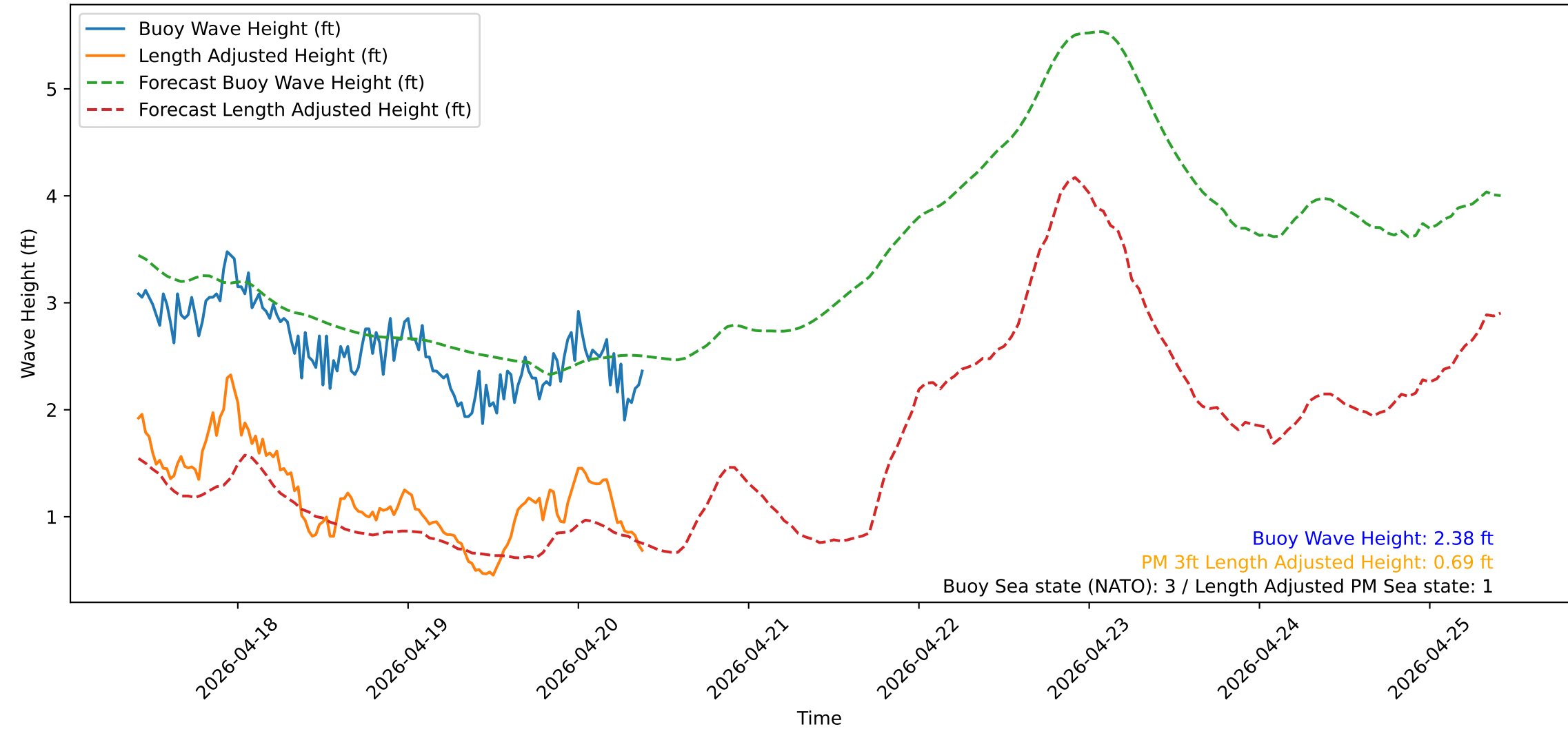
Wave Heights over Time for Green Beach at 2026-04-20 10:01:13
