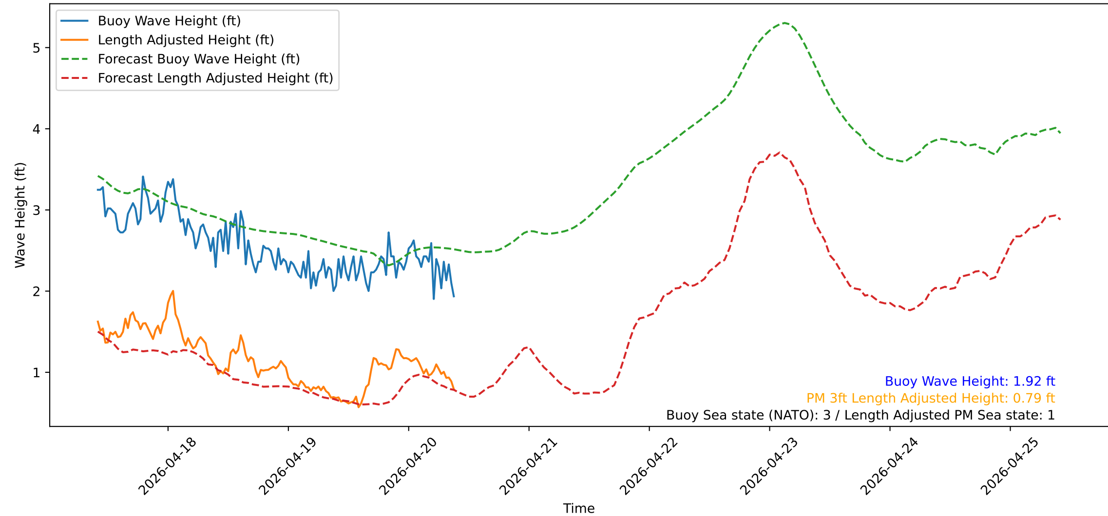
Wave Heights over Time for Oceanside Harbor at 2026-04-20 10:00:31
