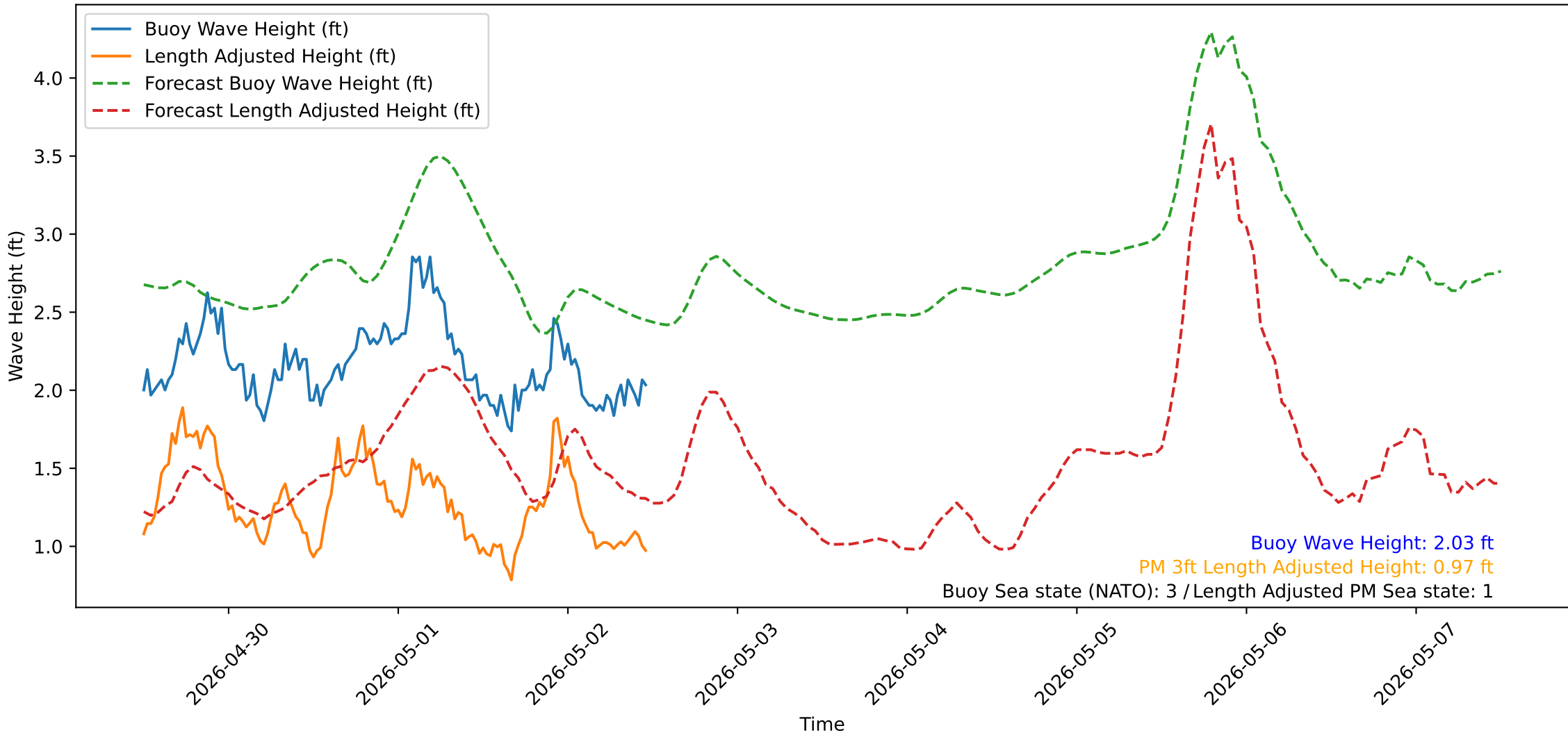
Wave Heights over Time for Green Beach at 2026-05-02 11:51:14
