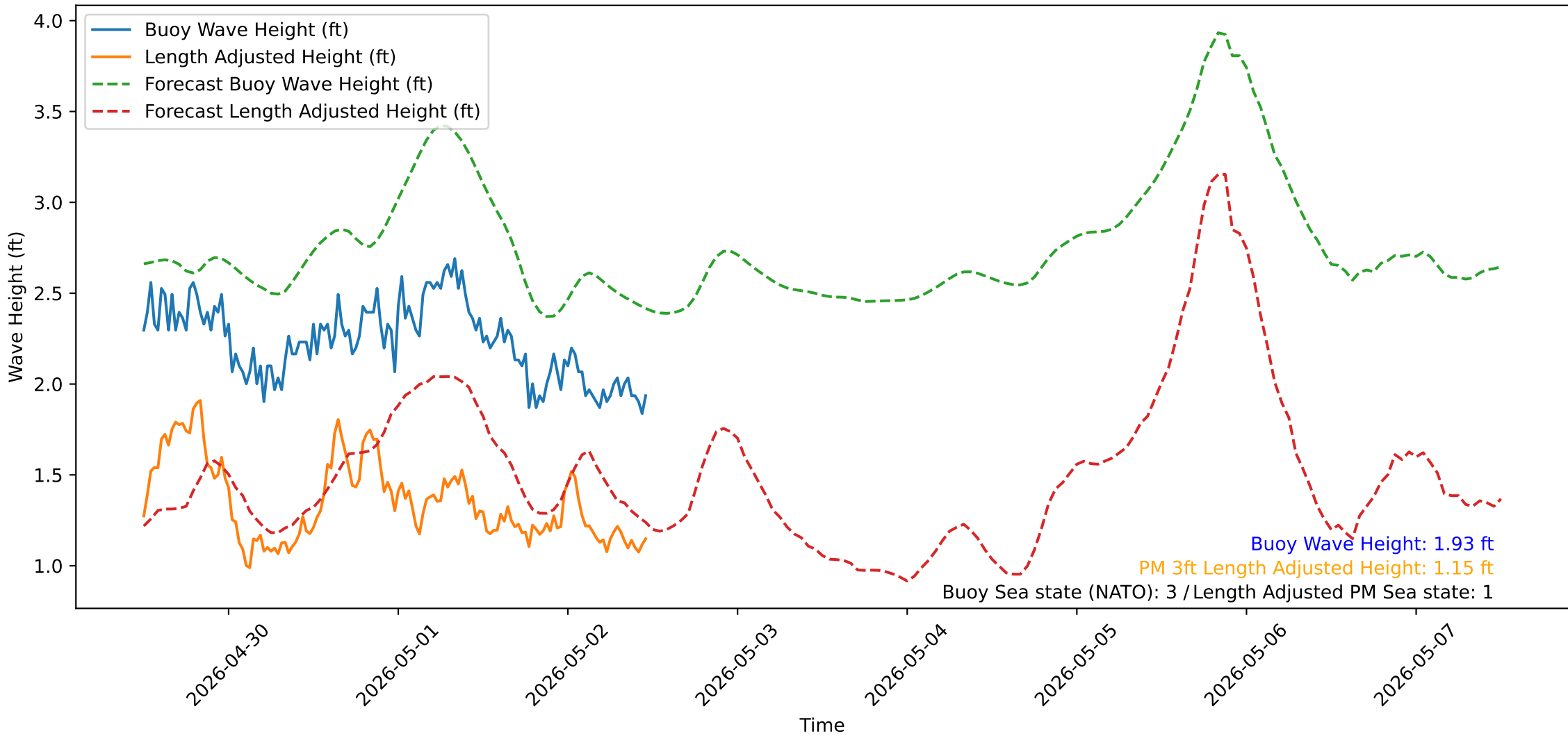
Wave Heights over Time for Oceanside Harbor at 2026-05-02 11:50:31
