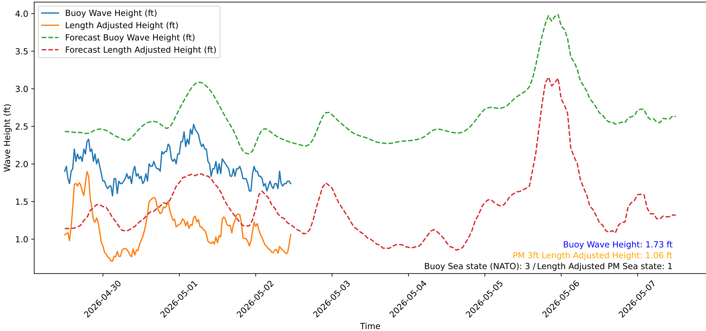
Wave Heights over Time for Red Beach at 2026-05-02 11:50:52
