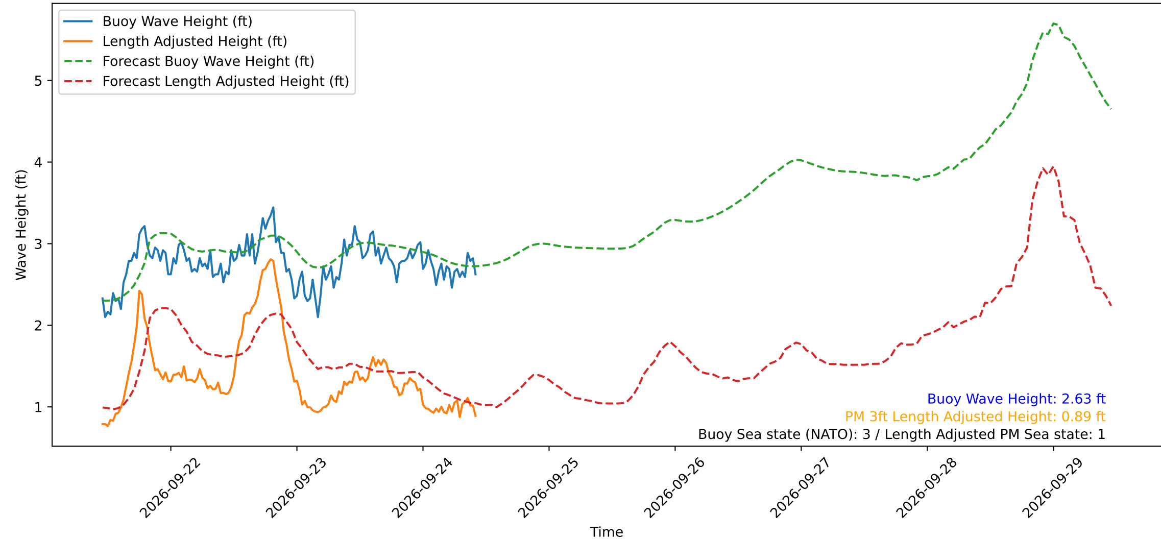
Wave Heights over Time for Green Beach at 2026-09-24 10:41:11
