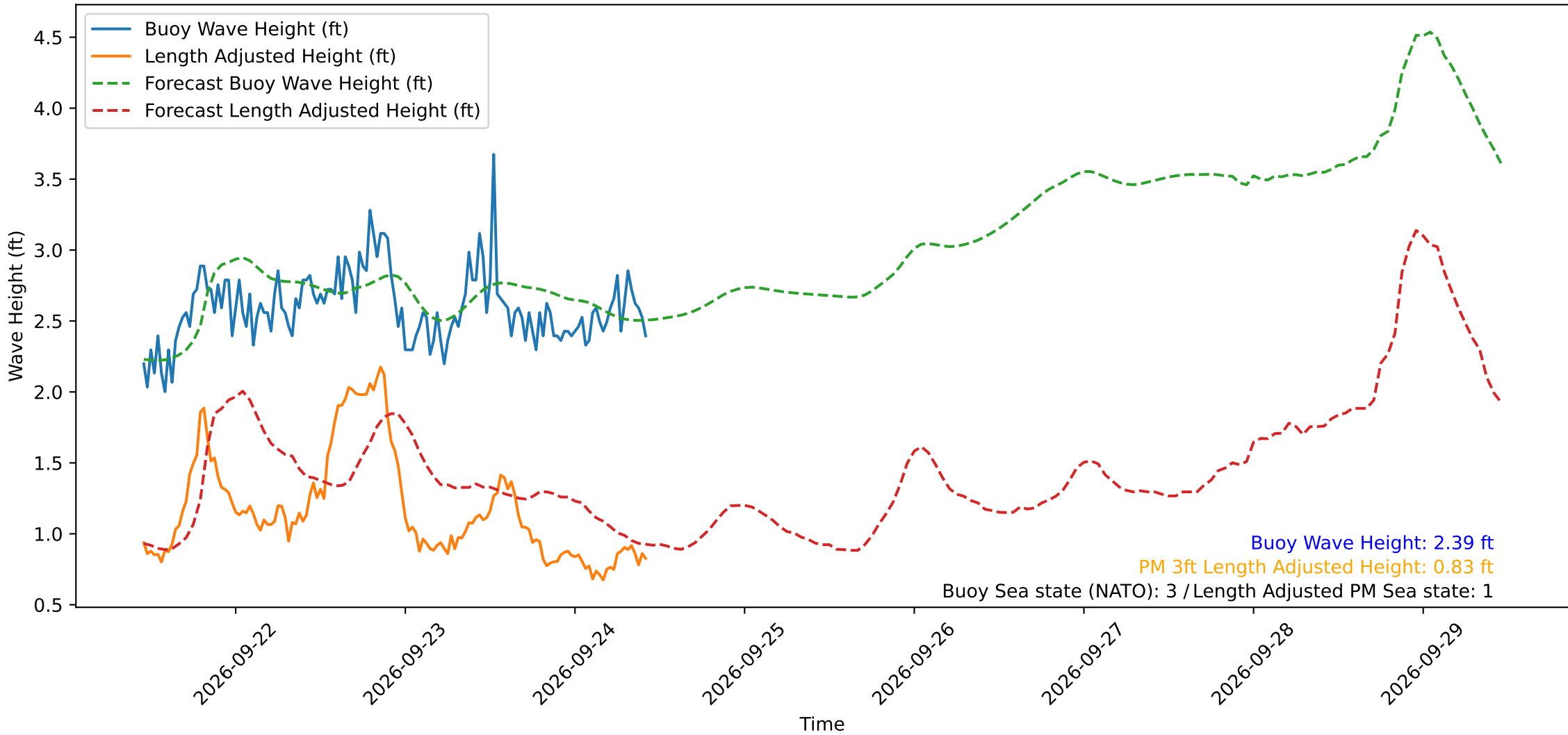
Wave Heights over Time for Red Beach at 2026-09-24 10:40:49
