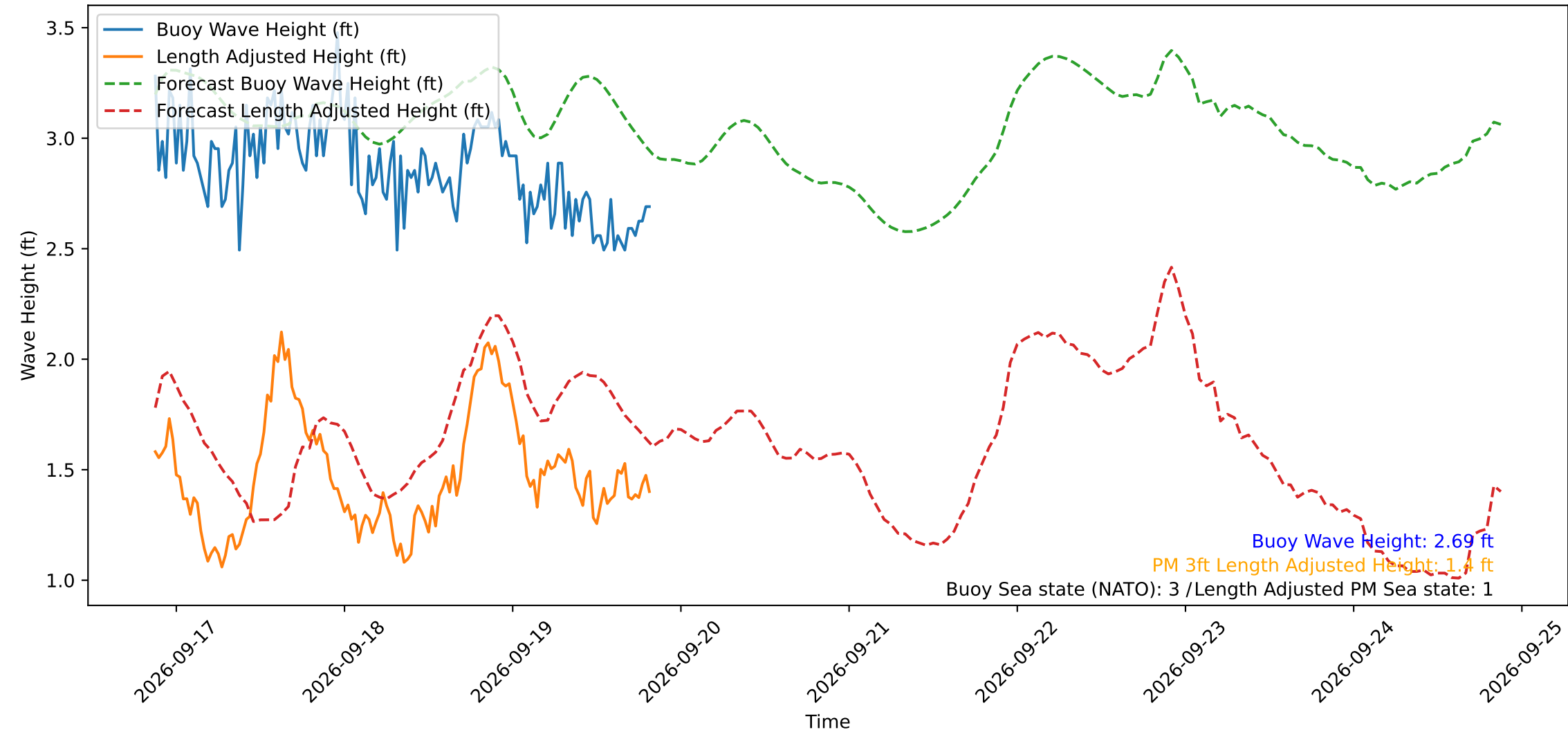
Wave Heights over Time for Green Beach at 2026-09-19 20:31:11
