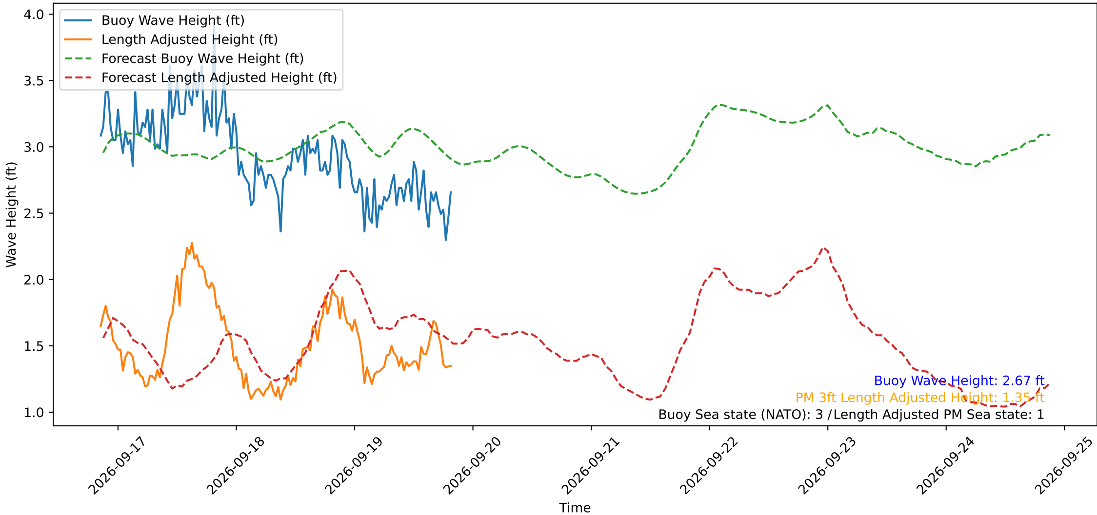
Wave Heights over Time for Oceanside Harbor at 2026-09-19 20:30:29
