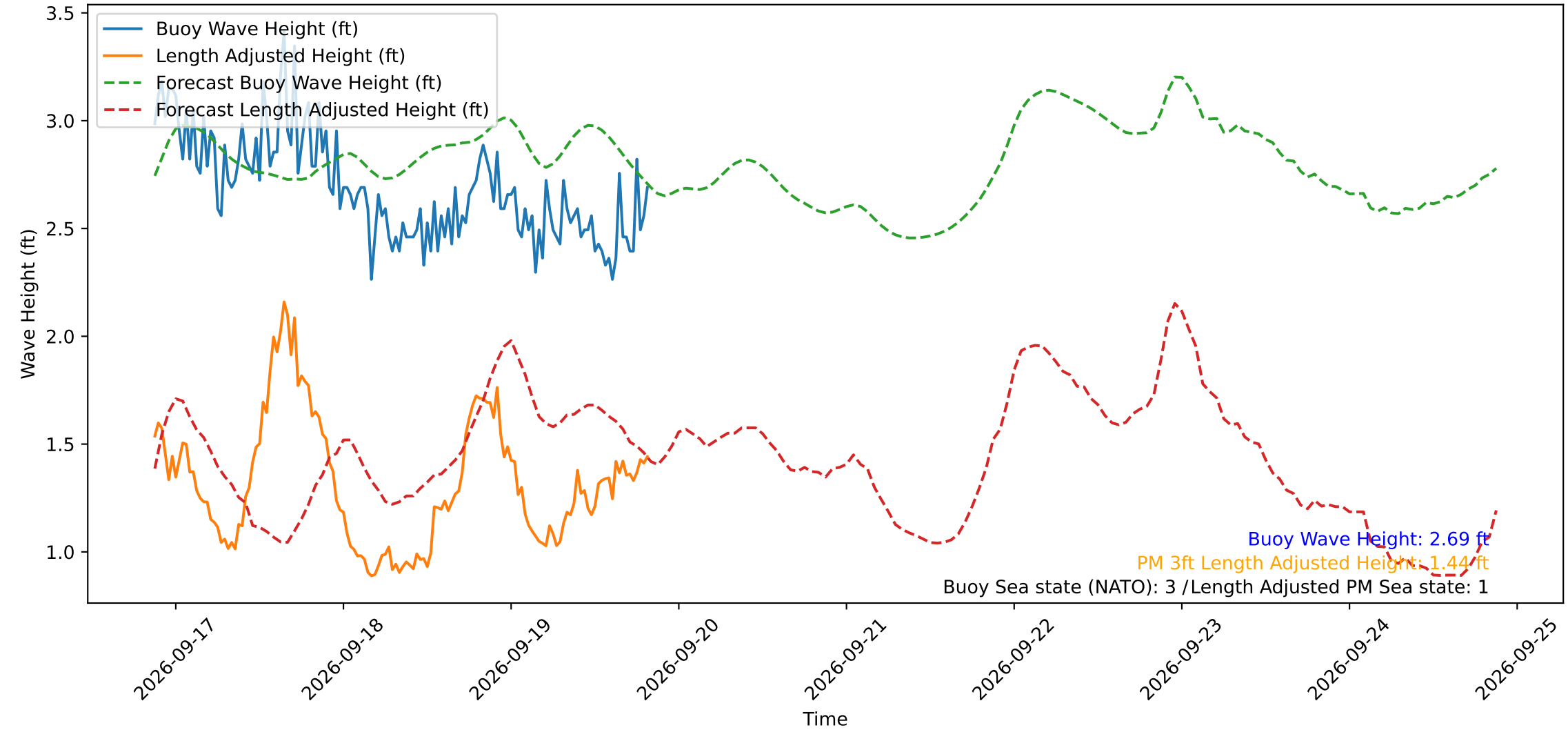
Wave Heights over Time for Red Beach at 2026-09-19 20:30:49
