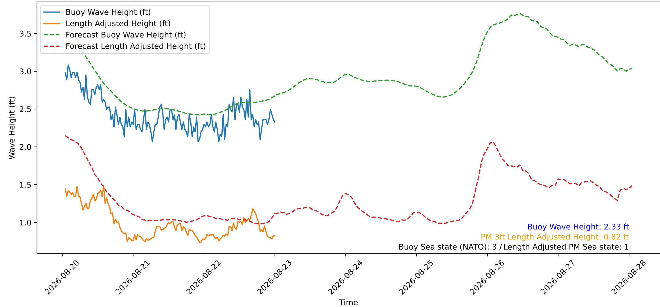
Wave Heights over Time for Red Beach at 2026-08-23 00:50:51
