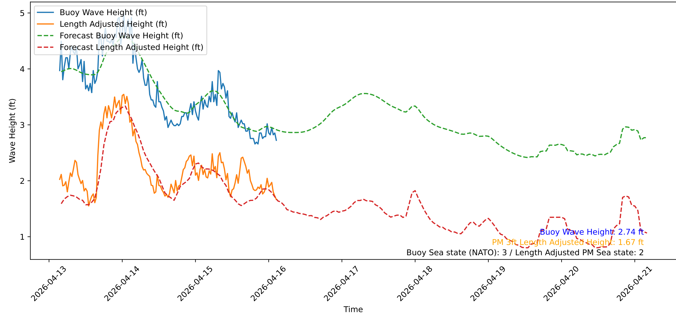
Wave Heights over Time for Green Beach at 2026-04-16 03:31:12
