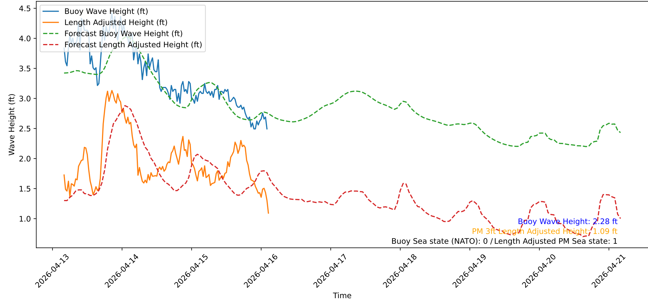
Wave Heights over Time for Red Beach at 2026-04-16 03:30:50
