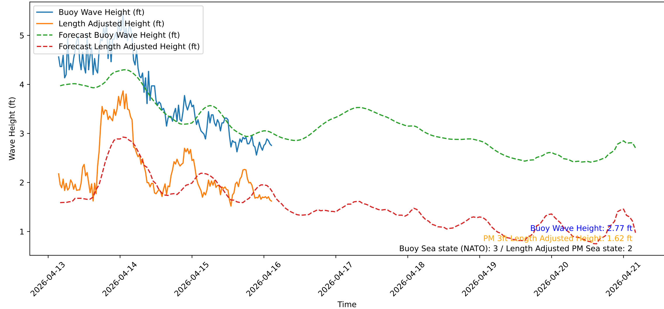
Wave Heights over Time for Oceanside Harbor at 2026-04-16 03:30:31
