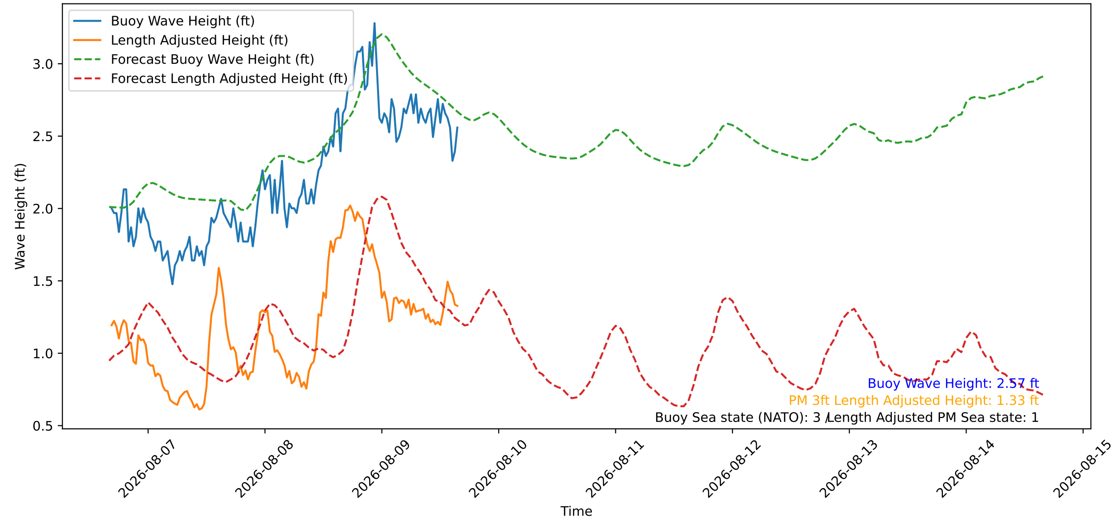
Wave Heights over Time for Red Beach at 2026-08-09 16:20:48
