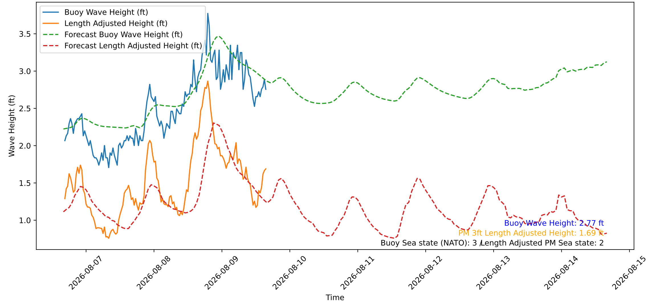
Wave Heights over Time for Green Beach at 2026-08-09 16:21:12
