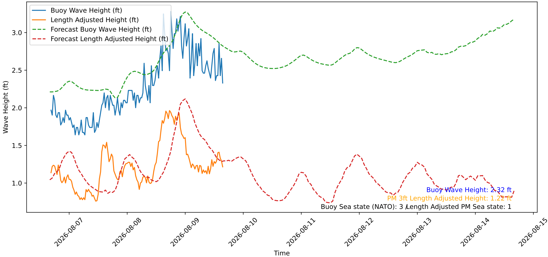
Wave Heights over Time for Oceanside Harbor at 2026-08-09 16:20:27
