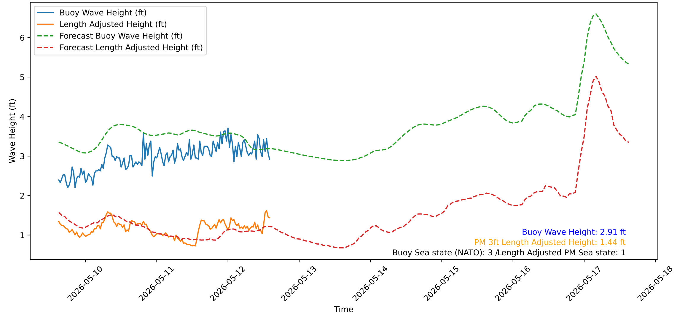
Wave Heights over Time for Oceanside Harbor at 2026-05-12 15:10:31
