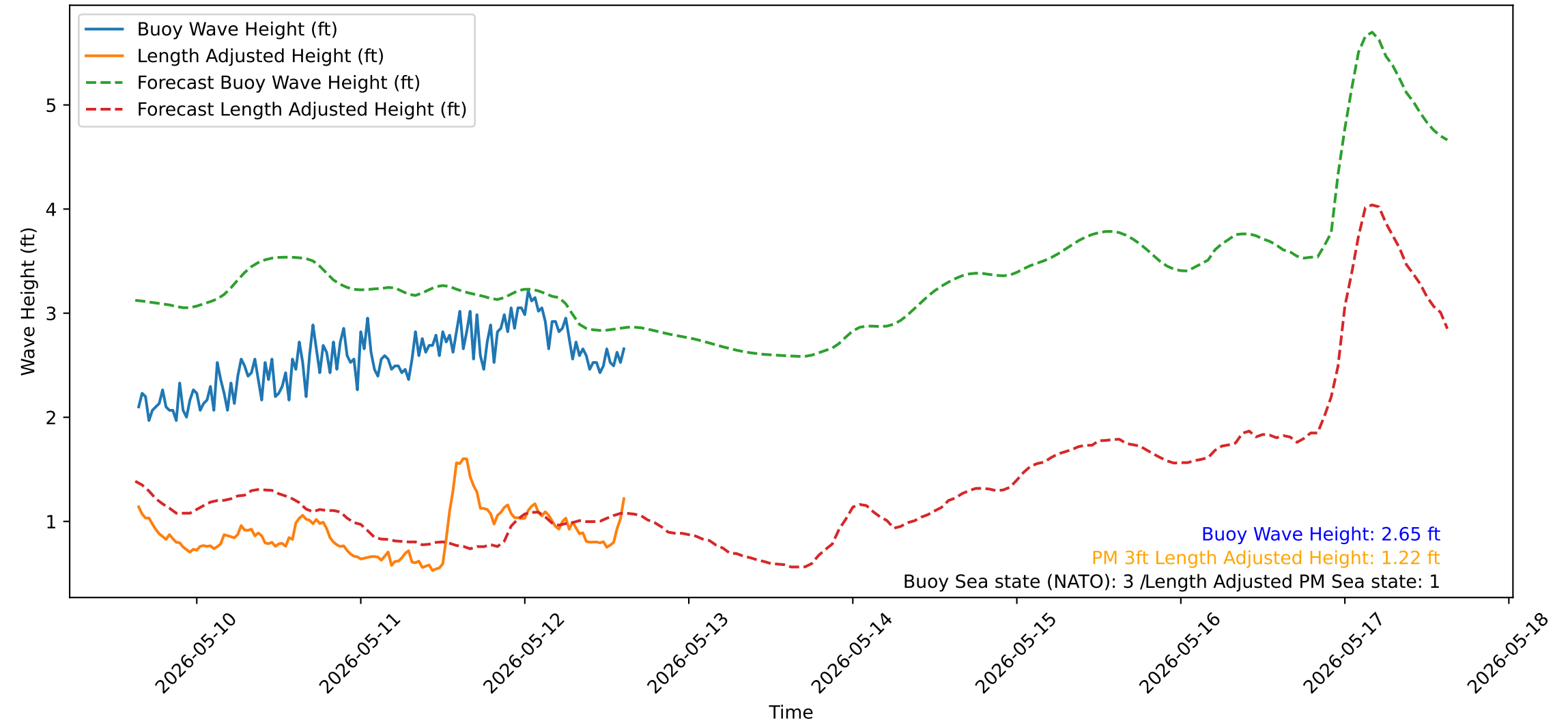
Wave Heights over Time for Red Beach at 2026-05-12 15:10:50
