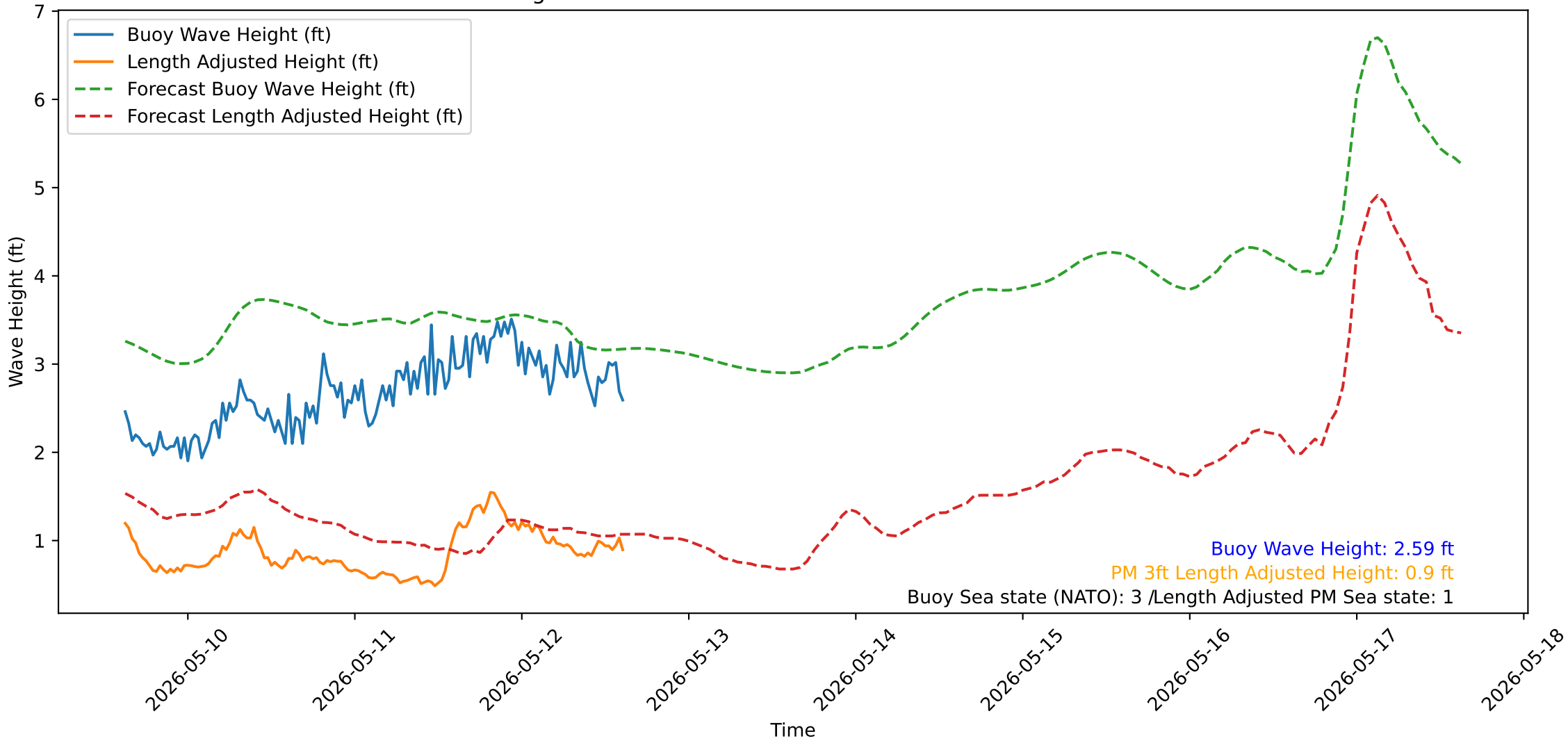
Wave Heights over Time for Green Beach at 2026-05-12 15:11:13
