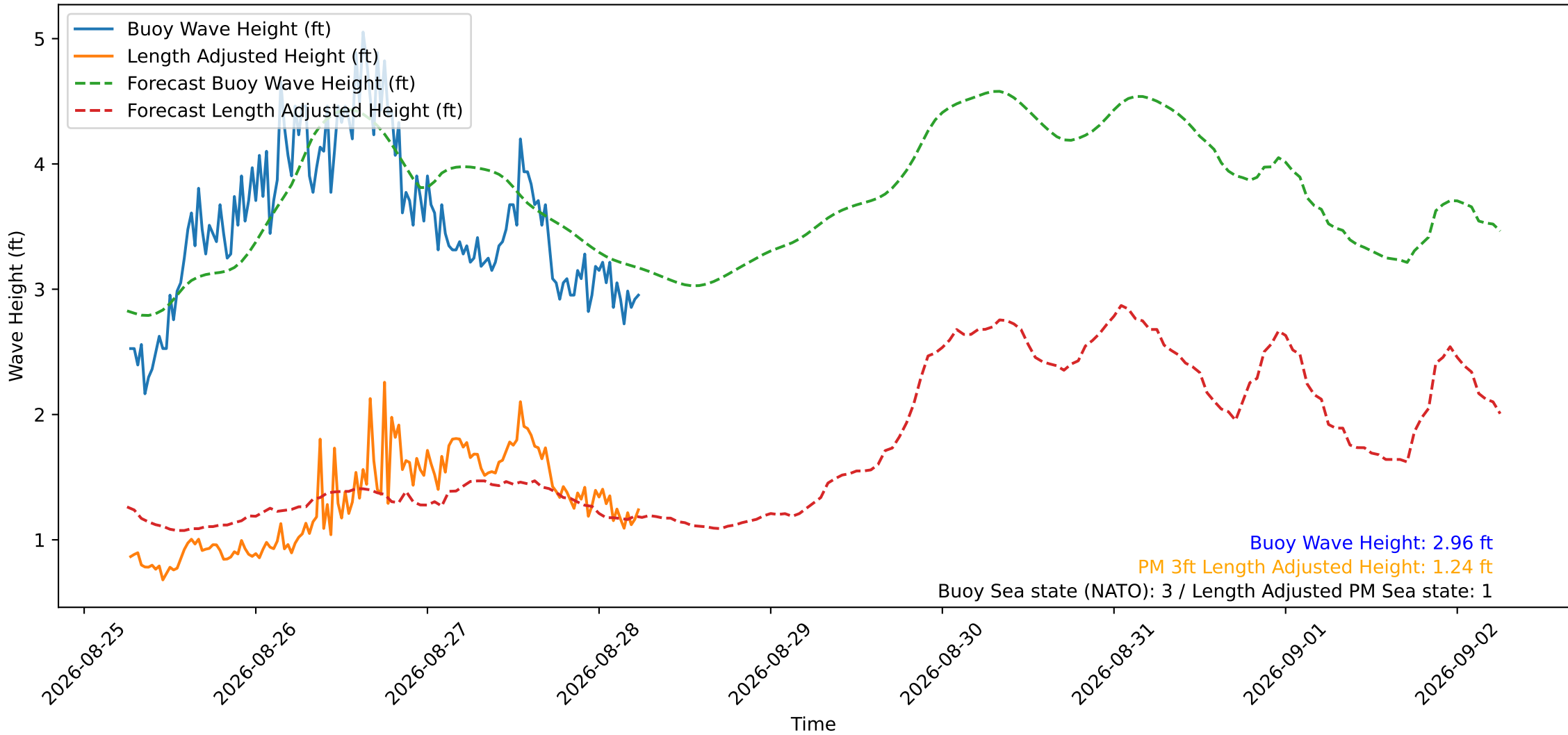
Wave Heights over Time for Red Beach at 2026-08-28 06:10:50
