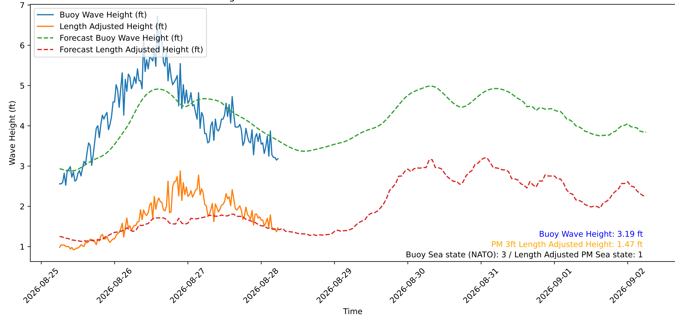
Wave Heights over Time for Oceanside Harbor at 2026-08-28 06:10:29
