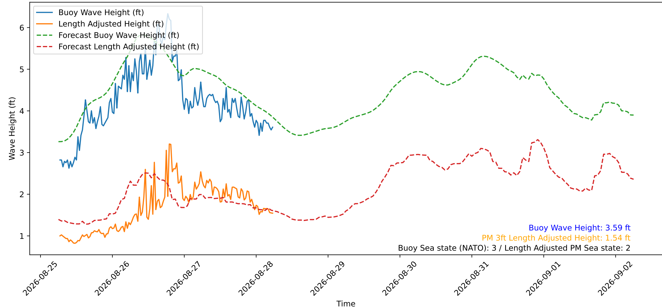
Wave Heights over Time for Green Beach at 2026-08-28 06:11:13
