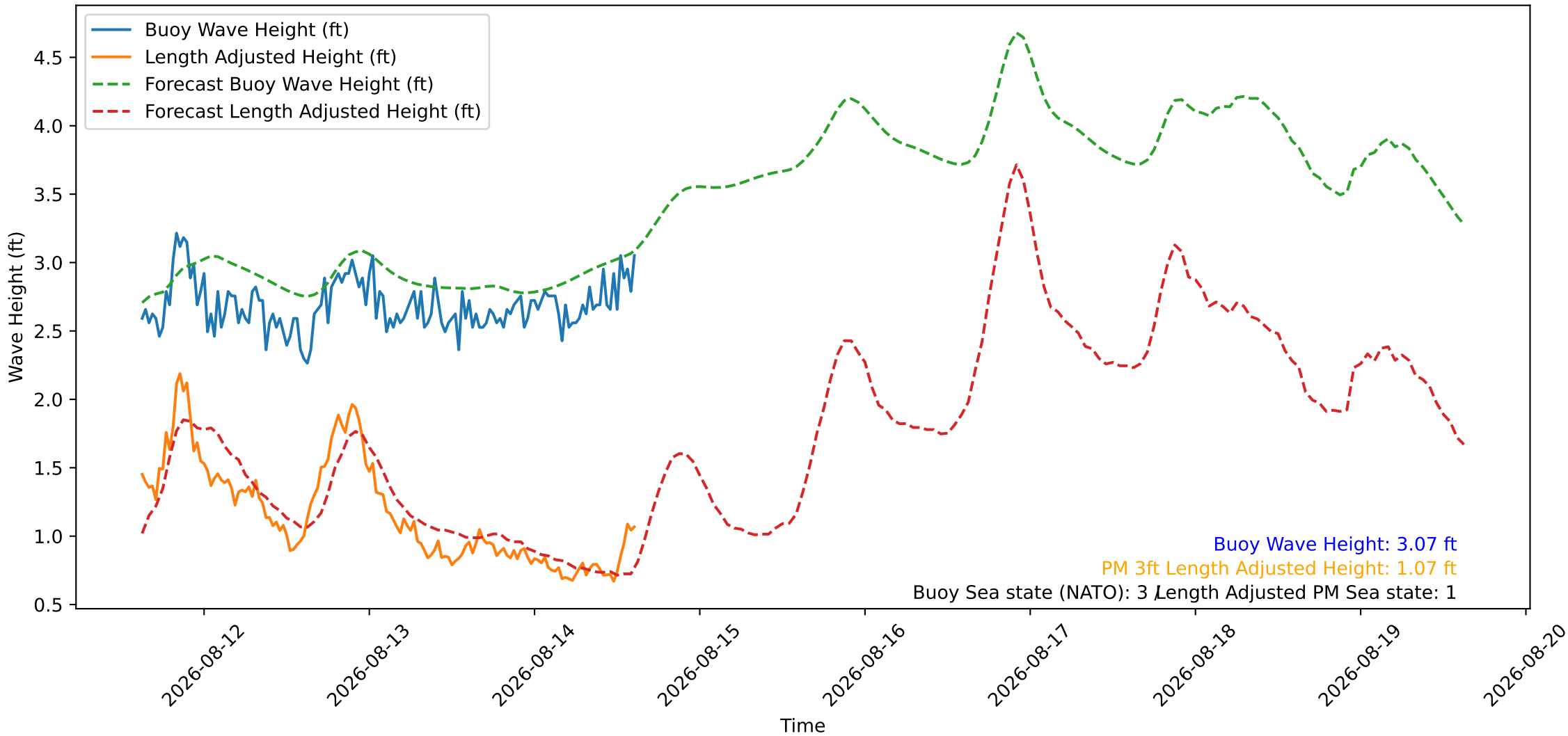
Wave Heights over Time for Green Beach at 2026-08-14 15:11:08
