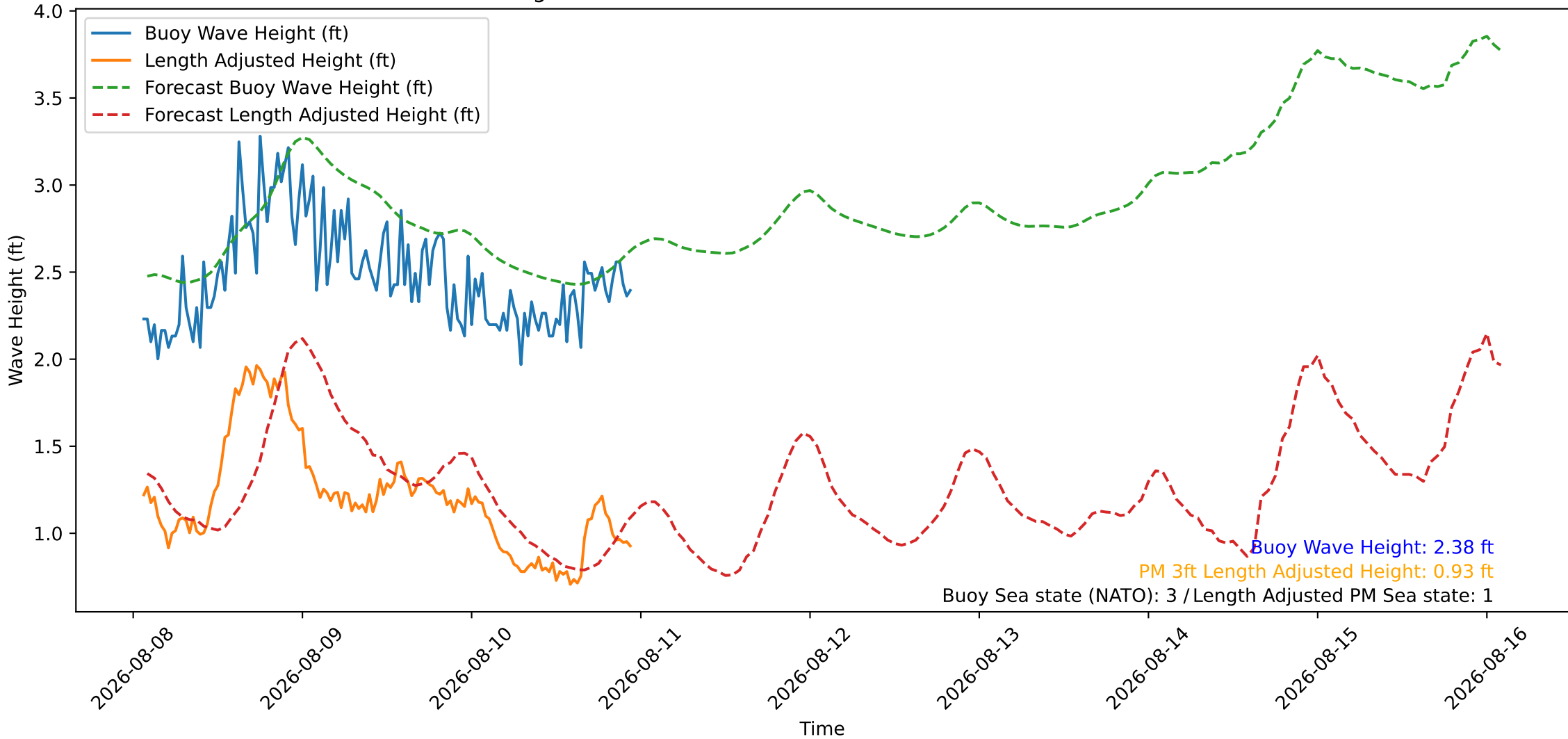
Wave Heights over Time for Oceanside Harbor at 2026-08-11 01:30:26
